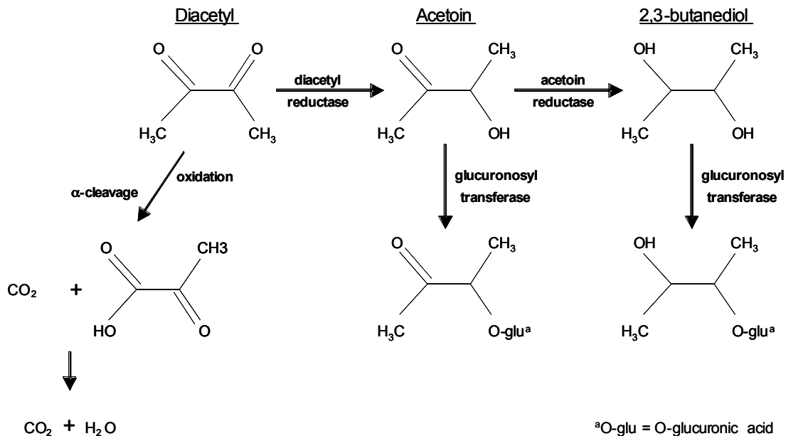
Figure 1. Diacetyl/acetoin metabolism
