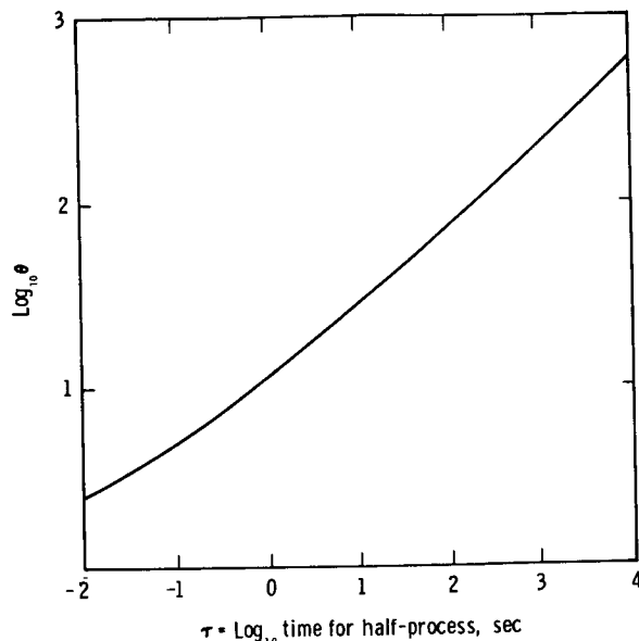
FIGURE 7.—Relation between \theta and \tau for diffusion of dissolved nitrogen from space between two coaxial cylinders of radii a and b , for b = 4 \times 10^{-4} cm, \theta = a/b , \tau = half process time. (AFTER ROUGHTON. 371 )
