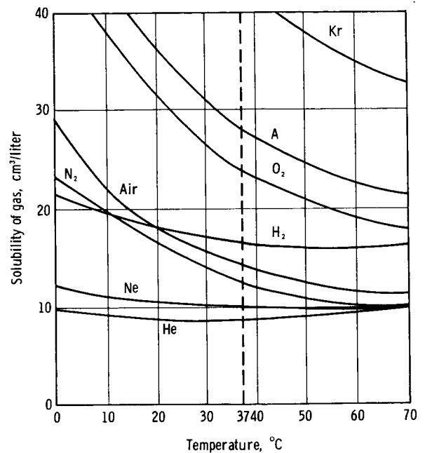
FIGURE 3.— Solubility of gases in water at different temperatures. (AFTER TIETZE. 422 )
