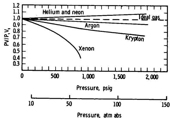
FIGURE 2.—Compressibility of the inert gases at 21^\circ\text{C} ( P = \text{pressure} ; V = \text{volume} ). (AFTER JENKINS AND COOK. 245 )
