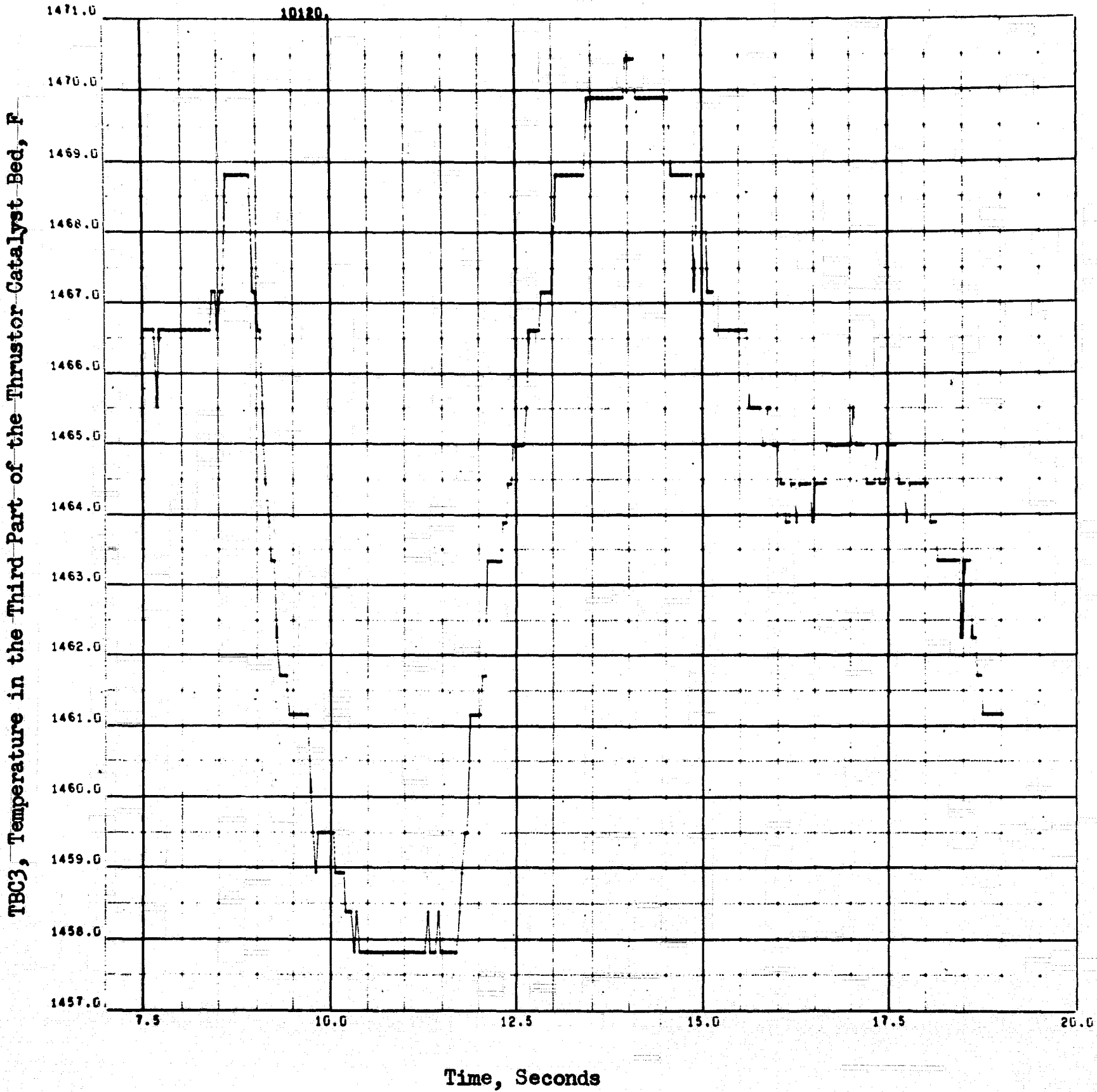
Figure 130. Temperature in the Third Part of the Catalyst Bed, (Thruster Part of the Thruster, Conditioner System)
