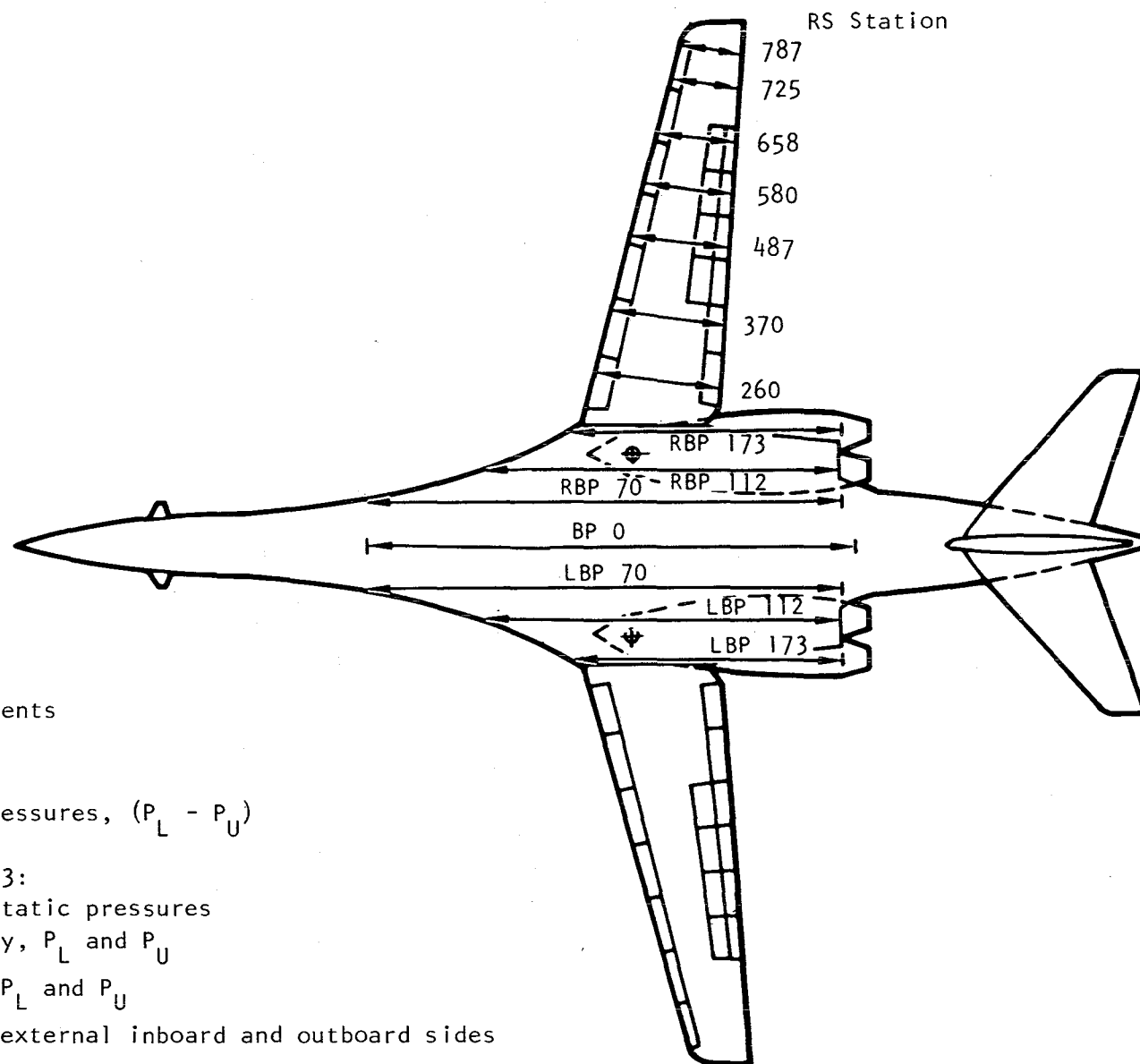
Figure 9.- Location of pressure measurements.
