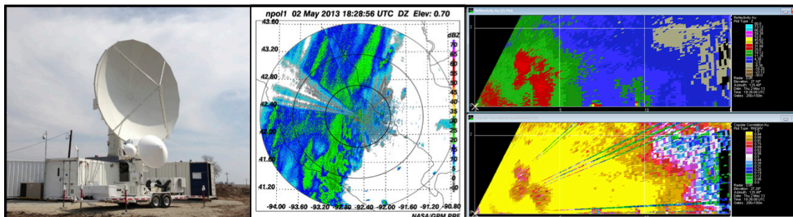
Figure 2.6: The NPOL and D3R radars are shown as deployed in Traer, Iowa.
