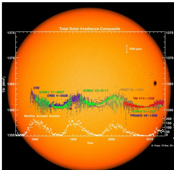
Figure 3.3: Solar Irradiance Composite
