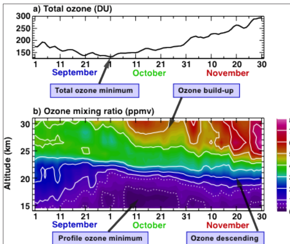
Figure 2.5: Daily time series of satellite ozone measurements near the center of the Antarctic ozone hole during the Southern Hemisphere spring of 2012 (September–November). Panel (a) is the time series of total ozone values (DU) observed by OMPS Total Column Mapper showing ozone depletion in September and its gradual recovery in October and November. Panel (b) shows the evolution of the ozone vertical distribution (ppmv) measured by the OMPS Limb Profiler in the middle and lower stratosphere. In October, while the ozone concentration in the lower stratosphere continues to decline, a strong ozone build-up occurs in the middle stratosphere. Sharp vertical gradients caused by the ozone loss are observed between 20 km and 25 km.
