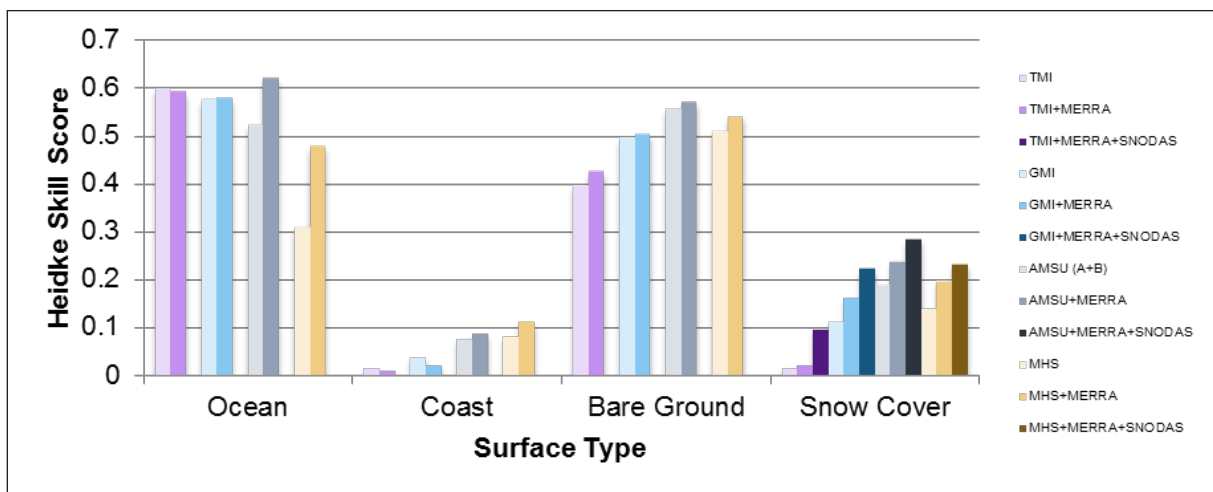
Figure 2.2: Relative precipitation detection skill over various surfaces and impact of ancillary data regarding atmospheric temperature and water vapor profiles (from MERRA reanalysis) and snow cover (from SNODAS) is shown for four passive microwave sensors: TMI, GMI, AMSU, and MHS.
