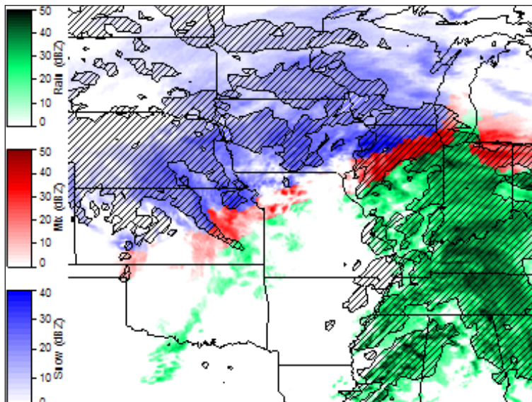
Figure 2.1: Ground mosaic surface reflectivity from a winter storm on December 8, 2009, is overlaid with precipitation detection (hatched area) from an SSMIS overpass. The contour overlay represents the precipitation detection threshold corresponding to a precipitation rate of 0.25 mm/hr. Some regions of snowfall over the upper Midwest are missed at this threshold, while some false detection (associated with snow covered ground) is evident over western Nebraska and North Dakota. Changing the threshold can result in detection of lighter precipitation rates, but at the expense of more false detections.
