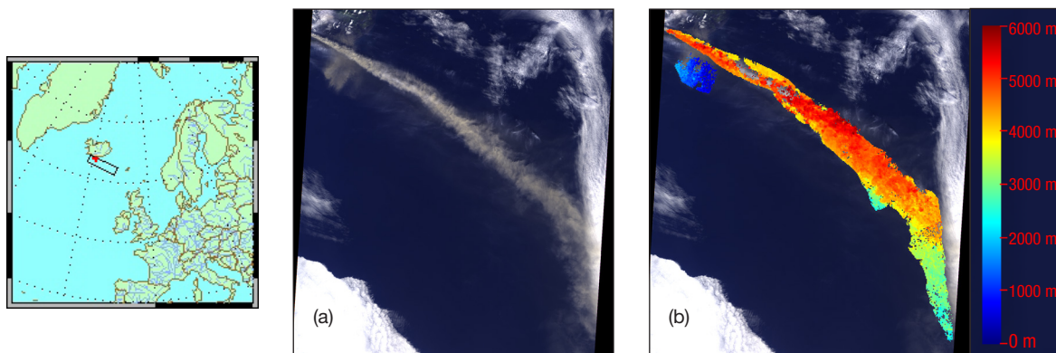
Figure 2.3: Map of the plume's location. (a) MISR true-color image of the Iceland volcanic plume on May 7, 2010, with map inset. (b) Plume height, in meters, derived from MISR multi-angle stereo imagery using the "MINX" algorithm. Note the near-surface (blue) plume of re-mobilized ash blown toward the southwest.
