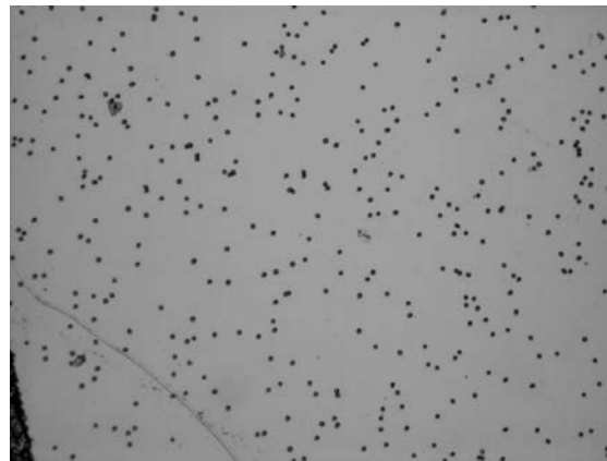
Figure XIII.11. a) Indoor radon monitor having a polycarbonate film detector b) Tracks due alpha particles from radon in polycarbonate film, magnification 40, the photographed area is about 1.3 by 1.0 mm ( http://pages.csam.montclair.edu/~kowalski/cf/327squeeze.html ).
