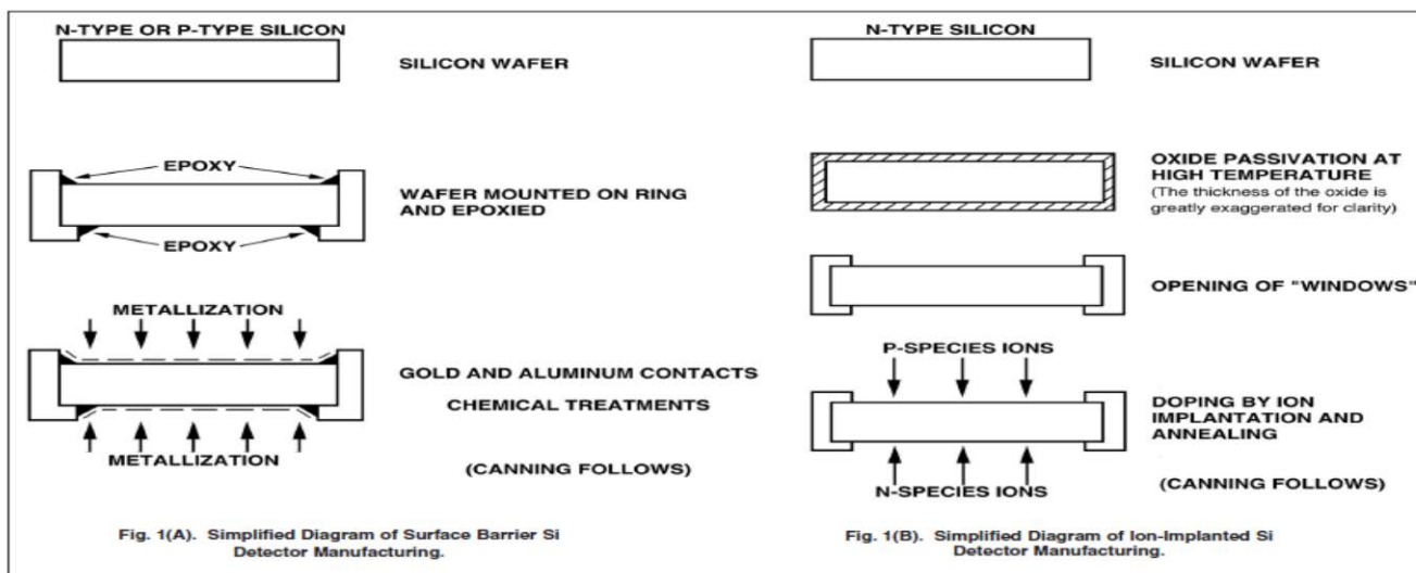
Figure XI.1. Production of silicon detectors for alpha spectroscopy. Left: surface barrier detectors. Right: Passivated ion-implanted detector. ( http://www.ortec-online.com/Products-Solutions/RadiationDetectors/silicon-charged-particle-detectors.aspx ).
