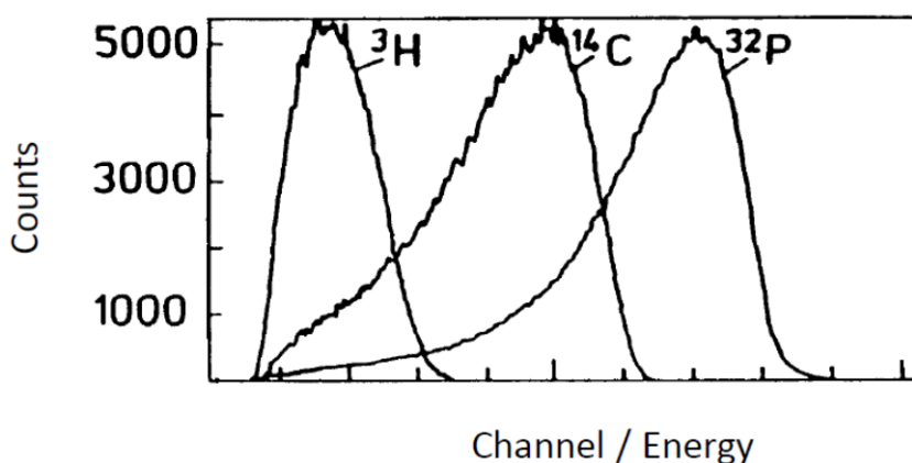
Figure XII.8. The individually determined liquid scintillation spectra of ^3\text{H} ( E_{\text{max}} 18 keV), ^{14}\text{C} ( E_{\text{max}} 180 keV) and ^{32}\text{P} ( E_{\text{max}} 1700 keV).
