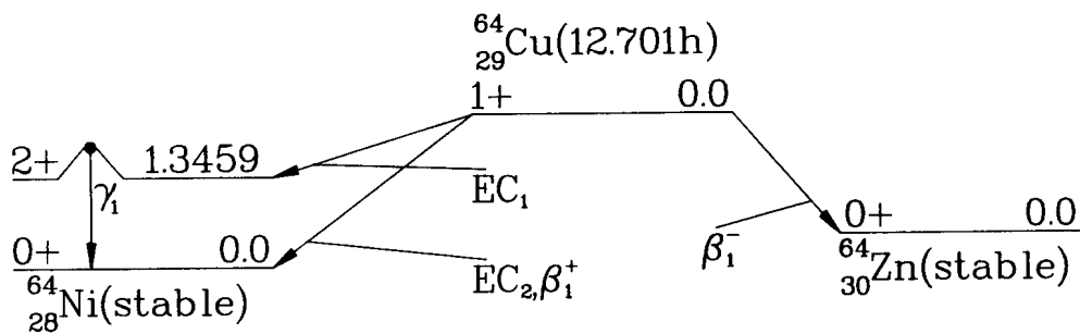
Figure V.17. Decay scheme of ^{64}\text{Cu} (Radionuclide Transformations, Annals of the ICRP, ICRP Publication 38, Pergamon Press, 1983).
