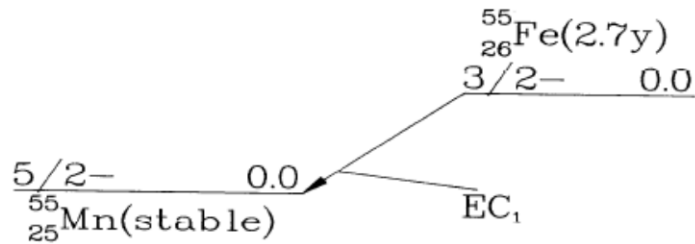
Figure V.14. Decay scheme of ^{55}\text{Fe} (Radionuclide Transformations, Annals of the ICRP, ICRP Publication 38, Pergamon Press, 1983).
