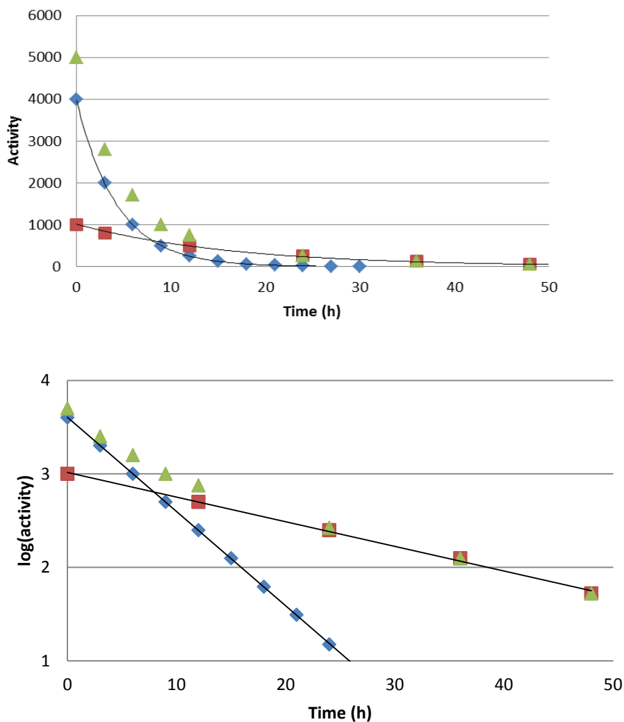
Figure VI.2. Individual and total activities of two coexisting radionuclides as a function of time. Top: activity in linear scale. Bottom: activity in logarithmic scale. Diamond (◆): Radionuclide with a half-life of 3 hours. Square (■): radionuclide with a half-life of 12 hours. Triangle (▲): total activity.
