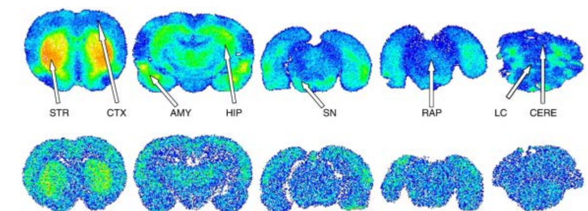
Figure XIII.10. Autoradiograms of representative ex vivo rat brain sections at 15 min after injection of dopamine transporter (DAT) radioligand [ ^{18}\text{F} ] \beta -CFT-FP. The upper row depicts a control rat, and the lower row depicts a rat pretreated with the DAT inhibitor GBR12909 (Koivula, T. et al. Nucl. Med. Biol. 35 (2):177-183).
