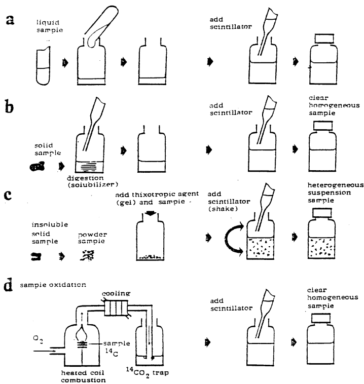
Figure XII.14. Sample preparation methods for liquid scintillation counting.
