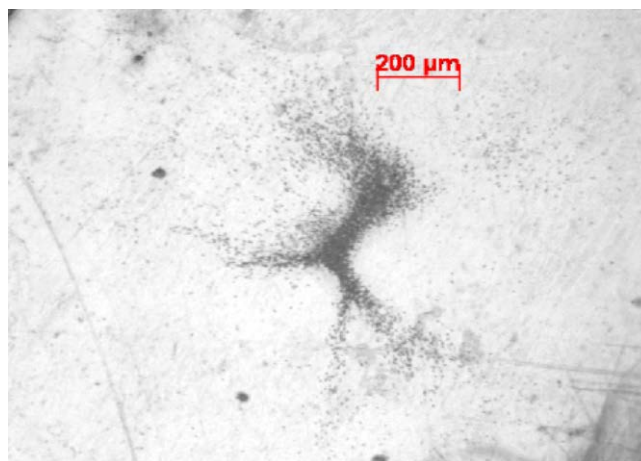
Figure XIII.12. An SSNTD image of an alpha-emitting particle in sediment (J. Jernström, M. Eriksson, J. Osán, G. Tamborini, S. Török, R. Simon, G. Falkenberg, A. Alsecz and M. Betti, Non-destructive characterisation of low radioactive particles from Irish Sea sediment by micro X-ray synchrotron radiation techniques: micro X-ray fluorescence ( \mu -XRF) and micro X-ray absorption near edge structure ( \mu -XANES) spectroscopy, J. Anal. At. Spectrom. 2004, 19, 1428-1433).
