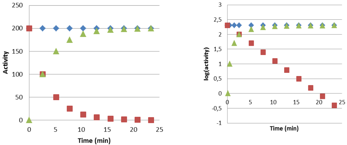
Figure VI.4. Development of a secular radioactive equilibrium in which the half-life of the parent nuclide very long and the half-life on the daughter nuclide ( ^{137\text{m}}\text{Ba} , t_{1/2} = 2.6 min) is considerably shorter than that of the parent ( ^{137}\text{Cs} , t_{1/2} = 30 a). Left: activity on linear scale. Right: activity on logarithmic scale. Diamond ( \blacklozenge ): ^{137}\text{Cs} . Square ( \blacksquare ): ^{137\text{m}}\text{Ba} if separated from ^{137}\text{Cs} . Triangle ( \blacktriangle ): ingrowth of ^{137\text{m}}\text{Ba} with ^{137}\text{Cs} after separation of ^{137\text{m}}\text{Ba} from ^{137}\text{Cs} .
