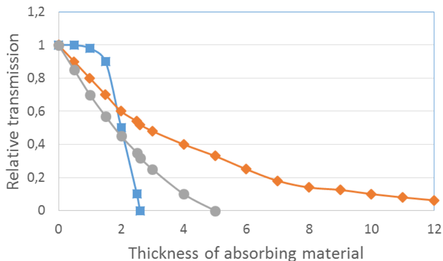
Figure VII.2. Absorption curves of alpha (square), beta (ball) and gamma radiation (diamond).
