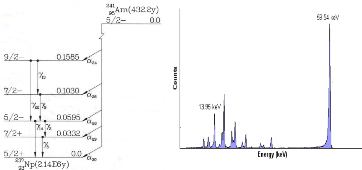
Figure V.20. Decay scheme (Radionuclide Transformations, Annals of the ICRP, ICRP Publication 38, Pergamon Press, 1983) and gamma spectrum ^{241}\text{Am} ( http://www.amptek.com/products/x-123-cdte-complete-x-ray-gamma-ray-spectrometer-with-cdte-detector/ ).
