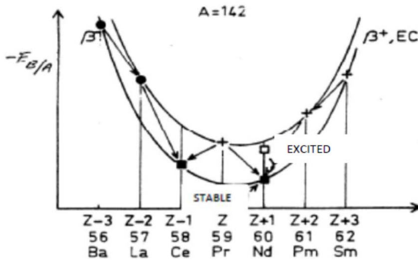
Figure V.16. Beta decay at the isobaric cross-section A=142 . Two stable nuclides, both even-even nuclides.
