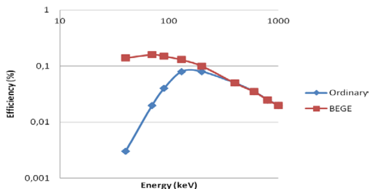
Figure IX.4. Efficiencies of an aluminum-covered ordinary and broad energy (BEGE) germanium detectors with same relative efficiency as a function of gamma ray energy.
