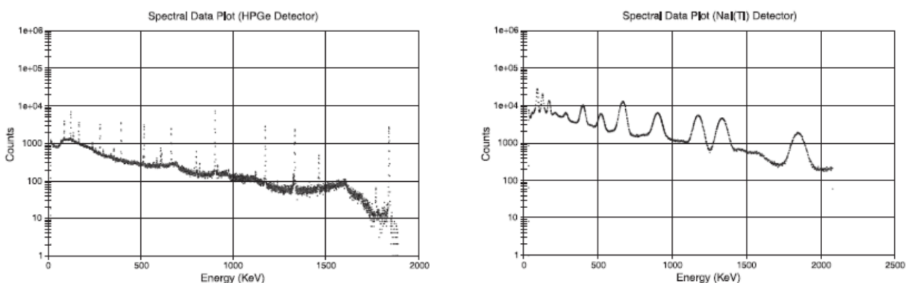
Figure IX.2. Gamma spectra collected from the same source by a semiconductor detector (left) and by a scintillation detector (right) ( http://www.canberra.com/literature/fundamental-principles/ ).
