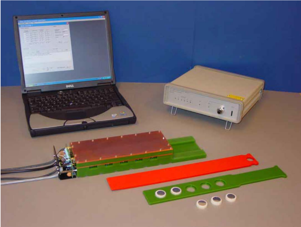
Figure X.4. Risö Beta Counter ( http://www.nutech.dtu.dk/english/Products-and-Services/Dosimetry/Radiation-Measurement-Instruments/GM_multicounter ).
