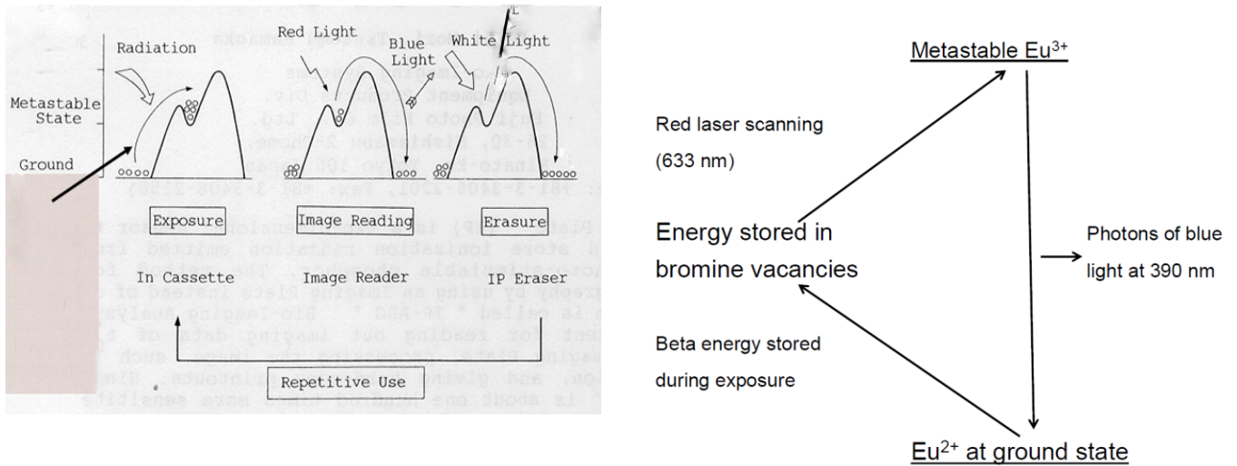
Figure XIII.4. Detection process of beta radiation in a phosphor imaging plate.
