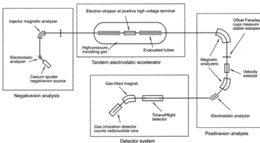
Figure VIII.7. Component of accelerator mass spectrometry (AMS) http://gsabulletin.gsapubs.org/content/115/6/643/F1.expansion.html .
