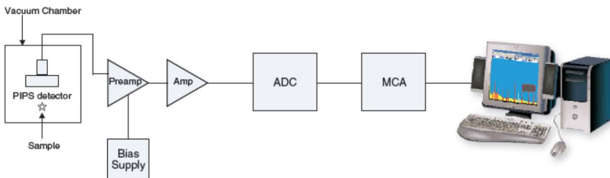
Figure XI.3. Electronics in alpha spectrometry ( http://www.ortec-online.com/Products-Solutions/RadiationDetectors/silicon-charged-particle-detectors.aspx ).
