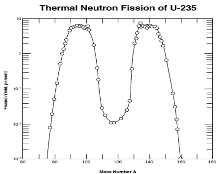
Figure V.4. Distribution of fission products of ^{235}\text{U} ( http://www.science.uwaterloo.ca/~cchieh/cact/nuctek/fissionyield.html ).
