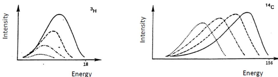
Figure XII.9. The effect of quenching on the beta spectrum in liquid scintillation counting.
