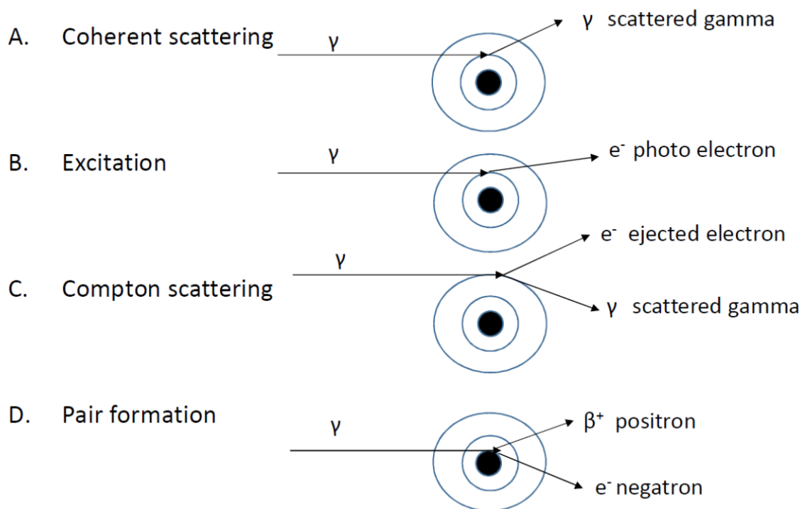
Figure VII.7. Attenuation mechanisms of gamma radiation in media.
