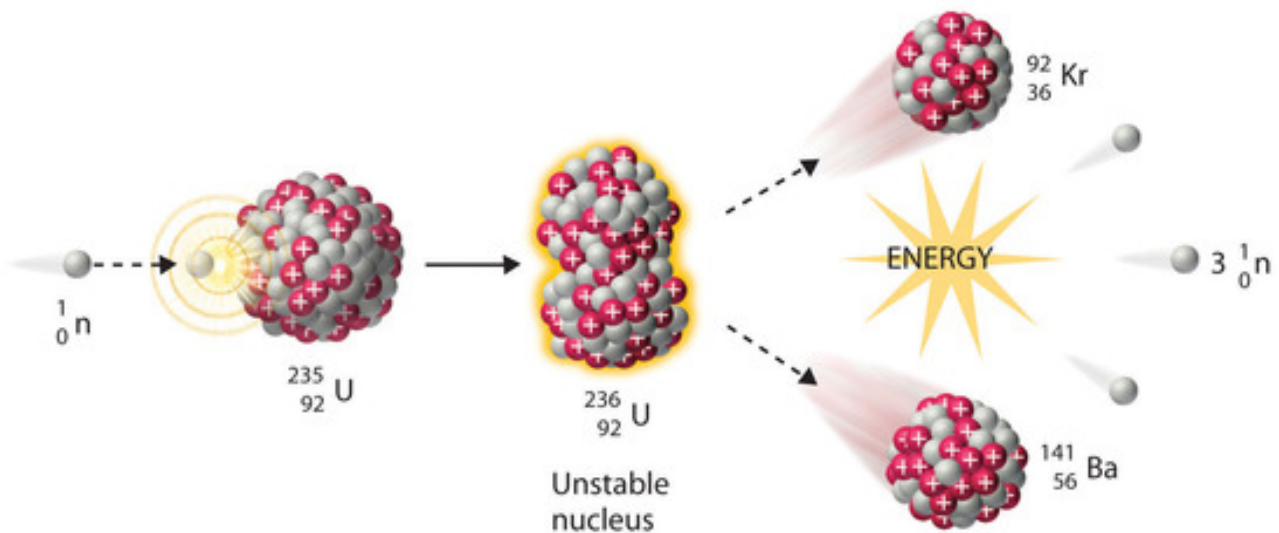
Figure V.2. Induced fission of a heavy nucleus into two nuclei of lighter elements ( http://chemwiki.ucdavis.edu/Physical_Chemistry/Nuclear_Chemistry/Nuclear_Reactions ).
