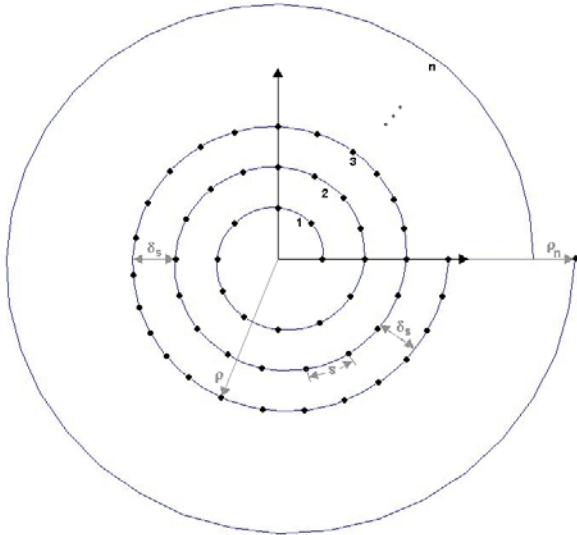
Figure 4. Overhead view of spiral remote sensing survey and parameters.
