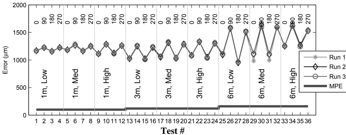
Figure 8. Two-face system test results for Tracker B.
