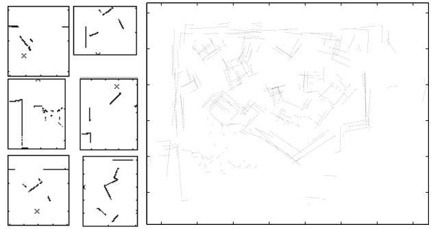
Figure 7: The NIST disaster area data set. Left: 6 example scans (from a total of 60). Crosses show each robot's position. Right: 60 scans superimposed using a rough pre-estimation, building the initial global map.
