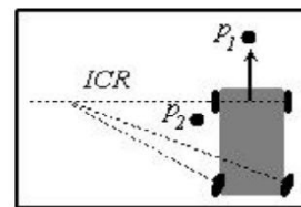
Figure 4. Case of a waypoint ( P_2 ) within the vehicle's ICR.
