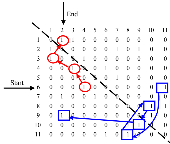
Figure 10: Repeated search algorithm to find all possible combinations of regions constructing a path from a starting region to a destination region
