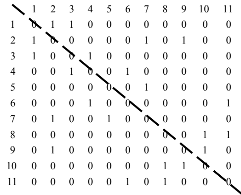
Figure 9: Intersection matrix representing the info on the intersecting free-obstacle regions
