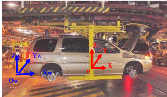
Figure 2 Line Tracking Reference Frames
