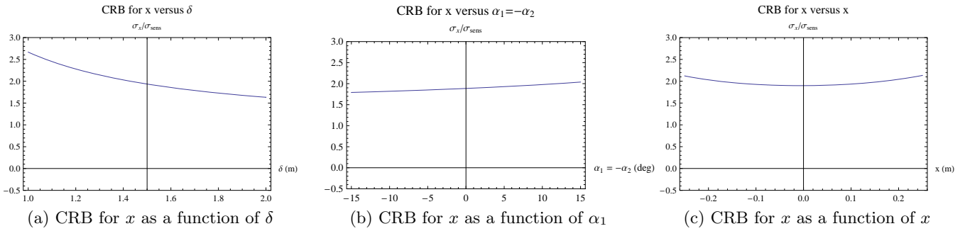
Figure 2: Changes in the CRB for x as a function of small perturbations of the other variables.
