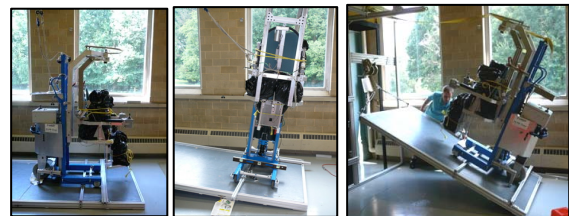
Figure 3: Photos of example test configurations, including: (left) forward, (middle) lateral, and (right) rear configurations.
