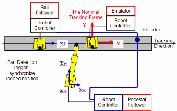
Figure 4 Encoder Connects to the Robot Controller of the Rail or Pedestal Follower
