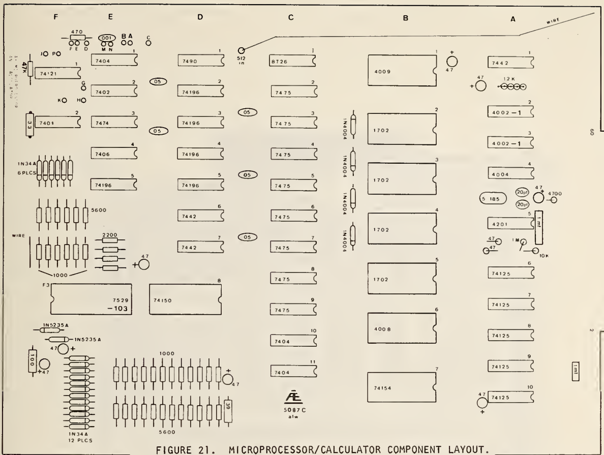
FIGURE 21. MICROPROCESSOR/CALCULATOR COMPONENT LAYOUT.
