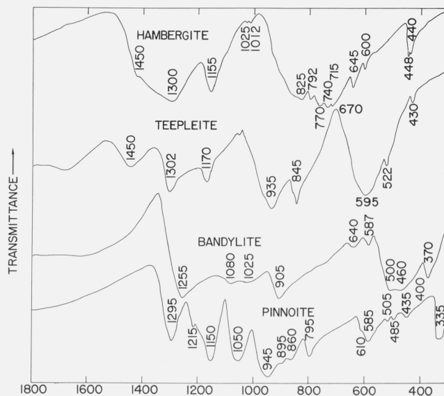
FIGURE 1. Infrared absorption spectra of hydrated borates containing simple anions.
