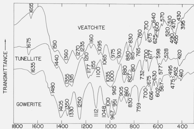
FIGURE 3. Infrared absorption spectra of \text{MeO} \cdot 3\text{B}_2\text{O}_3 \cdot \text{XH}_2\text{O} compounds.
