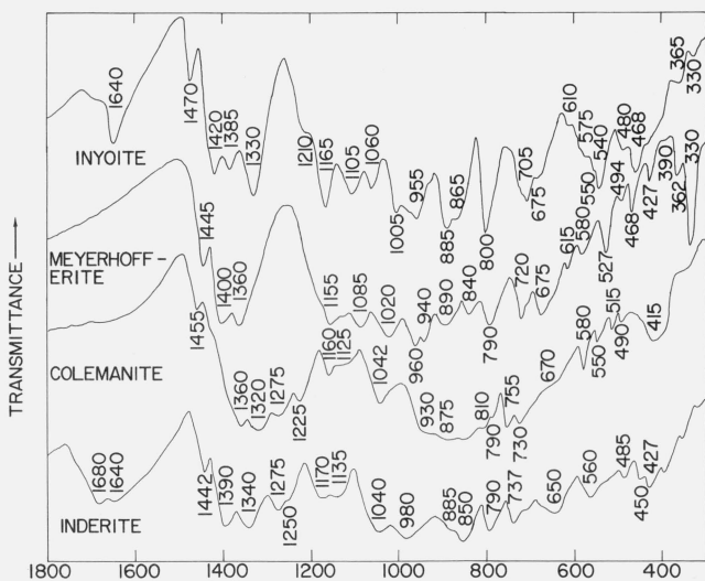
FIGURE 2. Infrared absorption spectra of 2\text{MeO} \cdot 3\text{B}_2\text{O}_3 \cdot \text{XH}_2\text{O} compounds.
