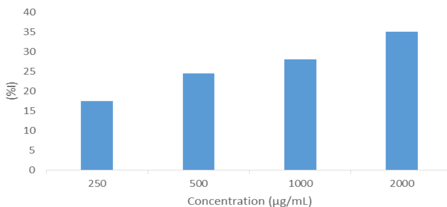
Figure 4. Radical scavenging activity of DPPH by the essential oil.
