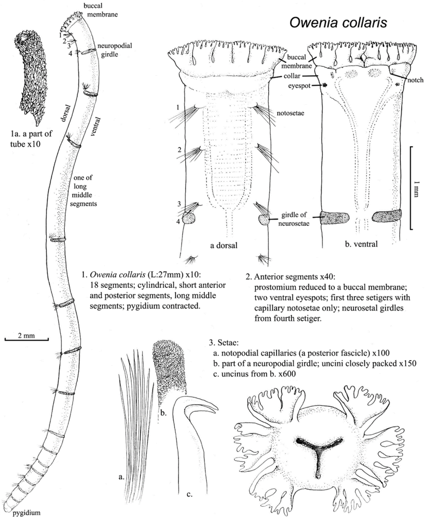
4. Lips, from above x40: one dorsal, two ventral lobes (after Watson, 1901).
