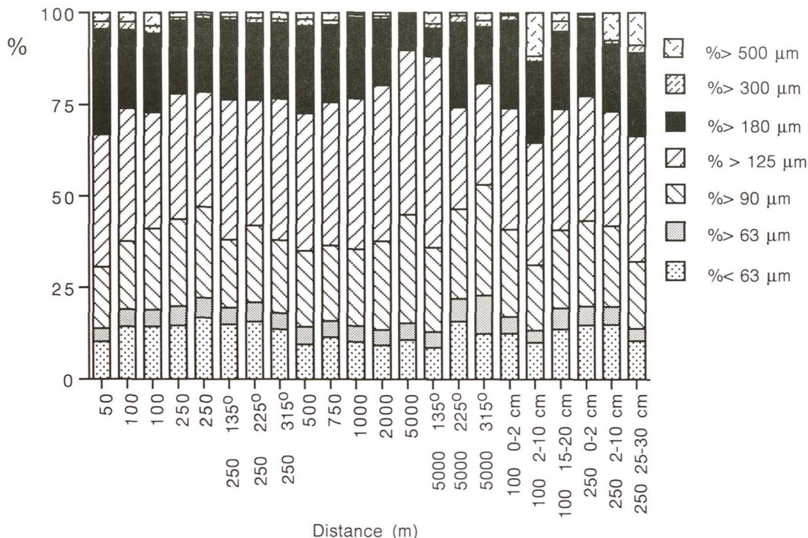
Fig. 3. Grainsize distribution along the different transects (data from GROENEWOLD, 1995).
