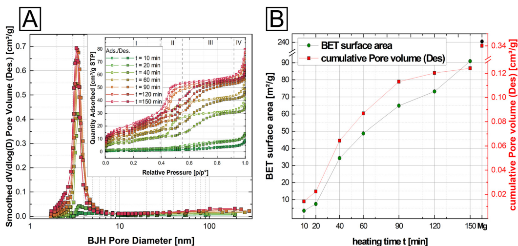
Fig. 3 \text{N}_2 adsorption/desorption BET surface measurements for a time series (10–150 min) of isothermally heated Ni-struvite at 90 °C (A) average desorption BJH pore size change ( dV/d \log(D) pore volume [ \text{cm}^3 \text{g}^{-1} ] vs. average pore diameter [nm]), inset: evolution of type IV adsorption/desorption isotherms of the t-series (B) Temporal evolution of BET surface area [ \text{m}^2 \text{g}^{-1} ] (green circles) and des. cumulative pore volume [ \text{cm}^3 \text{g}^{-1} ] (red squares) of thermally treated Ni-struvite with heated Mg-struvite as a reference (black circle: BET surface area, red circle: cumulative pore volume).
