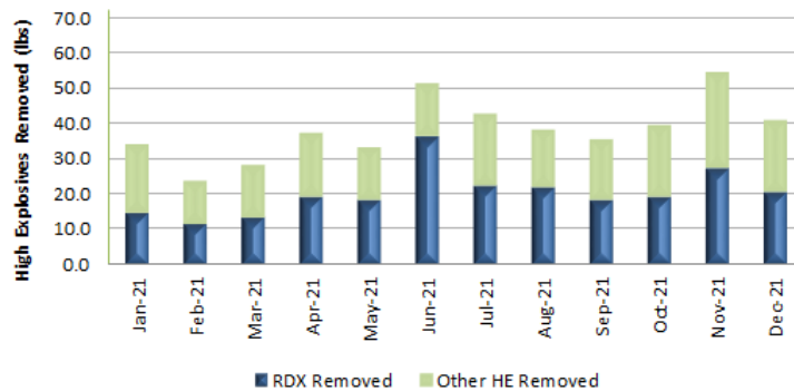
Figure 2-14. SEPTS High Explosive Mass Removal by Month
