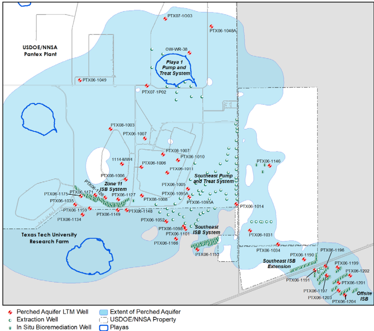
Figure 3-11. Perched Wells with Unexpected COC Trends
