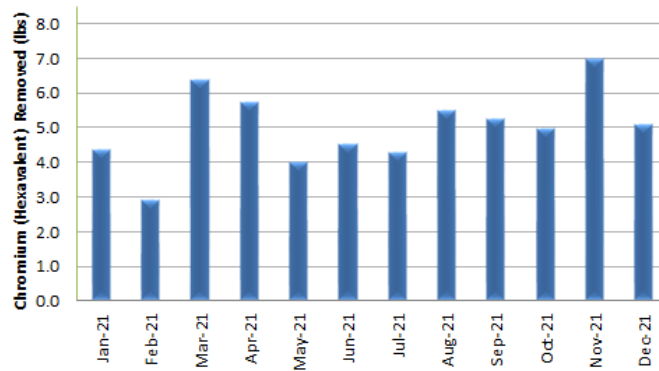
Figure 2-13. SEPTS Chromium Mass Removal by Month
