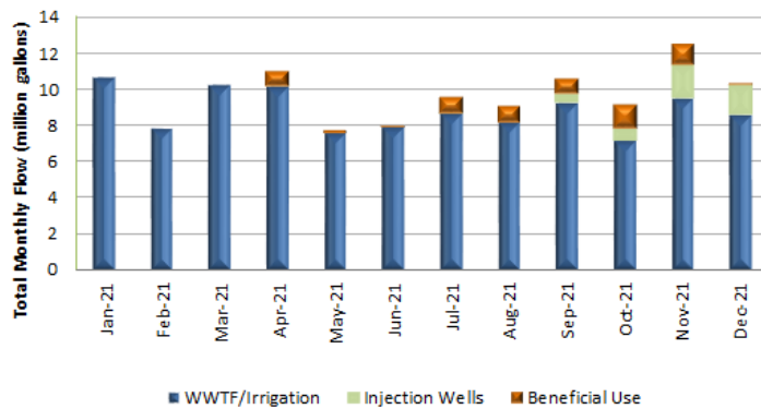
Figure 2-12. SEPTS Total Flow Volume and Disposition of Effluent
