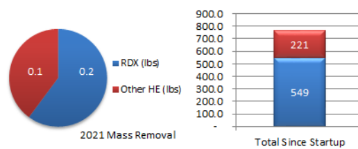
Figure E-4. P1PTS Mass Removal
