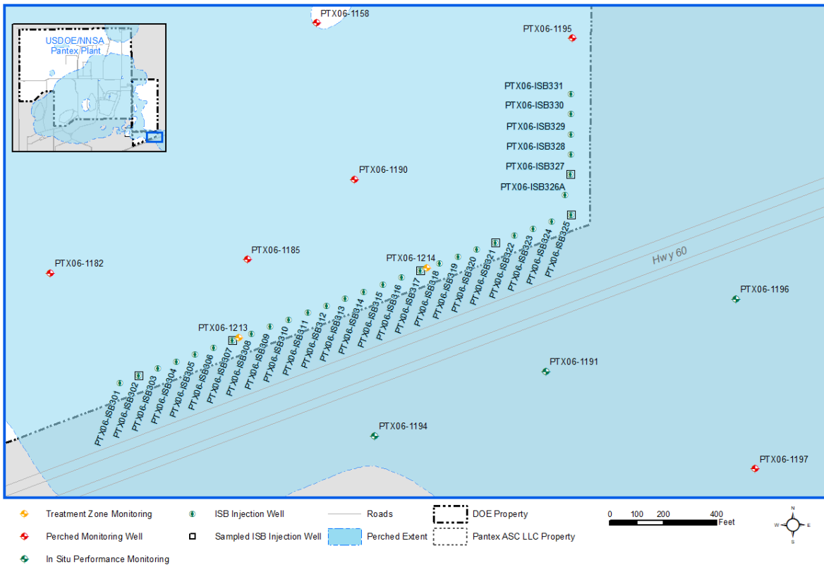
Figure 1-10. Southeast ISB Extension Treatment Zone and Performance Monitoring Wells
