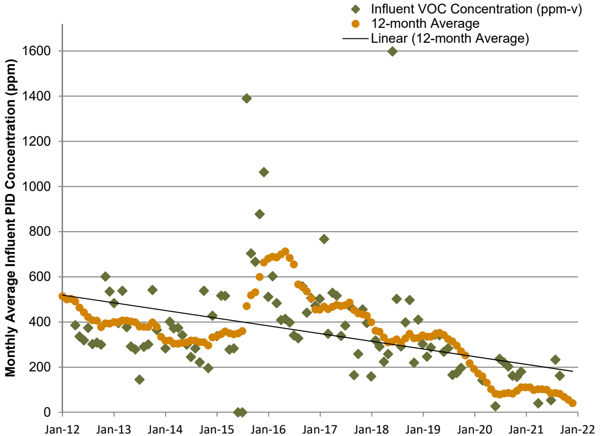
Figure 4-4. Influent Average PID VOC Concentrations vs. Time
