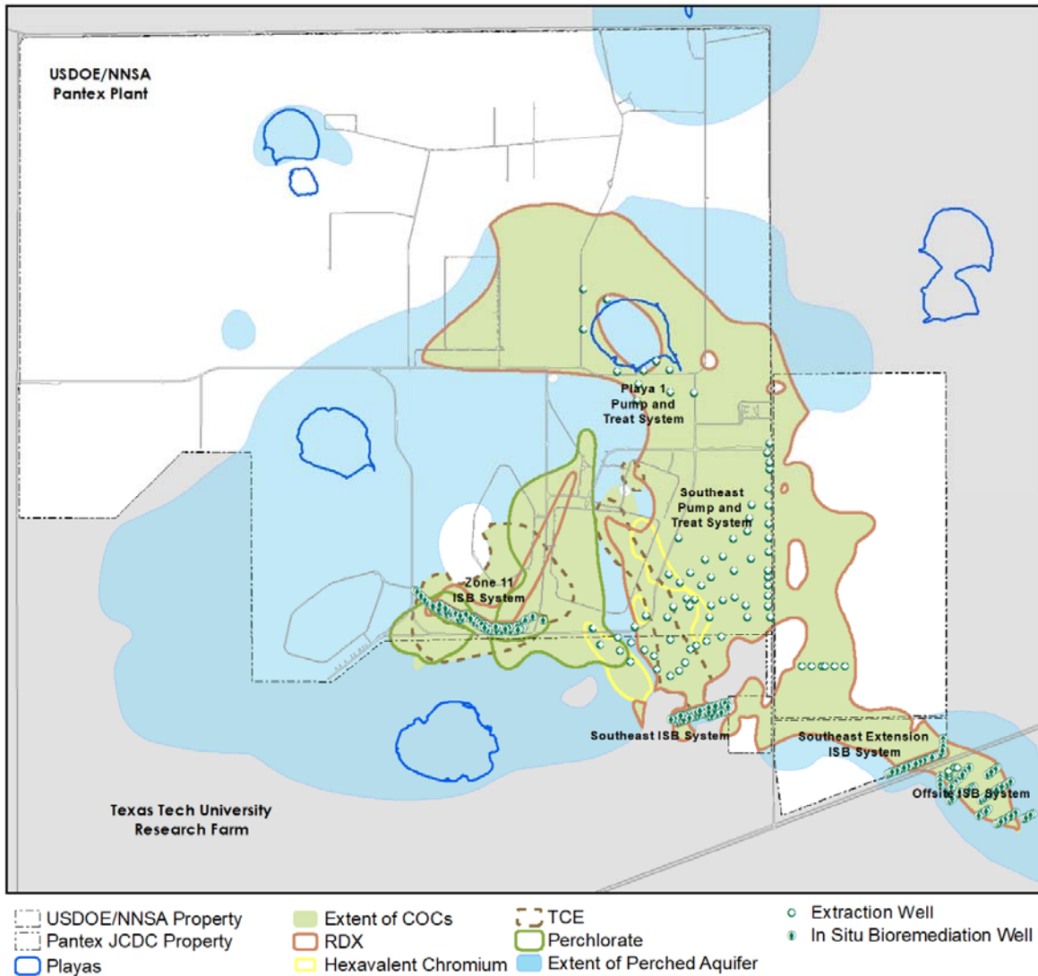
Figure E-8. Major COC Plumes in the Perched Aquifer
