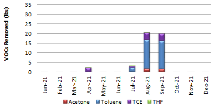
Figure 2-17. Burning Ground SVE Mass Removal
