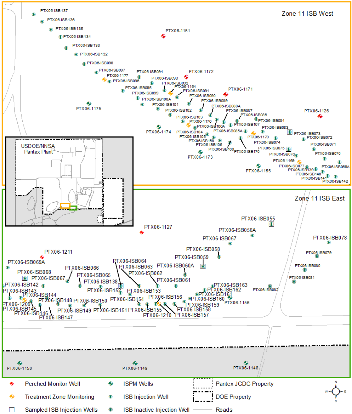
Figure 1-8. Zone 11 ISB Treatment Zone and Performance Monitoring Wells
