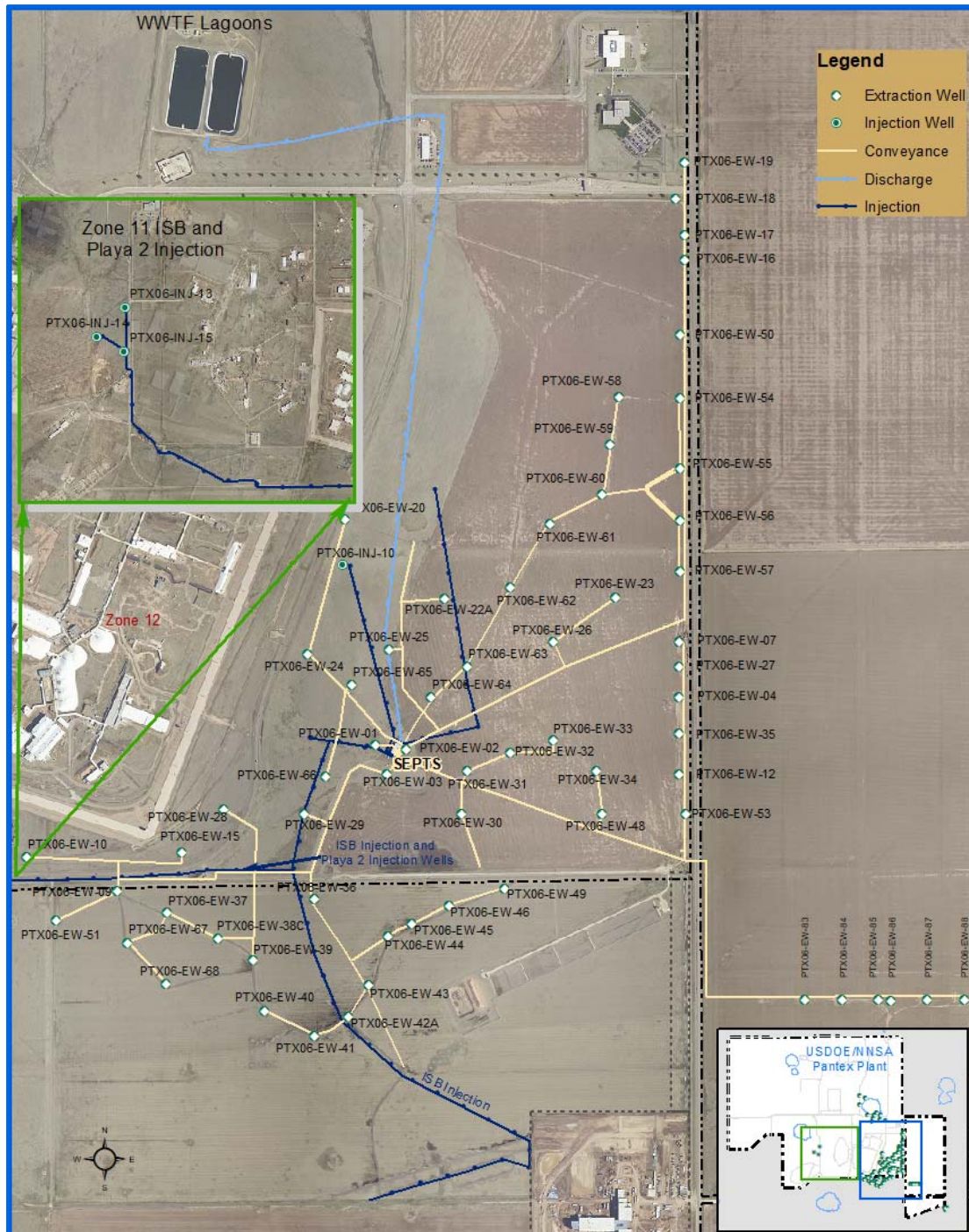
Figure 1-7. SEPTS Wells and Conveyance Lines
