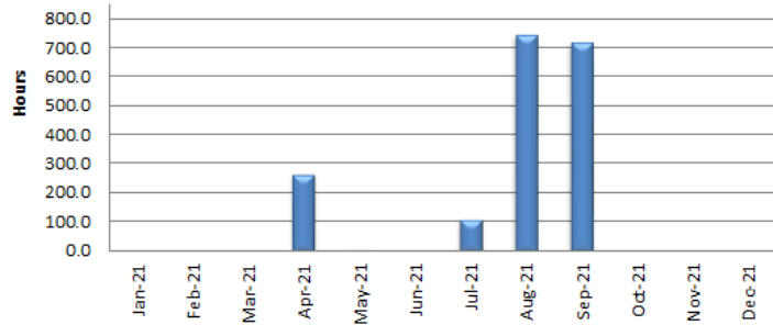
Figure 2-16. SVE System Operation
