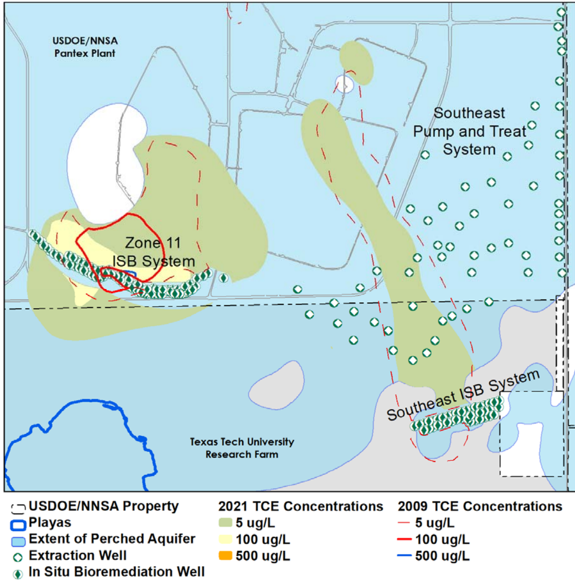
Figure 3-30. TCE Plume Movement, 2009-2021
