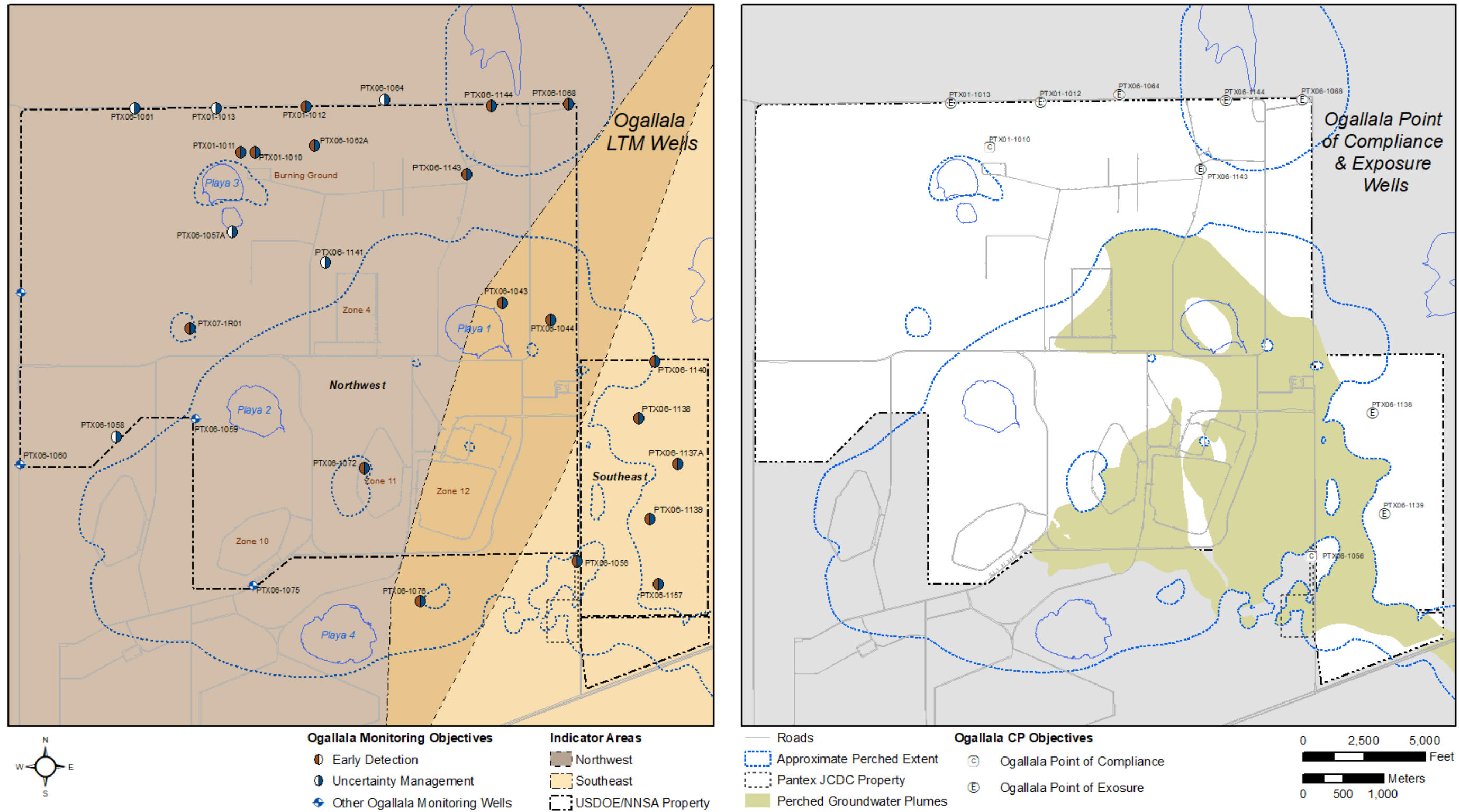
Figure 1-13. Ogallala Aquifer LTM Network and Compliance Plan Wells
