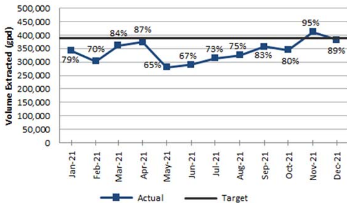
Figure 2-11. SEPTS Average GPD and % Capacity
