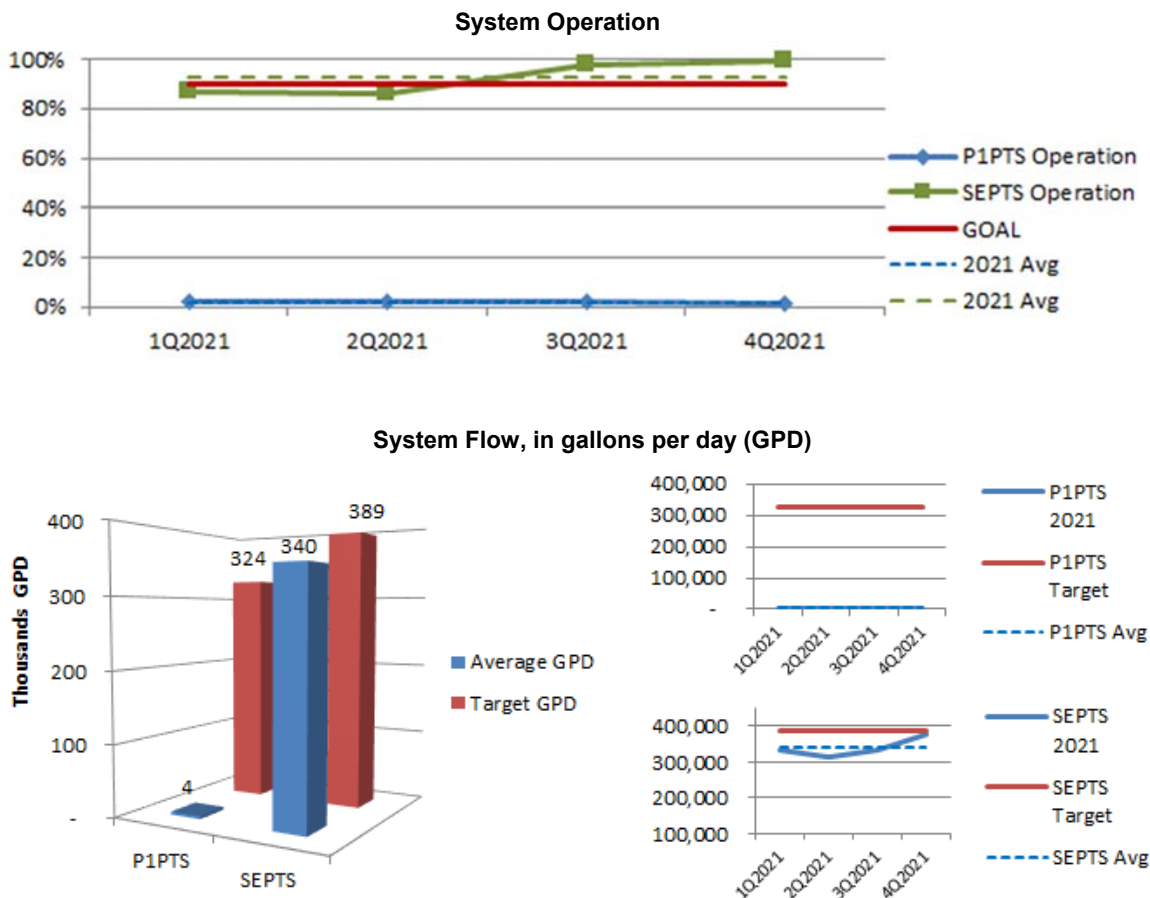
Figure E-1. Pump and Treat System Performance
