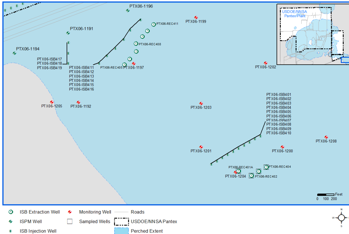
Figure 1-11. Offsite Treatment Zone and Performance Monitoring Wells
