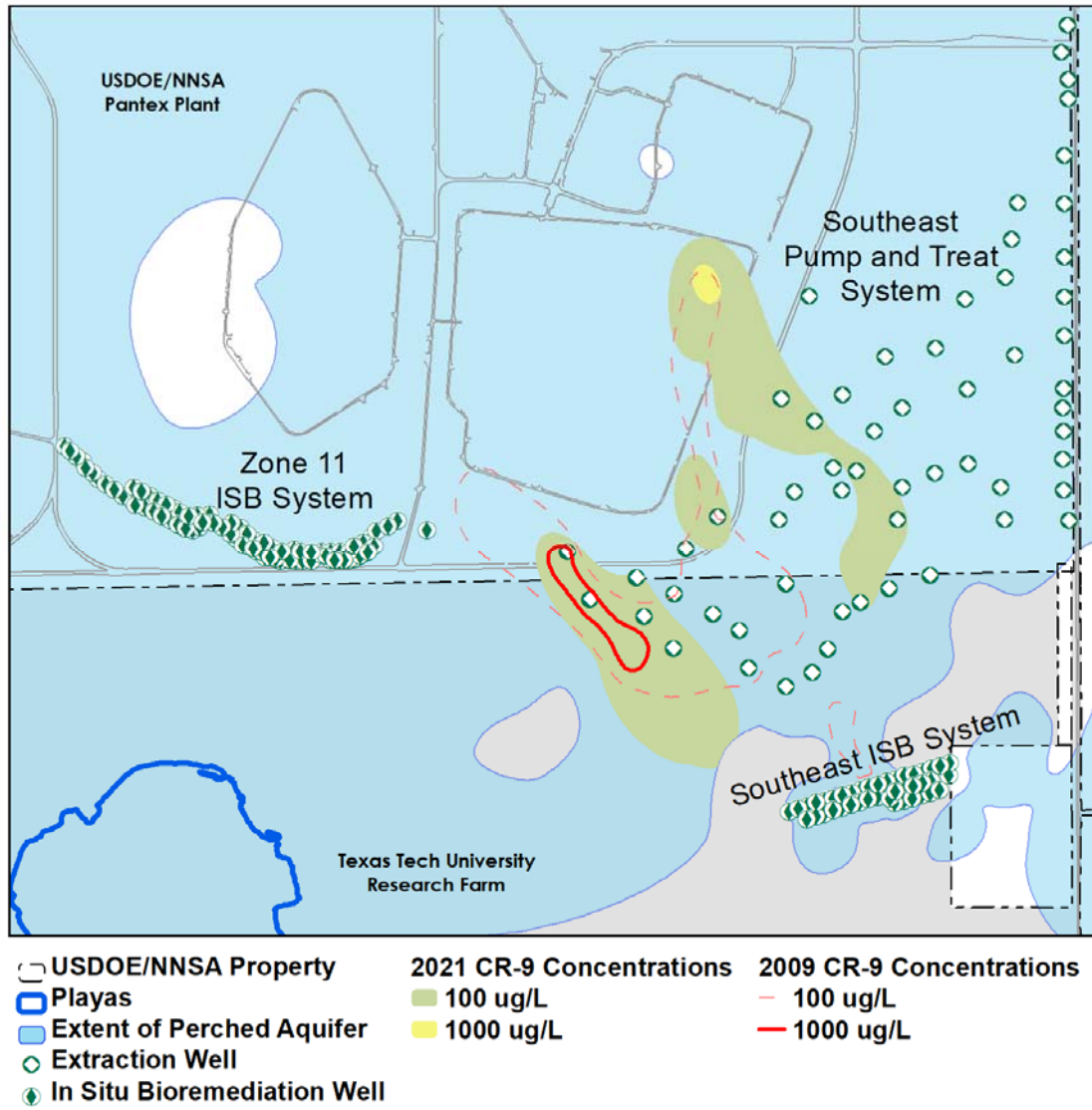
Figure 3-28. Hexavalent Chromium Plume Movement, 2009-2021
