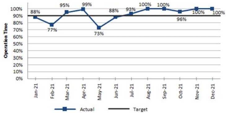
Figure 2-7. SEPTS Operation Time vs Target
