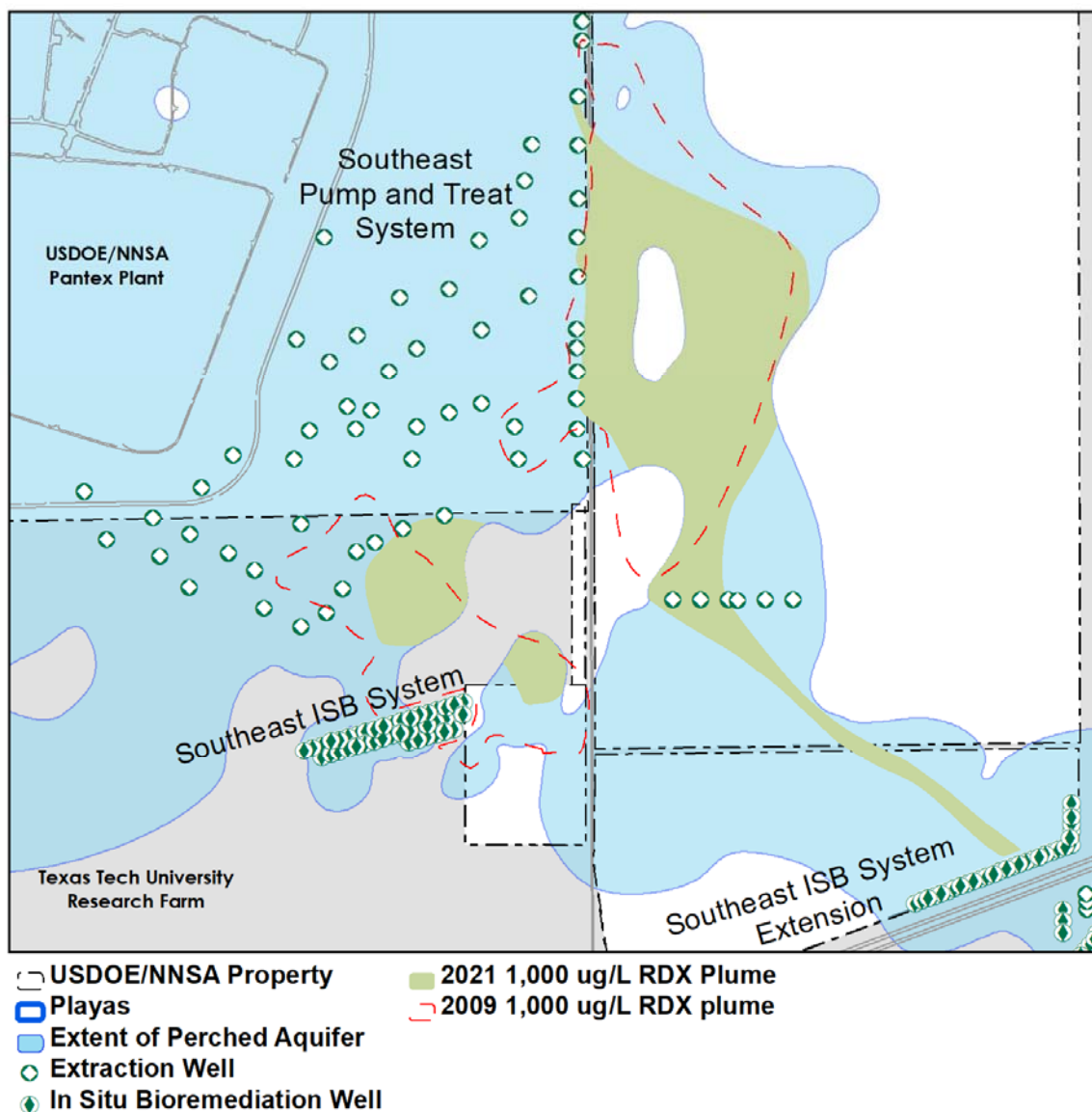
Figure 3-27. RDX Plume Movement, 2009-2021
