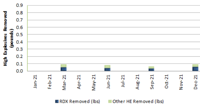
Figure 2-6. P1PTS Mass Removal by Month
