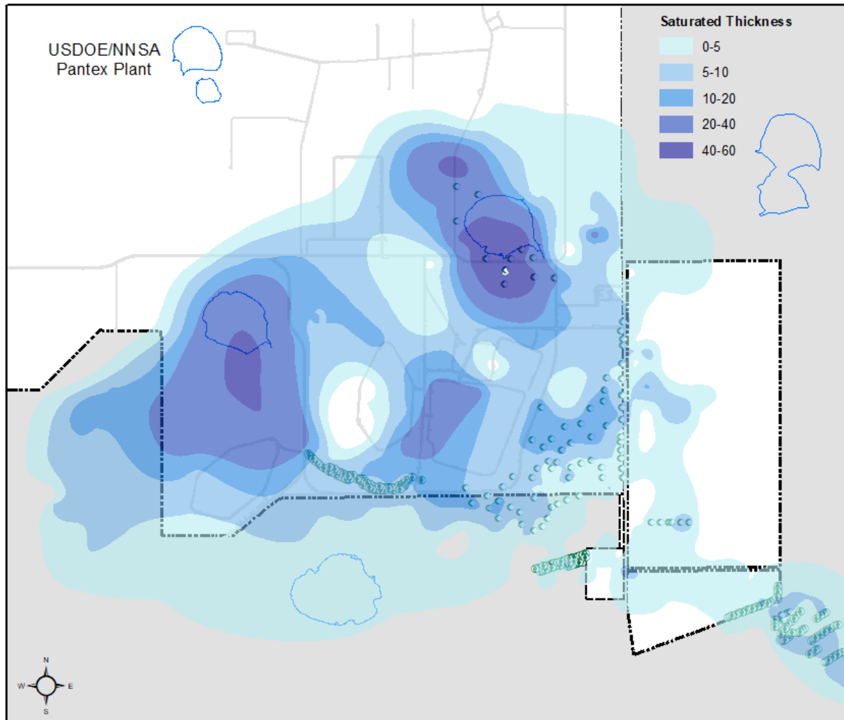
Figure 2-15. Perched Aquifer Saturated Thickness, 2021
