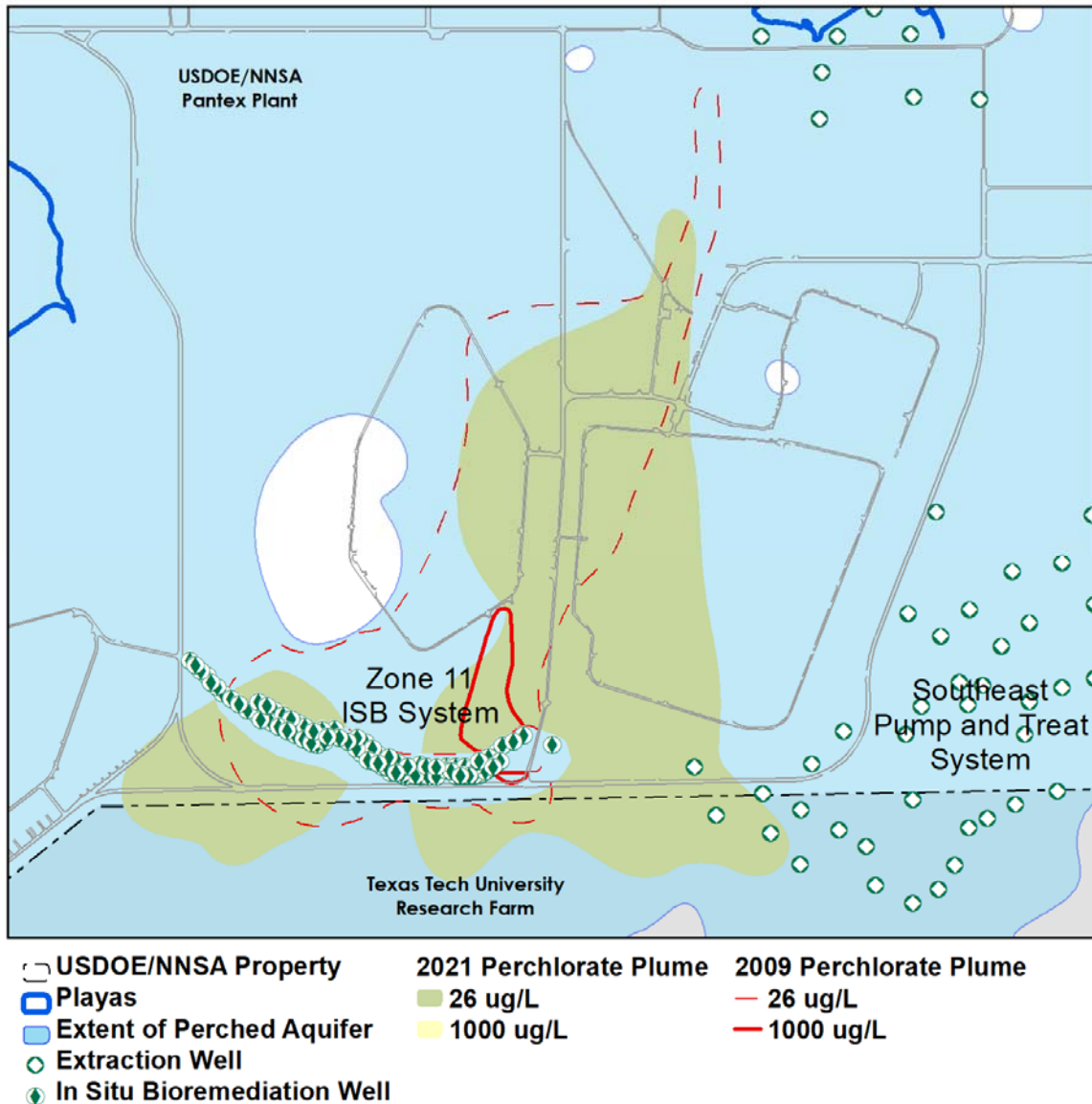
Figure 3-29. Perchlorate Plume Movement, 2009-2021
