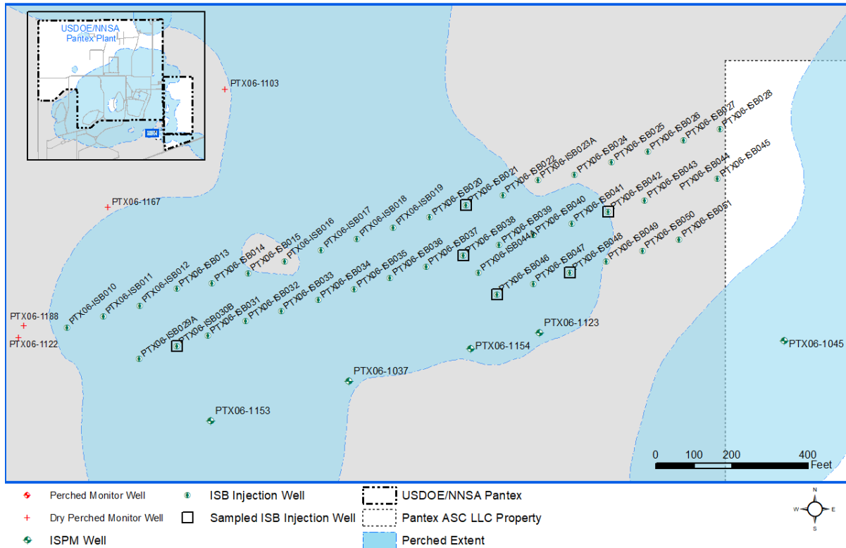
Figure 1-9. Southeast ISB Treatment Zone and Performance Monitoring Wells
