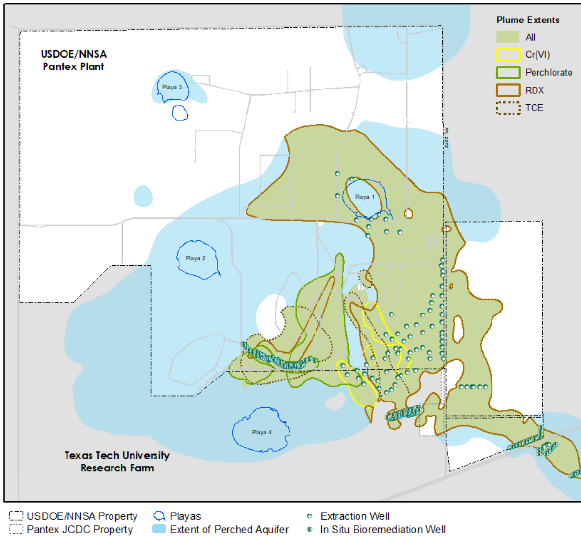
Figure 1-2. Extent of Perched Groundwater and Contaminant Plumes Exceeding the Groundwater Protection Standard
