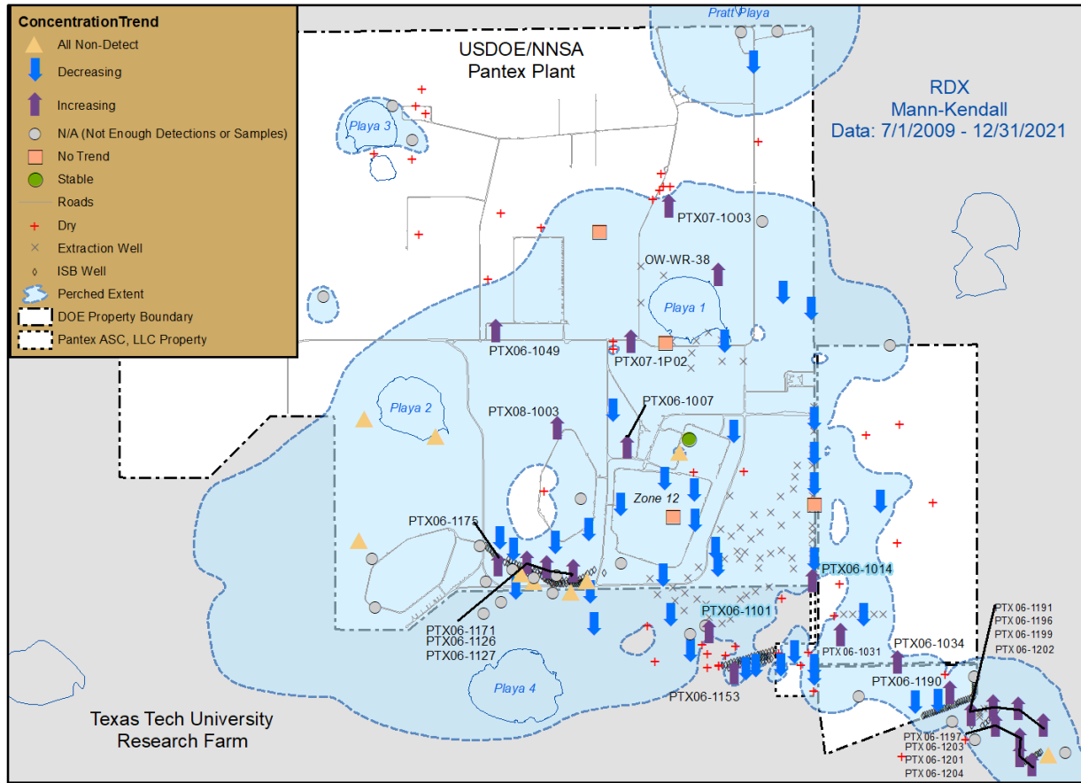
Figure E-7. RDX Trends in the Perched Aquifer
