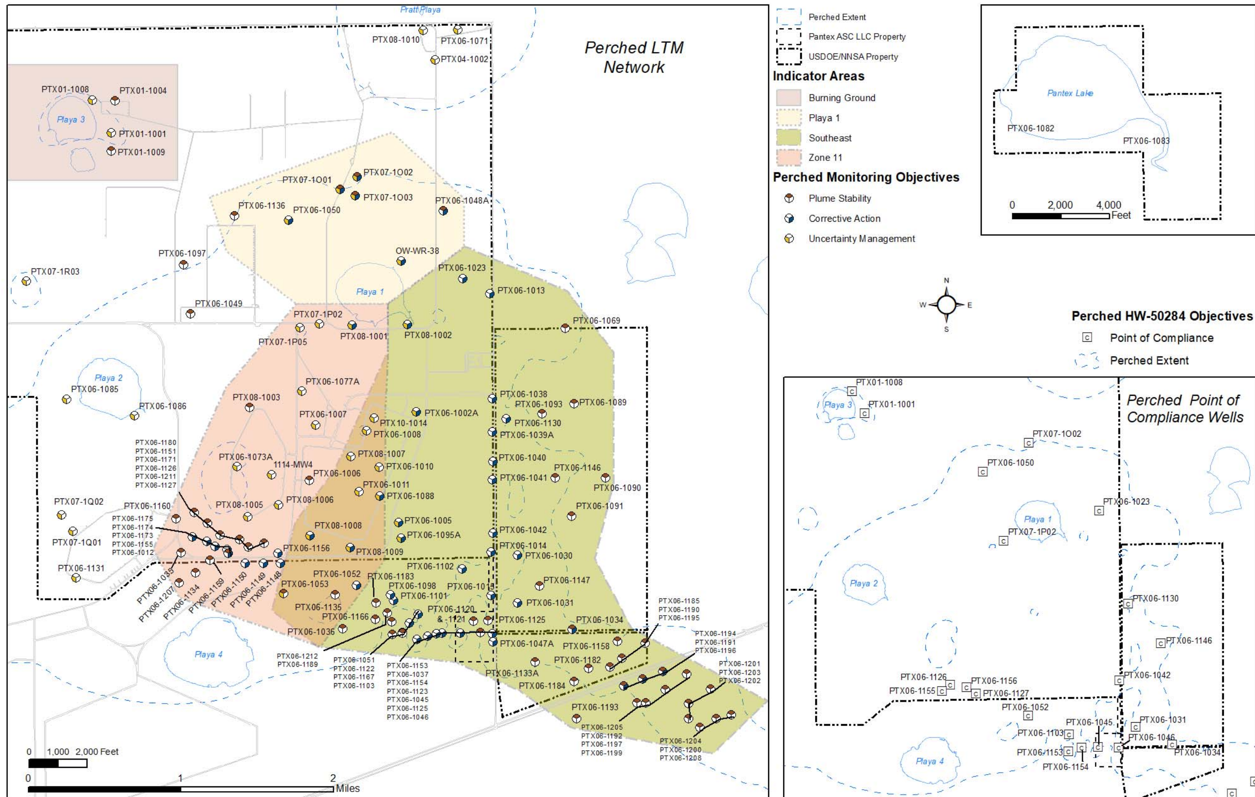
Figure 1-12. Perched LTM Network and Compliance Plan Wells
