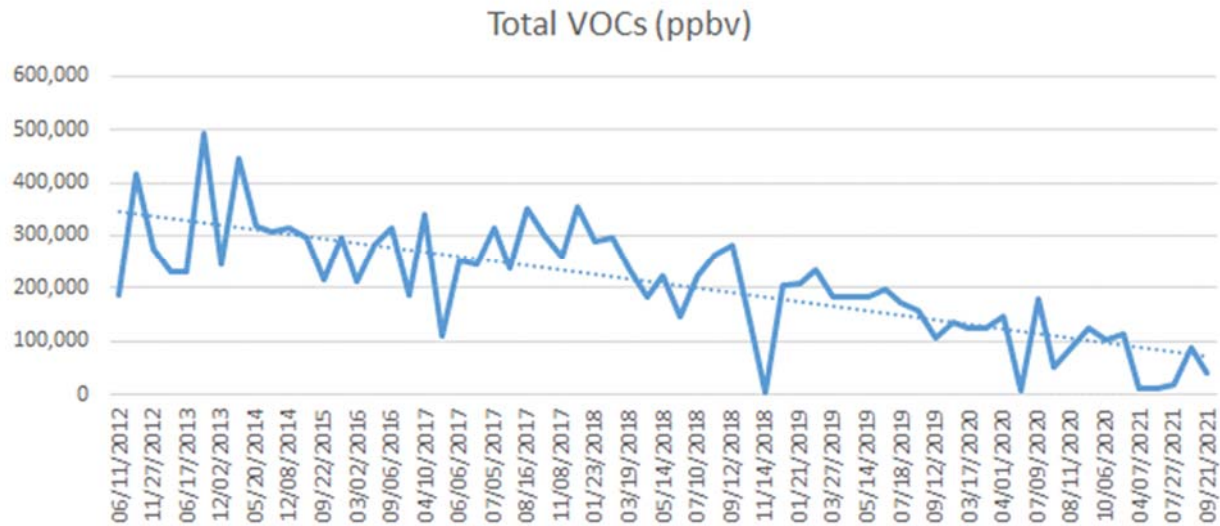
Figure 4-3. Total VOCs Since Installation of Current CatOX System
