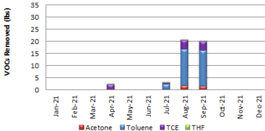
Figure 4-2. SVE System 2021 VOC Removal
