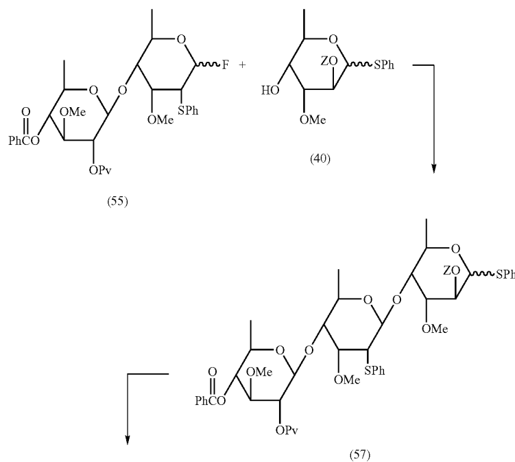
Reaction Scheme F
