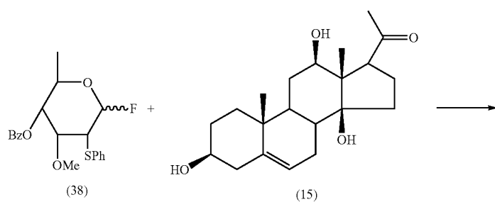
Reaction Scheme E
