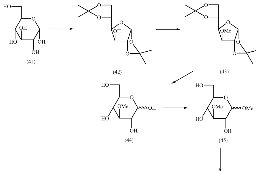
Reaction Scheme D
