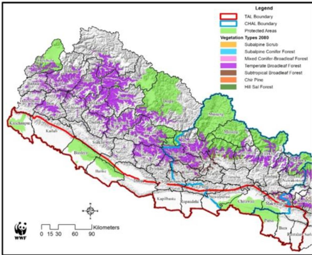
Figure 6. Resilient patches of the vegetation types in 2080 under the A2A climate projection scenario. These patches represent the areas where the vegetation composition is not expected to change under the A2A climate projection, and does not represent forest loss or fragmentation due to non-climate related anthropogenic activities.
