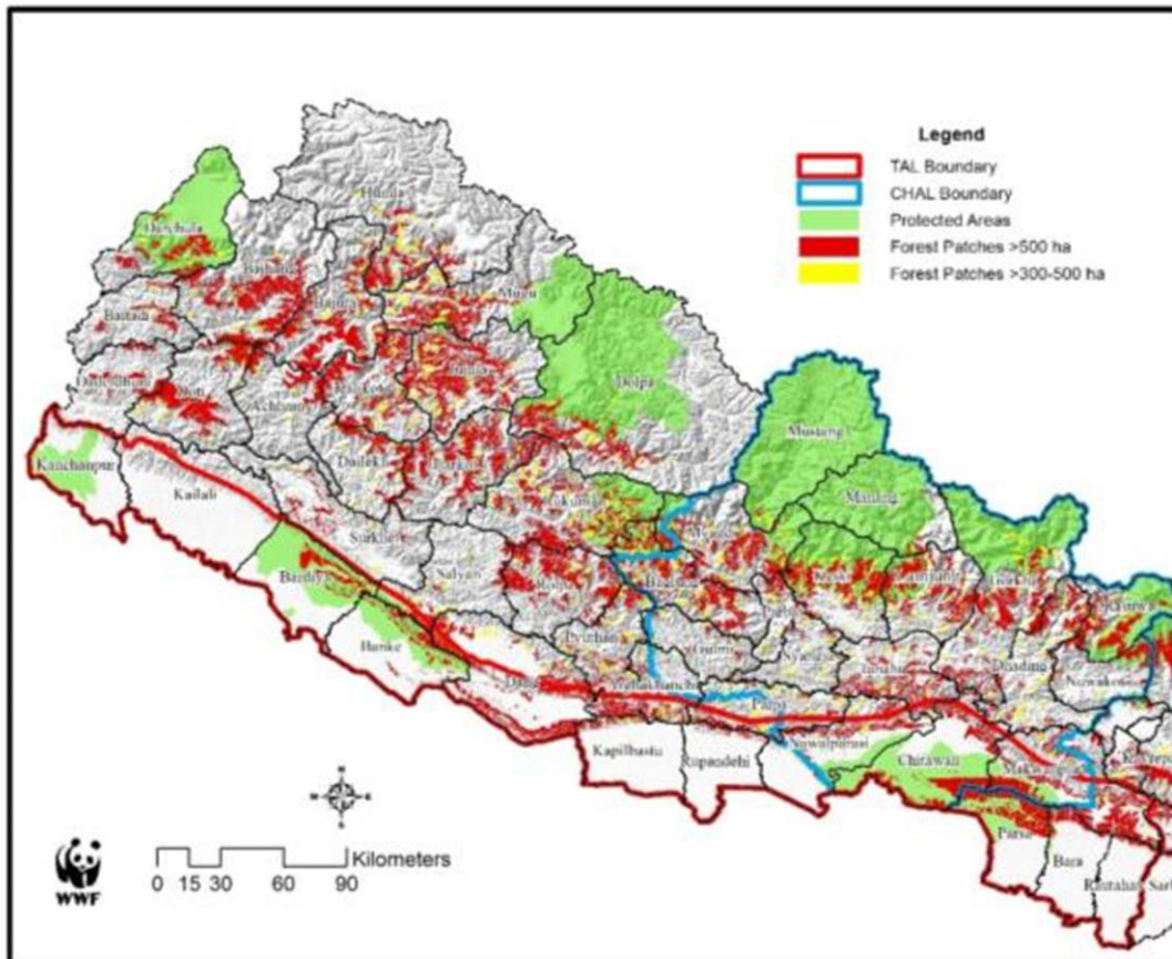
Figure 8. Distribution of larger patches of resilient forests in 2020. These represent potential climate 'macrorefugia' (sensu Ashcroft 2010).
