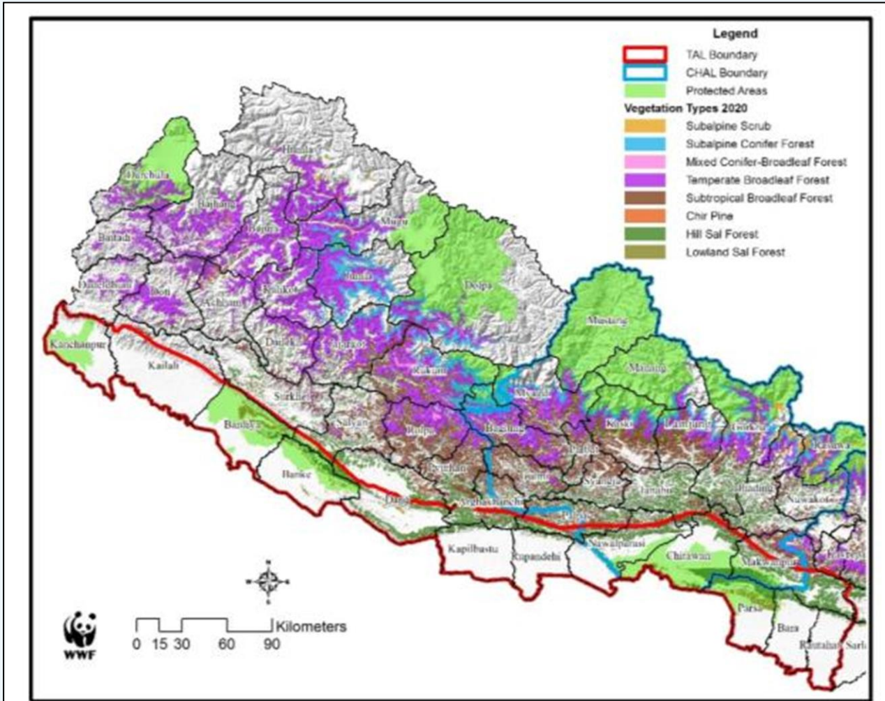
Figure 4. Resilient patches of the vegetation types in 2020 under the A2A climate projection scenario. These patches represent the areas where the vegetation composition is not expected to change under the A2A climate projection, and does not represent forest loss or fragmentation due to non-climate related anthropogenic drivers.
