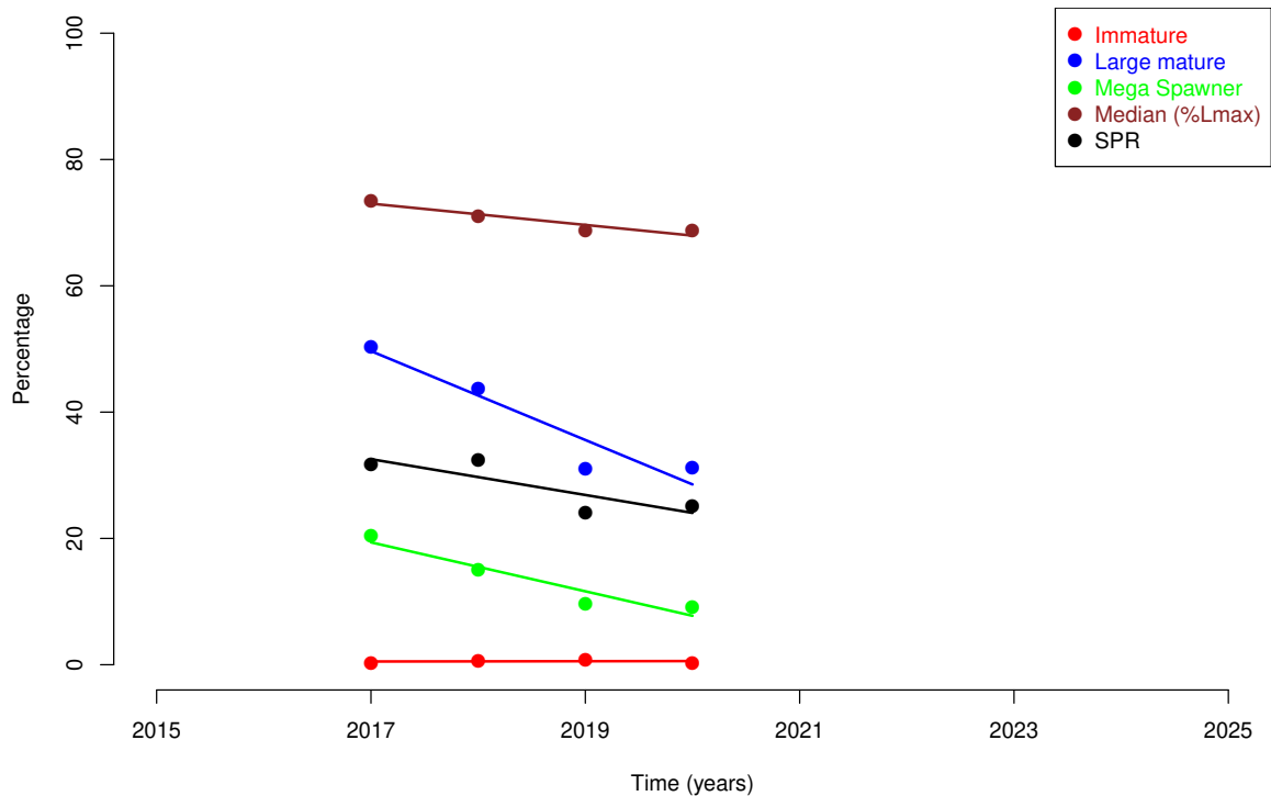
Trends in relative abundance by size group for Epinephelus bleekeri (ID #46, Epinephelidae) in WPP 718.
