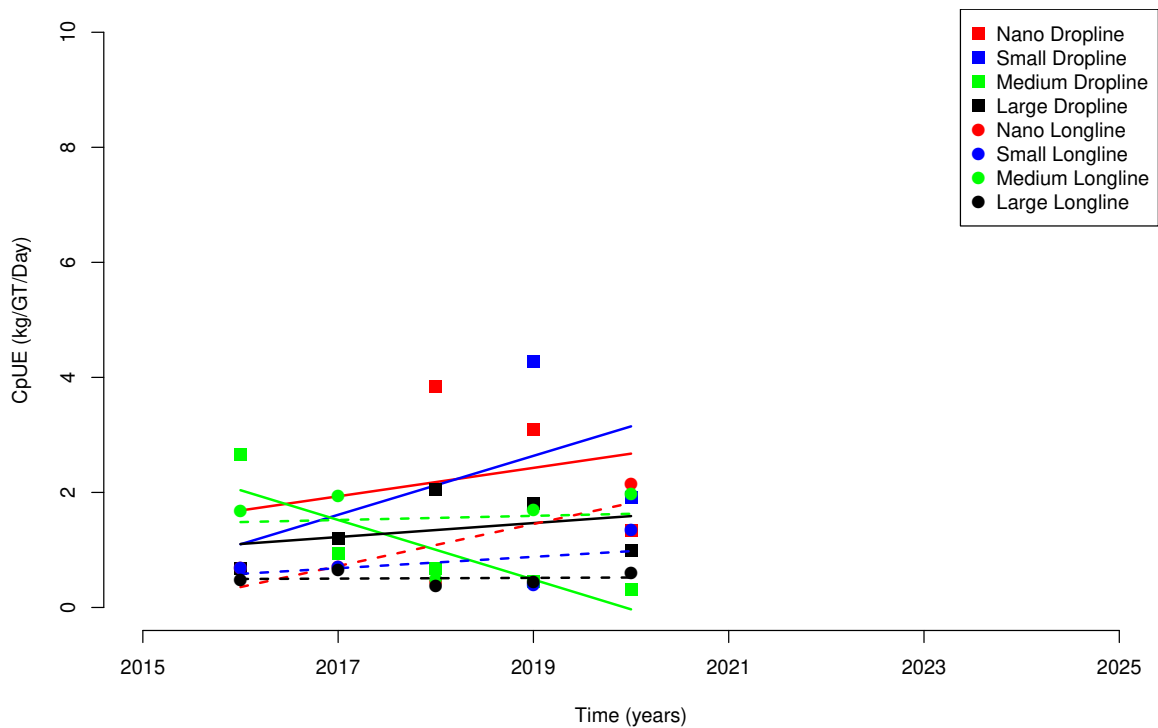
Figure 2.6: Catch per Unit of Effort per calendar year for Pristipomoides multidens in WPP 718 for Dropline and Longline catches by fleet segment. Solid lines and dashed lines for trends in Dropline CpUE and Longline CpUE respectively.
