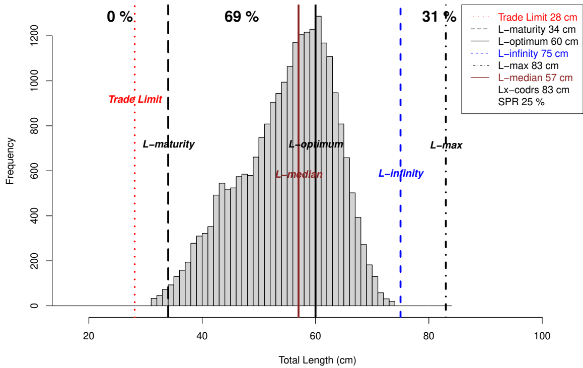
Catch length frequency for Epinephelus bleekeri (ID #46, Epinephelidae) in WPP 718 in 2020. N (Catch) = 24,313, n (Sample) = 1,506.
