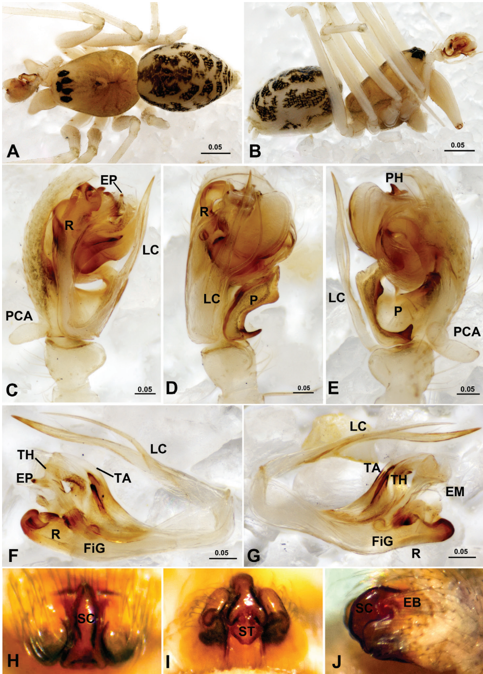
Figure 6. Acanthoneta dokutchbaevi (A–G) and Acanthoneta aggressa (H–J). A male, dorsal B male, lateral C male palp, prolateral D male palp, ventral E male palp, retrolateral F embolic division, ventral G embolic division, dorsal H epigynum, ventral I epigynum, posterior J epigynum, lateral ( H–J ) photos provided by Don Buckle). EB epigynal basal part; EM embolic membrane; EP embolus proper; FiG Fickert's gland; LC lamella characteristic; P paracymbium; PCA proximal cymbial apophysis; PH pit hook; R radix; SC scape; ST stretcher; TA terminal apophysis; TH thumb of embolus. [Scale bars: mm].
