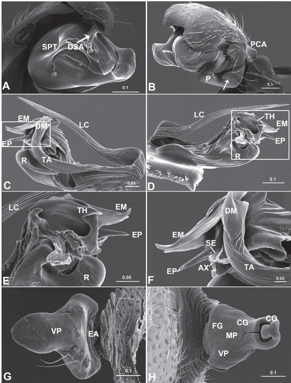
Figure 4. Acanoides beijingsis sp. n. A palp (embolic division removed), prolateral B palp, retrolateral, arrow indicates half rounded lateral tooth on paracymbium C embolic division, ventral D embolic division, dorsal E detail of D F detail of C G epigynum, ventral H epigynum, dorsal. AX apex of embolus; CG copulatory groove; CO copulatory opening; DM distal membrane of terminal apophysis; DSA distal suprategular apophysis; EA extensible area of epigynal basal part; EM embolic membrane; EP embolus proper; FG fertilization groove; LC lamella characteristica; MP median plate; P paracymbium; PCA proximal cymbial apophysis; R radix; S spermatheca; SE serrated area on embolus; SPT suprategulum; TA terminal apophysis; TH thumb of embolus; VP ventral plate. [Scale bars: mm].
