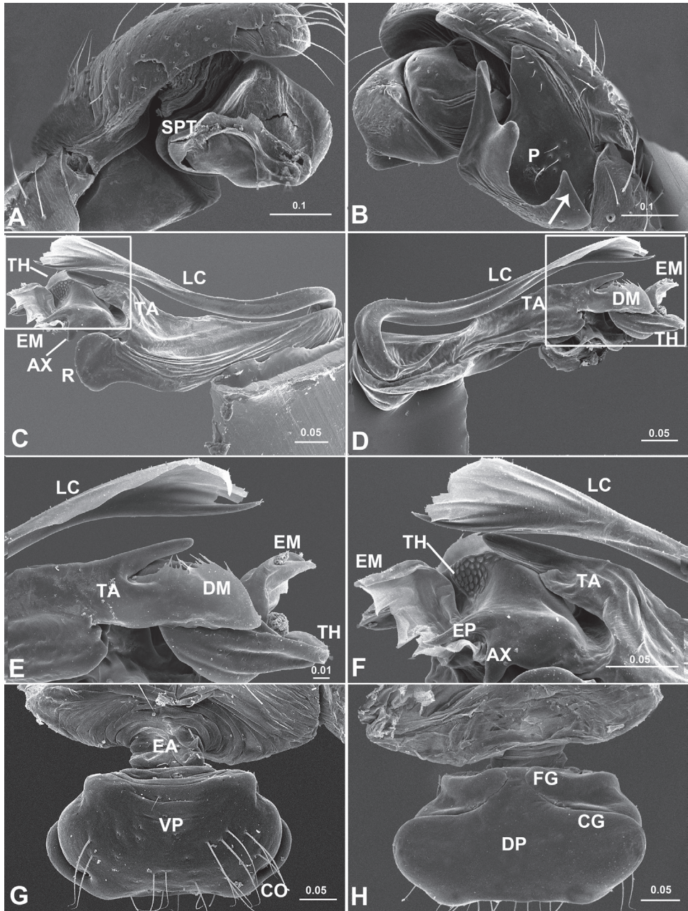
Figure 5. Acanoides bengshanensis . A palp (embolic division removed), prolateral B palp, retrolateral, arrow indicates pointed tooth on posterolateral margin C embolic division, ventral D embolic division, dorsal E detail of D F detail of C G epigynum, ventral H epigynum, dorsal. AX apex of embolus; CG copulatory groove; CO copulatory opening; DM distal membrane of terminal apophysis; EA extensible area of epigynal basal part; EM embolic membrane; EP embolus proper; FG fertilization groove; LC lamella characteristic; P paracymbium; PCA proximal cymbial apophysis; R radix; S spermatheca; SPT suprategulum; TA terminal apophysis; TH thumb of embolus; VP ventral plate. [Scale bars: mm].
