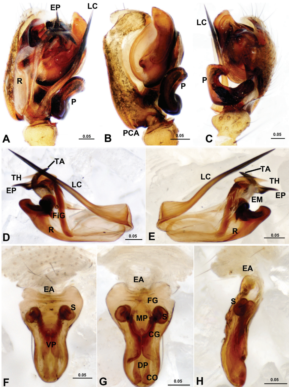
Figure 2. Acanoides beijingsensis sp. n. A male palp, prolateral B male palp, prolateral, with embolic division removed C male palp, retrolateral D embolic division, ventral E embolic division, dorsal F epigynum, ventral G epigynum, dorsal H epigynum, lateral. CG copulatory groove; CO copulatory opening; DP dorsal plate; EA extensible area of epigynal basal part; EM embolic membrane; EP embolus proper; FG fertilization groove; FiG Fickert's gland; LC lamella characteristica; MP median plate; P paracymbium; PCA proximal cymbial apophysis; R radix; S spermathecae; TA terminal apophysis; TH thumb of embolus; VP ventral plate. [Scale bars: mm].
