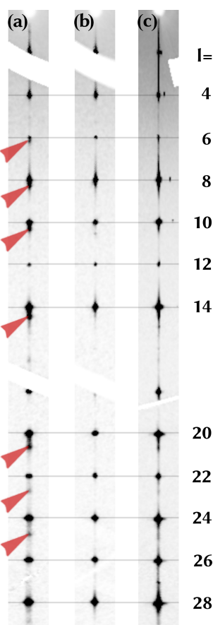
Figure 9. Diffuse scattering of three crystals of kahlenbergite is shown. Stripes (along the 00l line) of the reciprocal space layer 0kl are compared. Crystal (a) shows extra reflections (red arrows), which are caused by domains of hibonite, whereas crystal (c) exhibits stronger diffuse scattering and only broad maxima at the positions of the hibonite peaks. Data of crystal (b) were used for the structure refinement as the crystal's diffuse scattering is weak.
