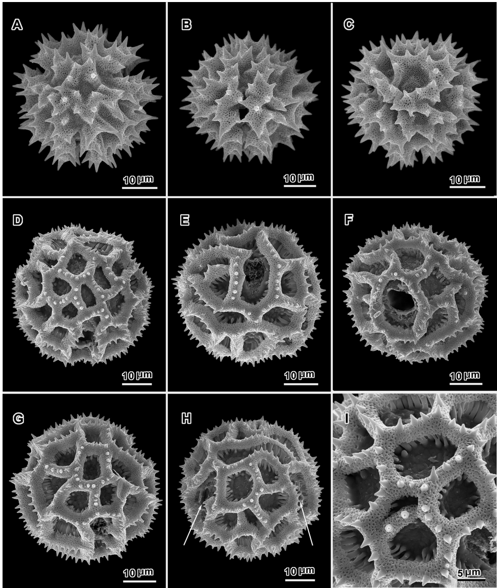
Figure 25. Scanning electron micrographs of Vernonella and Vernoniastrum . A–C Scanning electron micrographs of acetolyzed sublophate-echinolophate pollen of Vernonella africana Sond. A Polar view B Equatorial view C Oblique polar view. A–C from Wood 753. D–I Scanning electron micrographs of acetolyzed echinolophate pollen of Vernoniastrum nestor (S. Moore) H. Rob., showing diversity of lacunae and lophae. D–H Oblique and near polar views showing apertures in markedly long lacunae with irregular lophae H Lateral view with apertures (arrows) occupying long lacunar spaces I Enlarged section of surface showing columellae in irregular rows under muri). D–I from Reekmans 9185.
