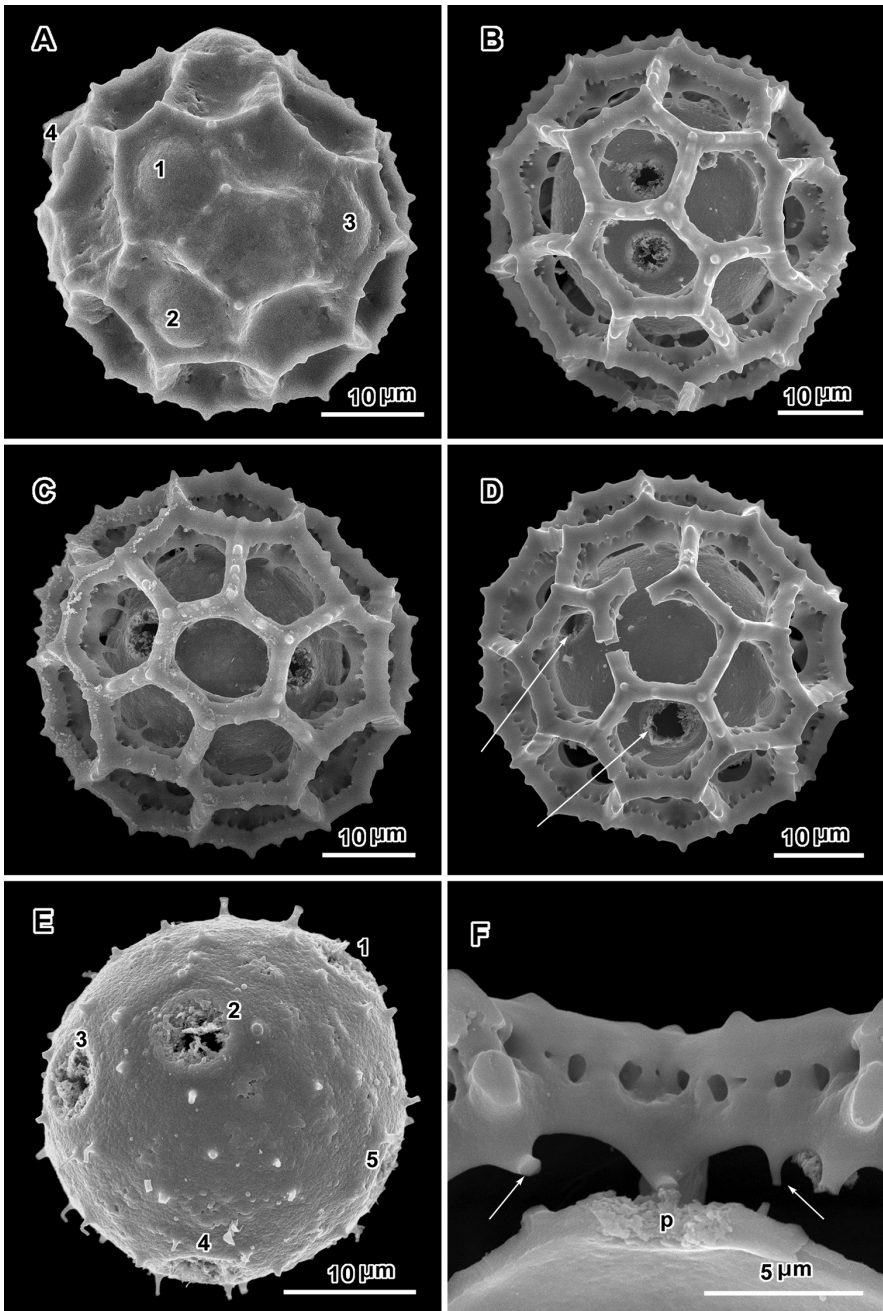
Figure 18. Scanning electron micrographs of Oocephala staebelinoides (Harv.) H. Rob. & Skvarla. A Unacetylated grain showing three pores with caps intact, two pores in adjacent lacunae B–D Intact or nearly intact grains showing pores in both pentagonal and hexagonal lacunae B with pores in adjacent lacunae E Grain stripped of muri showing five pores and stubs of muri attachments F Segment of muri showing rhizomate structure and remnants of weak basal attachments to footlayer, (p) pore. A–F are from collection of Liebenberg 8843.
