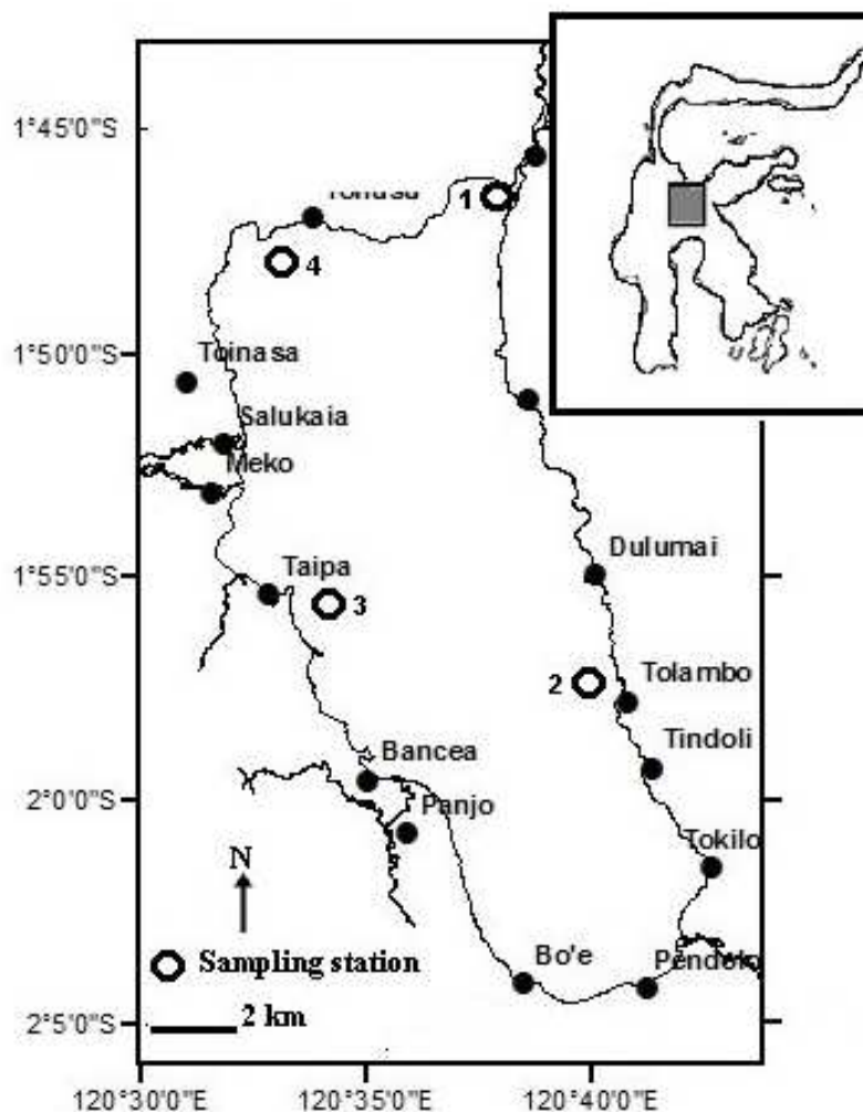
Figure 2. Map of the Lake Poso Study Site and Sampling Stations
