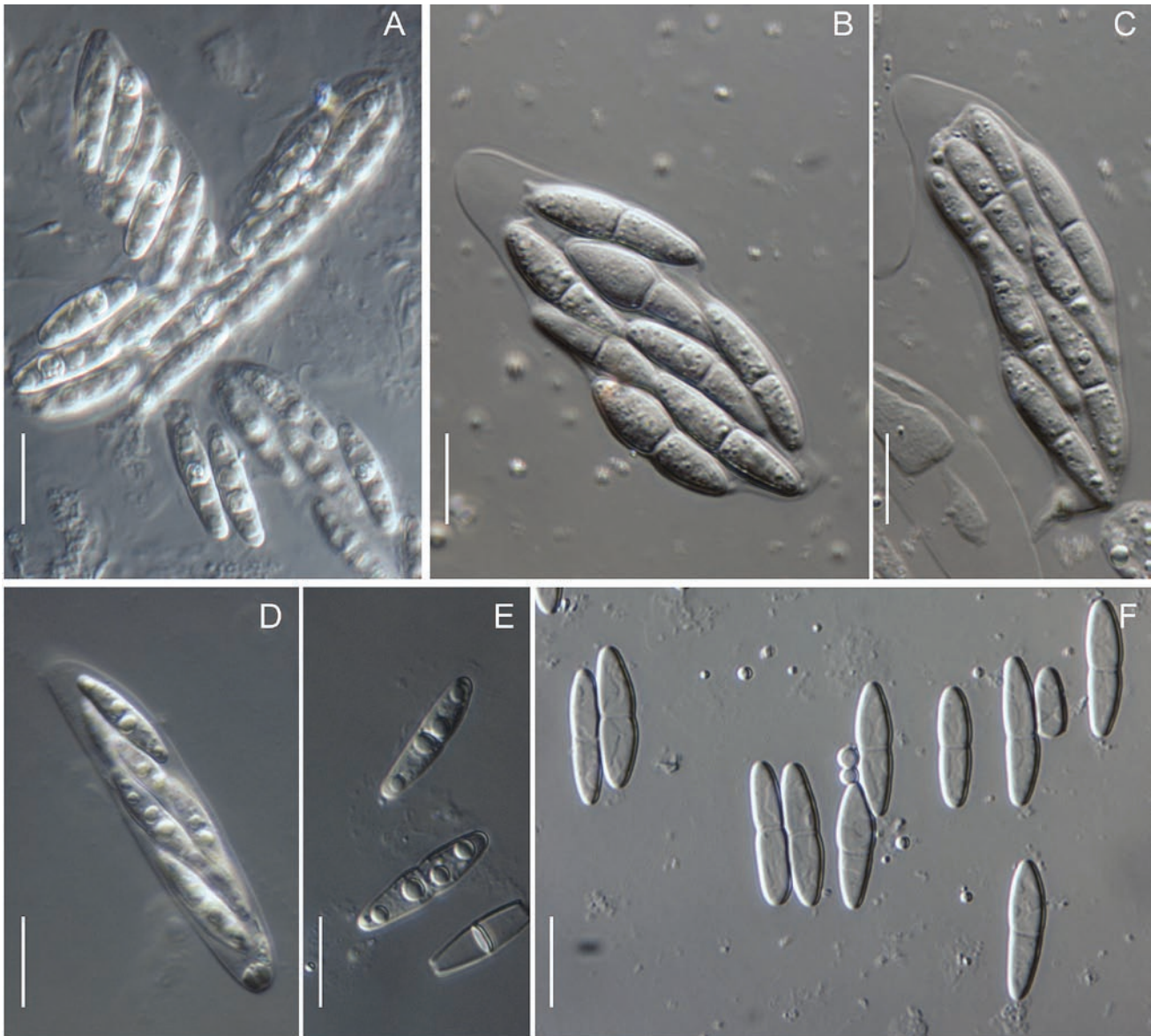
Fig. 44. Morphology on natural substrates, asci and ascospores. A. Plagiostoma euphorbiae , lectotype Fungi Rhenani 863, BPI bound. B, C. P. aesculi , epitype BPI 748430. D–F. P. barriae , holotype BPI 877717B. Scale 10 \mu\text{m} .
