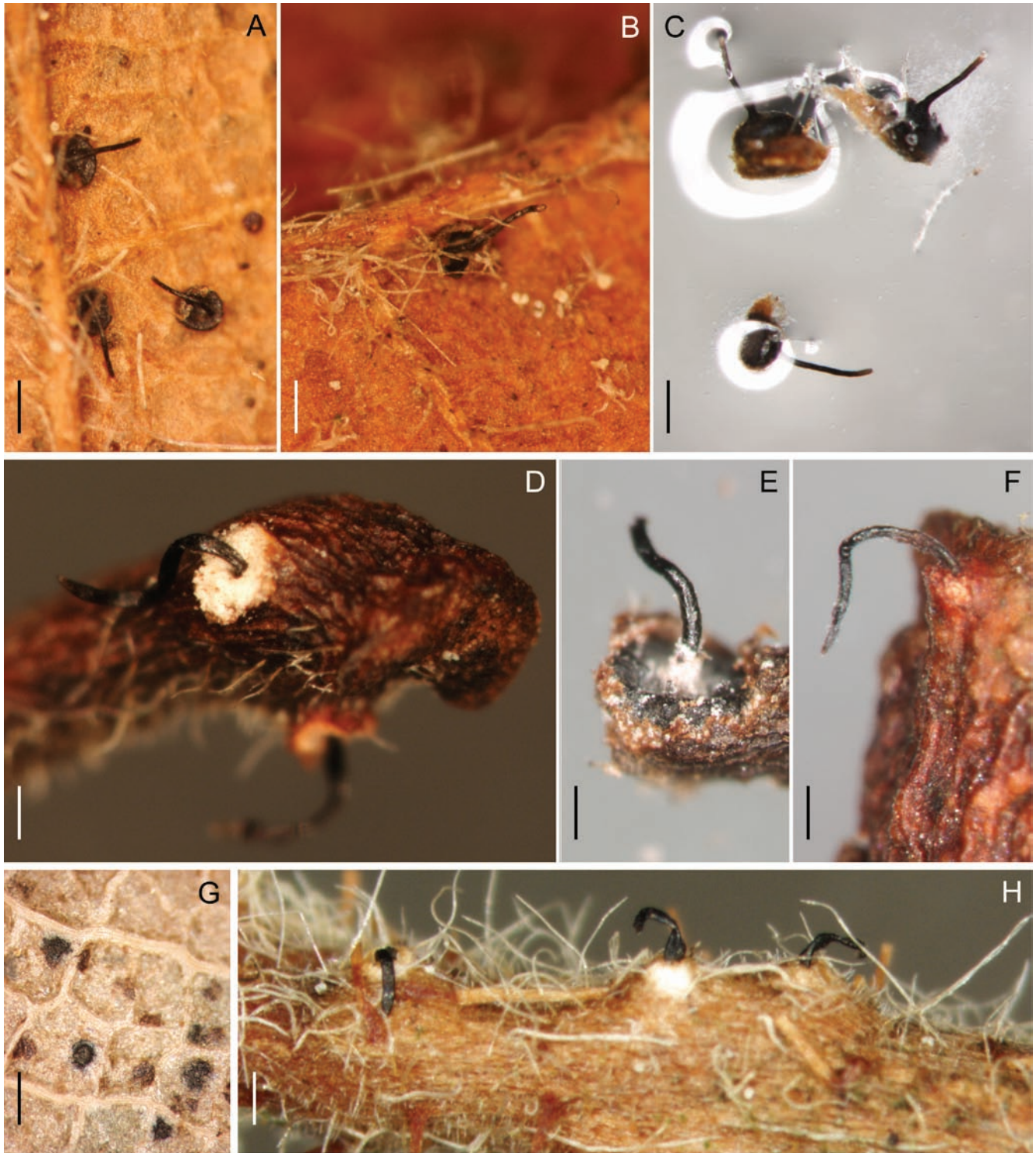
Fig. 12. Morphology on natural substrate, perithecia. A–C. Gnomonia virginiana . A. BPI 878210. B. BPI 877565A. C. BPI 878209. D–F. G. amoena . D, E. BPI 877469. F. BPI 877468. G. G. arnstadiensis , BPI 877470. H. G. pseudoamoena , BPI 877516. A, B, D, F–H. Intact air-dry perithecia on leaves and petioles. C. Extracted and rehydrated perithecia. E. Air-dry perithecium on fragment of petiole with removed outer tissue. Scale 200 µm.
