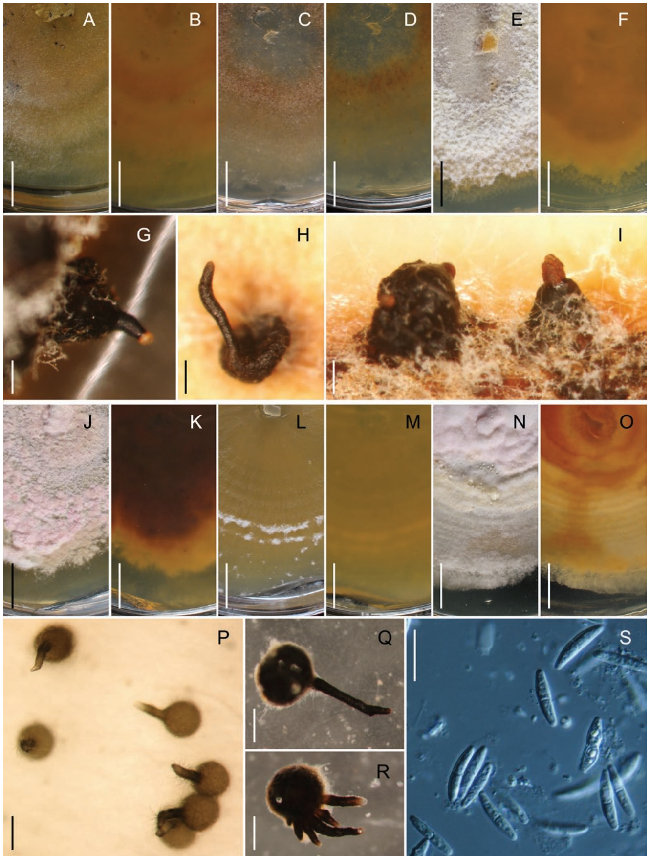
Fig. 33. Culture morphology. A–I. Ophiognomonium vasiljevae ex-type CBS 121253. J–S. O. cf. alni-viridis CBS 121250. A–F, J–O. Colony habit, 40 d, 23 °C. A, C, E, J, L, N. Surface. B, D, F, K, M, O. Reverse. G–I. Sterile perithecia or perithecium-like bodies, 2/10 °C. P. Young perithecia, 2/10 °C. Q, R. Perithecia, 2/10 °C. G, H, Q, R. 4.5 mo. I. 8 mo. P. 40 d. A, B, G, H, Q–S. PDA. C, D, I, P. MEA. E, F. MYA. G, H, Q–S. Scale: A–F, J–O. 1 cm. G–I, P–R. 200 \mu m. S. 10 \mu m.
