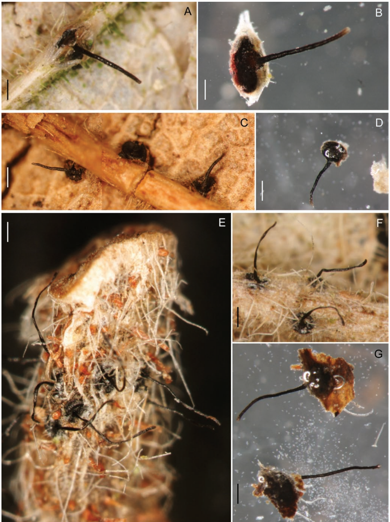
Fig. 9. Morphology on natural substrate, perithecia. A, B. Gnomonia pendulorum , holotype BPI 877526B. C, D. G. rodmanii , holotype BPI 878211A. E–G. G. skokomishica . E, G. Holotype BPI 877465B. F. BPI 877535. A, C, E, F. Intact air-dry perithecia on leaves. B, D, G. Extracted and rehydrated perithecia. Scale 200 \mu m.
