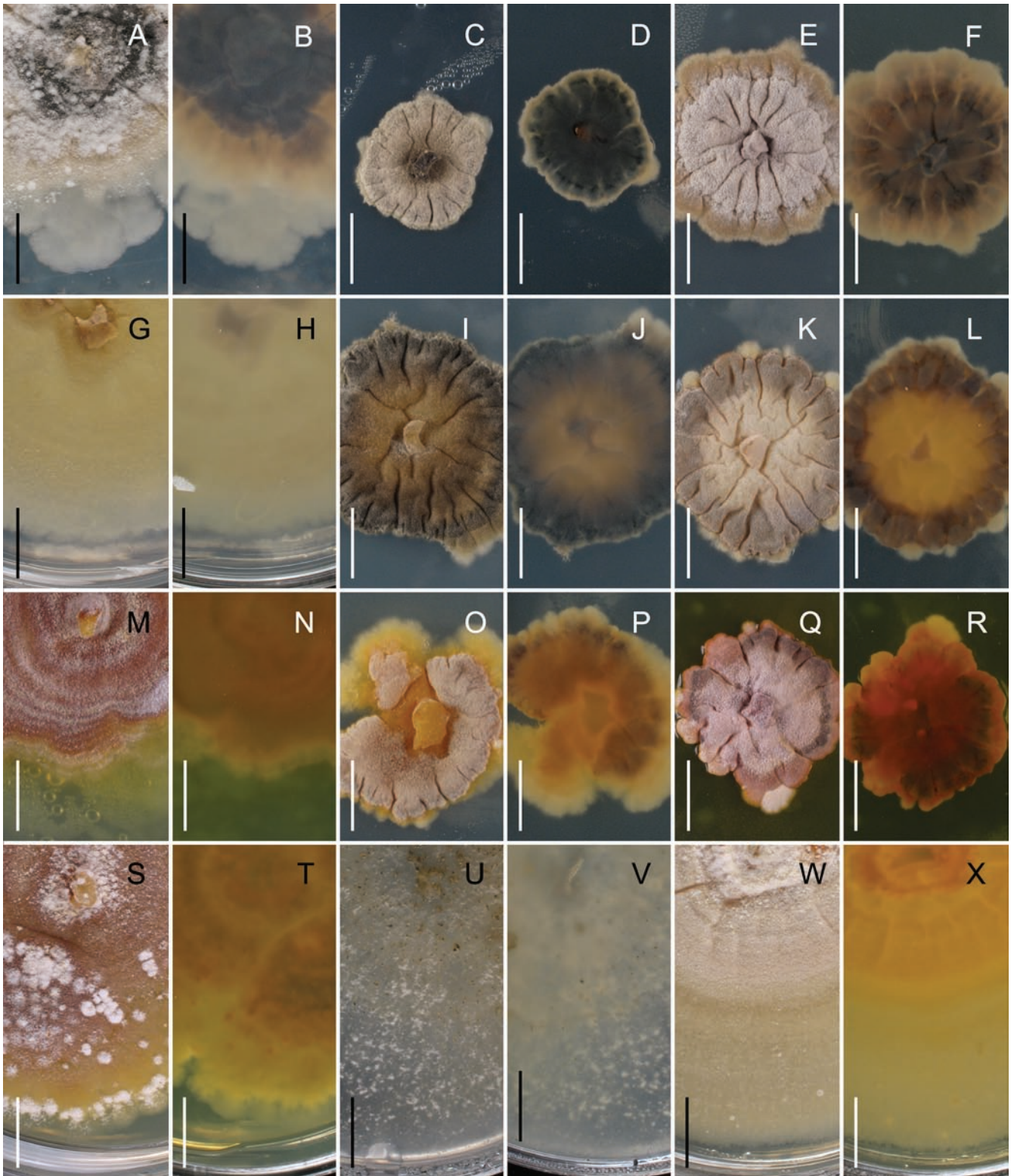
Fig. 42. Ophiognomonia setacea , culture morphology, colony habit, 40 d, 23 °C. A–F. CBS 116406. G–L. CBS CBS116408. M–P. CBS 121235. Q, R. CBS 121237. S–X. O. cf. setacea CBS 121256. A, C, E, G, I, K, M, O, Q, S, U, W. Surface. B, D, F, H, J, L, N, P, R, T, V, X. Reverse. Scale 1 cm.
