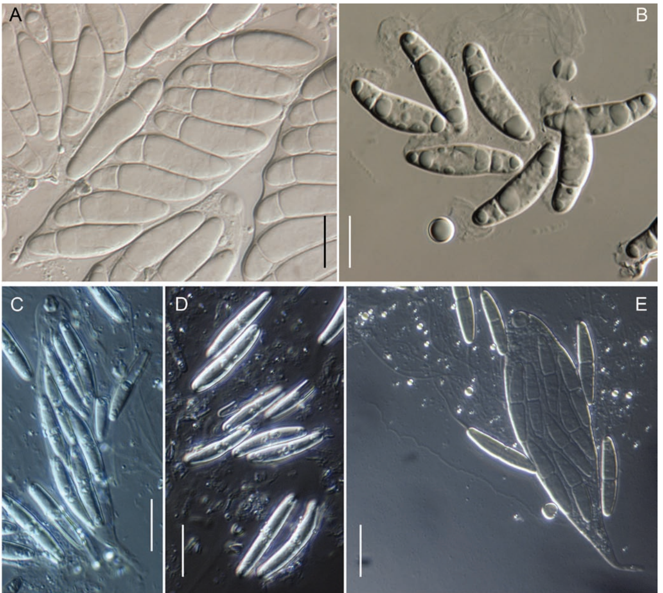
Fig. 19. Morphology on natural substrate, asci and ascospores. A, B. Apiognomonia acerina , BPI 877677. C–E. A. hystrix . C. BPI 877697. D. BPI 877698. E. BPI 877692. Scale 10 \mu m.
