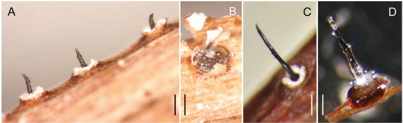
Fig. 15. Morphology on natural substrate, perithecia. Ambarignomonium petiolorum . A, B. Epitype BPI 844274. C, D. BPI 877511. A, C. Intact air-dry perithecia on petioles. B. Air-dry perithecium on fragment of petiole with removed outer tissue. D. Extracted and rehydrated perithecia. Scale 200 \mu m.
