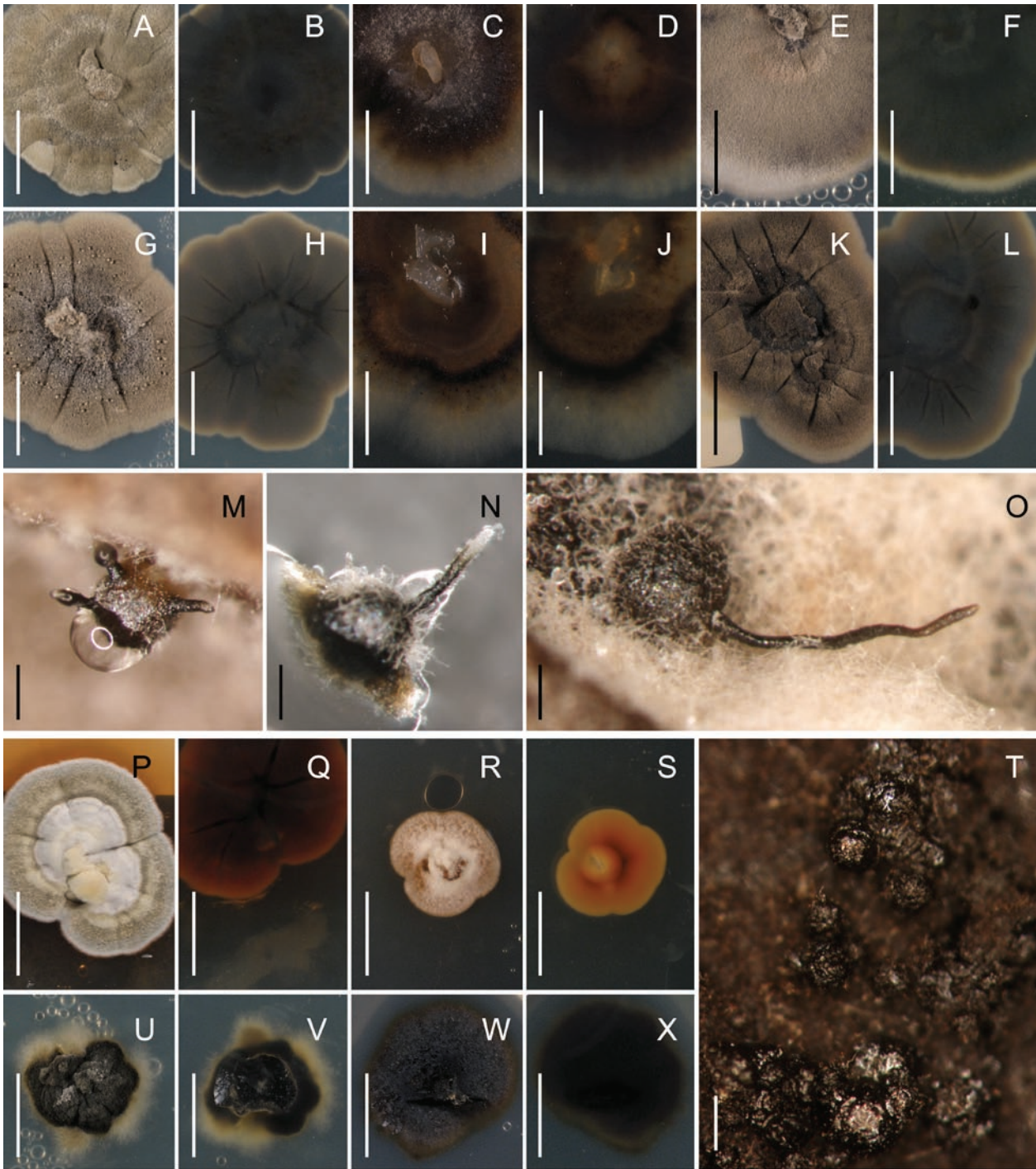
Fig. 7. Culture morphology. A–O. Gnomonia neognomon . A–F. CBS 121244. G–L. CBS 121265. M–O. Ex-type CBS 121246. P–X. G. orcispora . P–S. AR 4286. T–X. CBS 121247. A–L, P–S, U–X. Colony habit, 40 d, 23 °C. A, C, E, G, I, K, P, R, U, W. Surface. B, D, F, H, J, L, Q, S, U, X. Reverse. M–O, T. Perithecia, 2/10 °C. M, N, T. 4.5 mo. O. 8 mo. A, B, G, H, P, Q, U, V. PDA. C, D, I, J, N, R, S, W, X. MEA. E, F, K–M, O, T. MYA. Scale: A–L, P–S, U–X. 1 cm. M–O, T. 200 \mu m.
