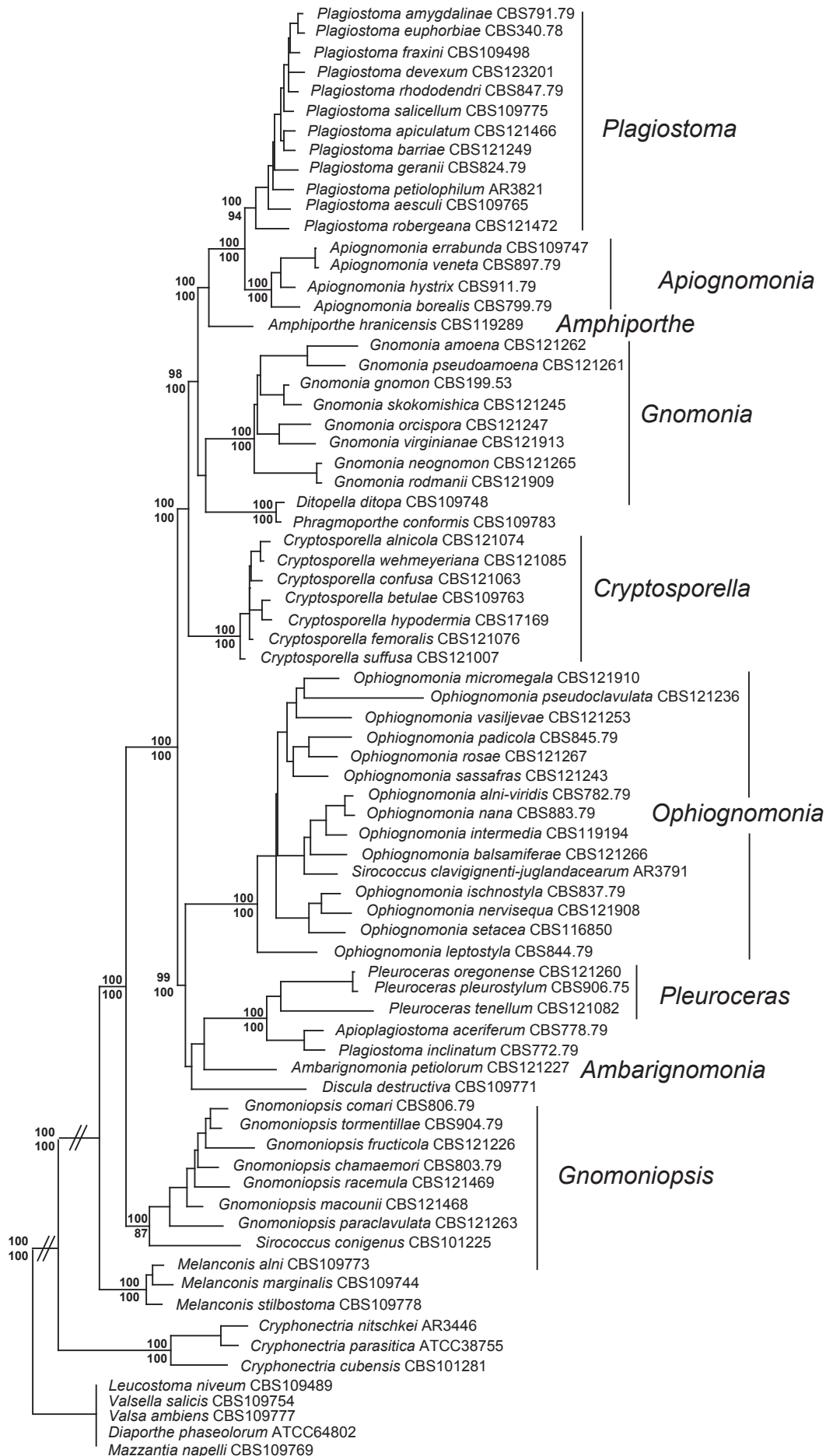
Fig. 1. ML phylogenetic analysis (ML score = -lnL 26702.18832) of sequences for the tef1- \alpha , nrlSU and rpb2 multigene analysis of genera in the Gnomoniaceae for 64 gnomoniaceous taxa and 11 outgroup diaporthean taxa. Bayesian posterior probabilities greater than 95 % are shown above each branch. MP bootstrap values greater than 70 % are shown below each branch.
