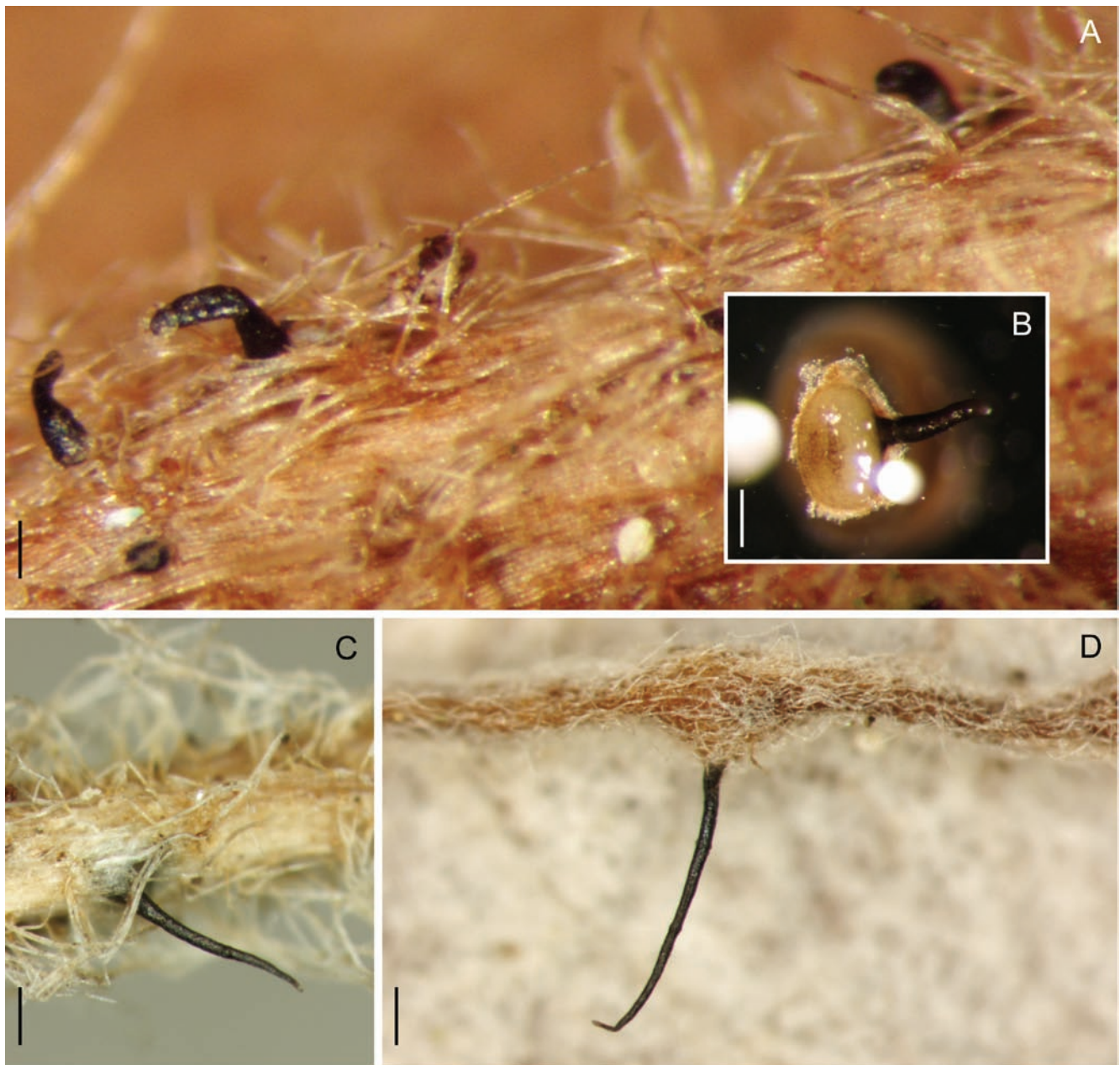
Fig. 37. Morphology on natural substrates, perithecia. A, B. Ophiognomonia micromegala . A. BPI 877613A. B. BPI 877634B. C. O. rosae , BPI 877586. D. O. rubi-idaei , BPI 877637. A, C, D. Intact air-dry perithecia on leaves. B. Extracted and rehydrated perithecium. Scale 200 \mu m.
