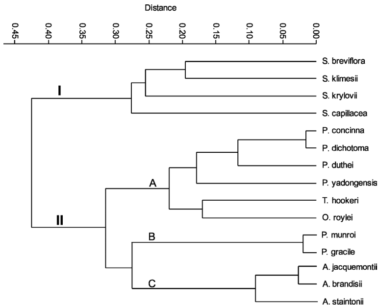
Figure 2. Cluster analysis (UPGMA method of classification and Gower's general similarity coefficient) performed on 16 qualitative morphological characters for all of the Nepalese members from the tribe Stipeae.
