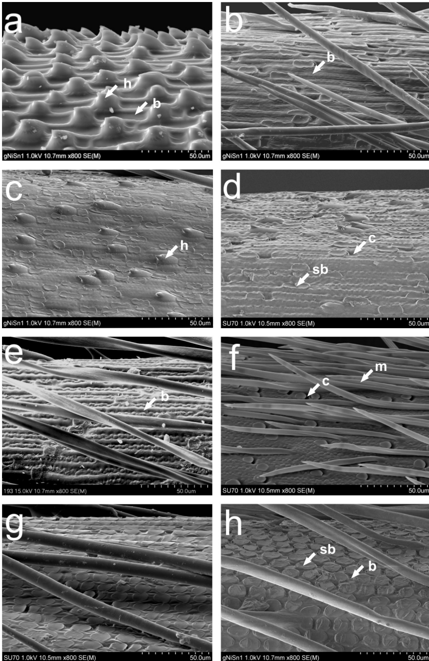
Figure 3. Lemma epidermal patterns (LEPs) of Old World Stipeae: a Stipa breviflora [Kyrgyzstan, near Issyk-Kul Lake, M. Nobis (KRA)] b Ptilagrostis concinna [India, Ladakh, Himalayas, L. Klimeš (KRA)] c Ptilagrostis duthiei [India, Himalayas, J.F. Duthie 3585 (LE)] d Orthoraphium roylei [India, Himalayas, J.F. Duthie 3568 (LE)] e Trikeriaia hookeri [China, Tibet (PE 718306)] f Piptatherum munroi [Nepal, Solukhumbu, M.F. Watson et al. DNEP3 AX33 (E)] g Achnatherum brandisii [India, Kashmir, R.R. Stewart 18120 (NY)] h Achnatherum staintonii [Nepal, Mustang, M.A. Farille 81-340 (E)]. Annotations: b – basal cells, c – cork cells, sb – silica bodies, m – macro-hairs.
