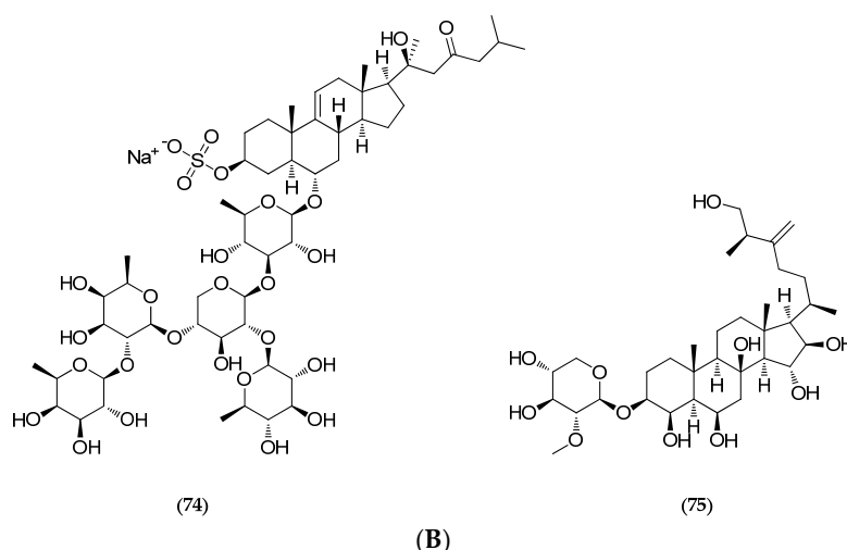
Figure 18. (A) Thromidia catalai . © IRD; (B) Structure of thornasteroside A (72), ophidianside F (73), regularoside B (74) and thromdioside (75).
