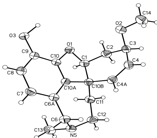
Figure 2. Crystal structure of chlidanthine ( 1 ).
