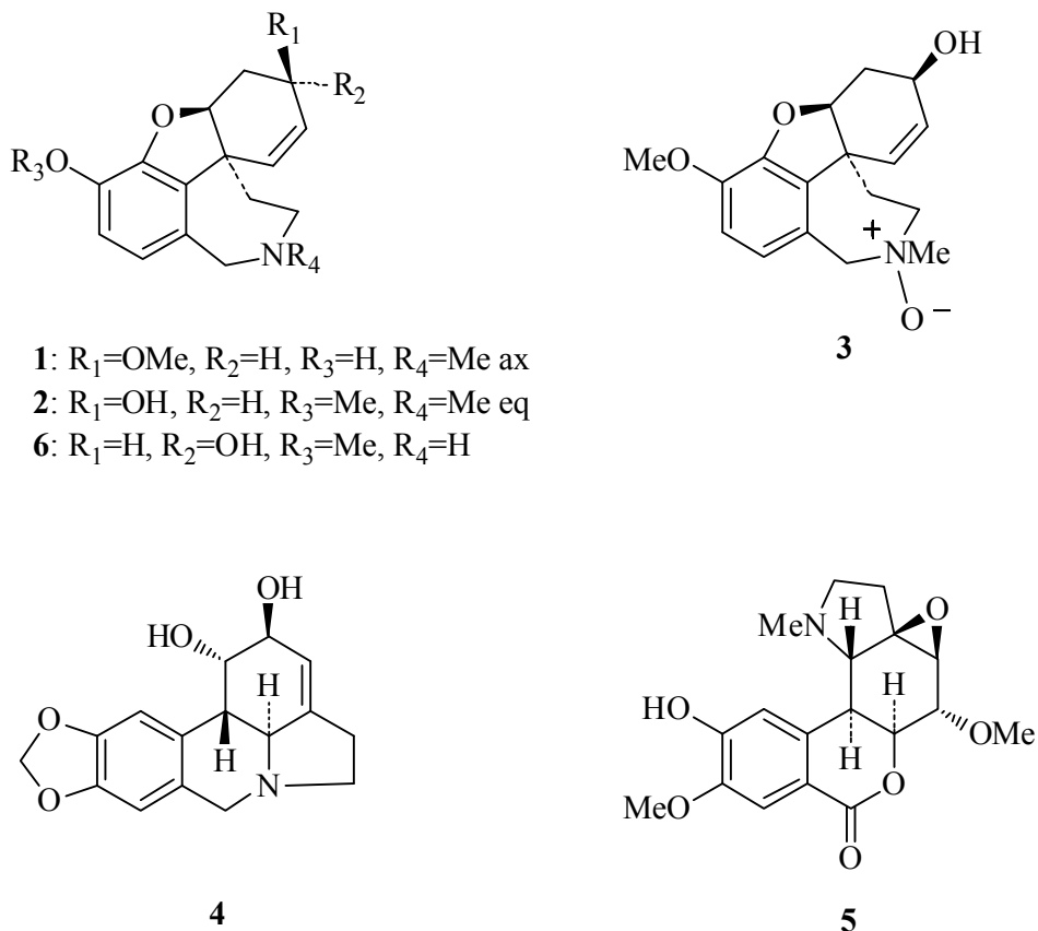
Figure 1. Alkaloids isolated from Zephyranthes concolor .
