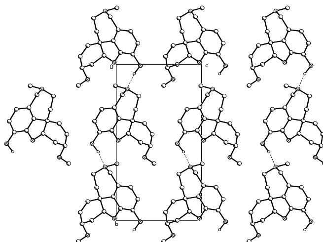
Figure 3. Crystal packing of chlidanthine ( 1 ) shows intermolecular hydrogen bonding.
