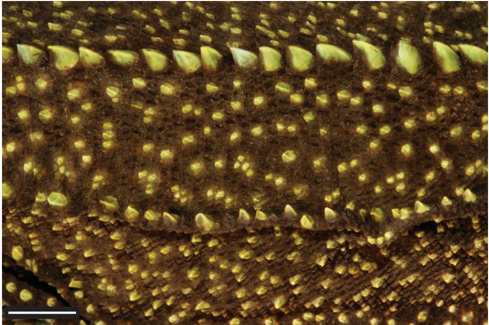
Figure 7. Close-up of left dorsum of Enyalioides anisolepis (QCAZ 12537, holotype) showing scattered enlarged scales. Scale bar = 5 mm. Photograph by Omar Torres-Carvajal.
