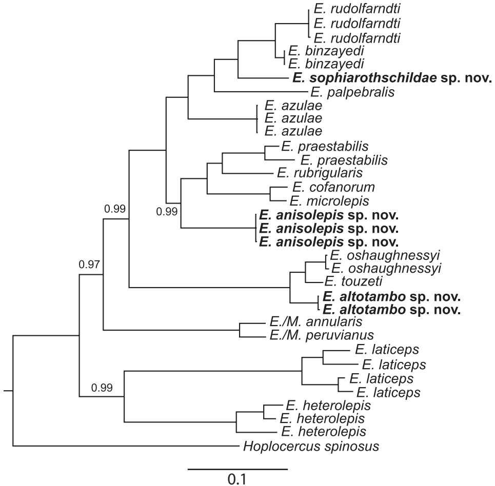
Figure 9. 50% Majority rule consensus tree of hoplocercine lizards ( E. = Enyalioides , M. = Morunasaurus ) based on a Bayesian analysis of mtDNA sequences. Posterior probabilities are equal to 1, unless otherwise noted by numbers next to branches. Outgroup taxa are not shown. The notation E./M. indicates that according to the phylogenetic definitions (de Queiroz and Gauthier 1990) of the names Enyalioides and Morunasaurus proposed by Torres-Carvajal et al. (2011), Morunasaurus is a subclade of Enyalioides .
