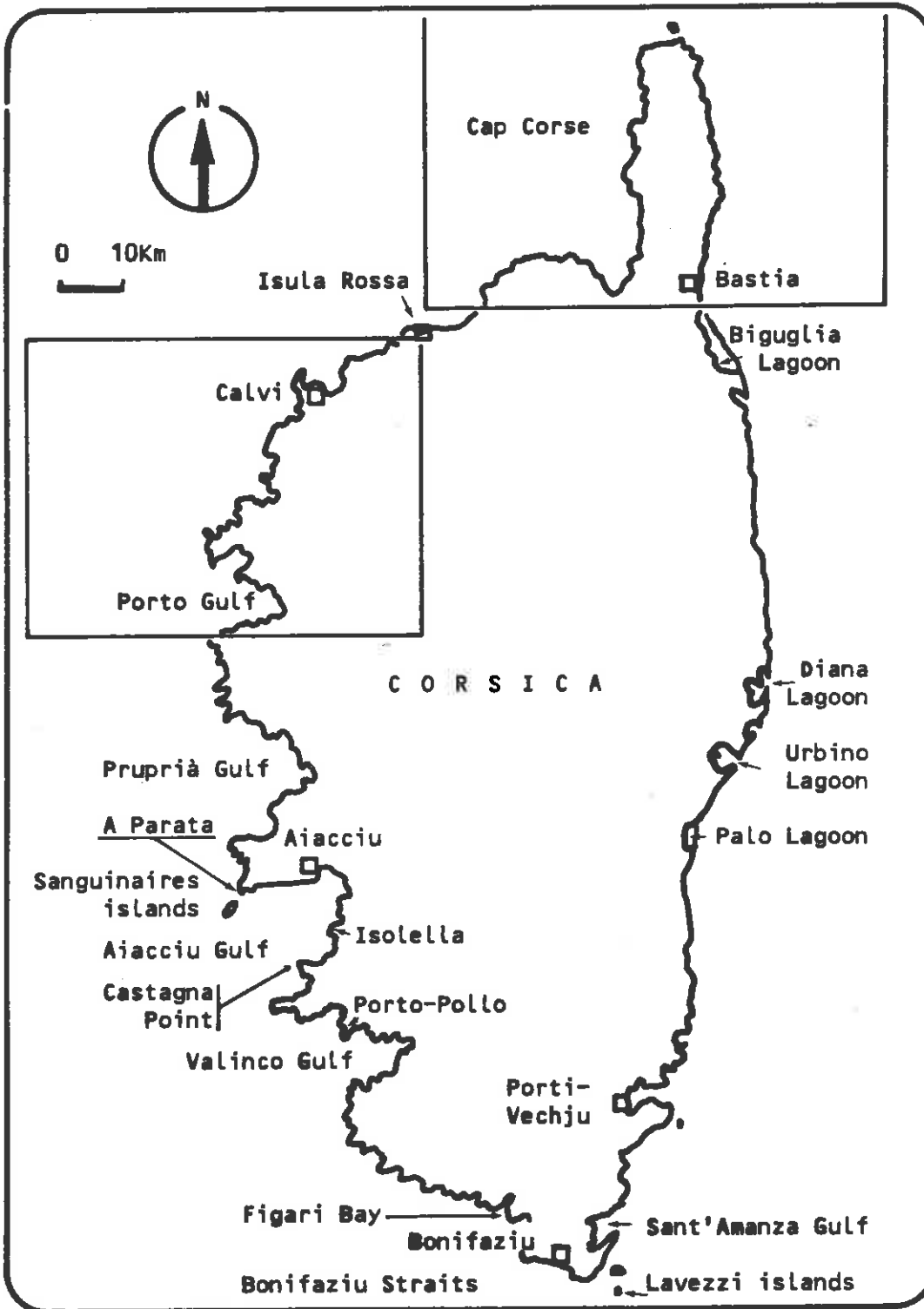
Fig. 1 : Map of Corsica. See Fig. 2 for details.
