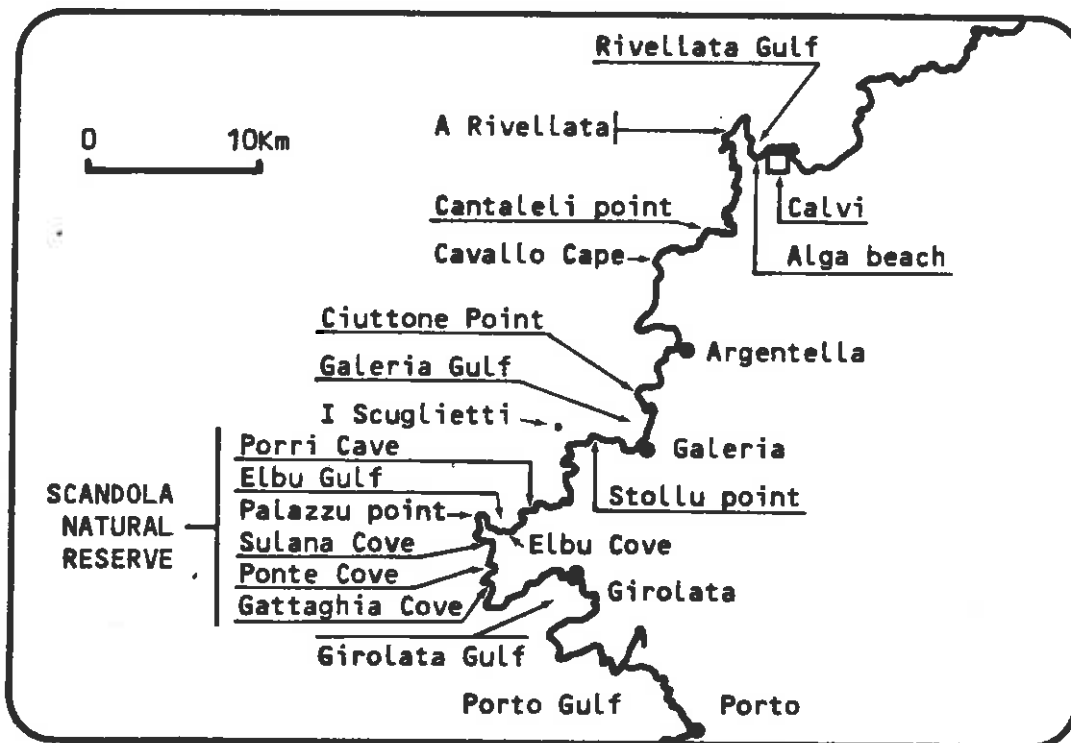
Fig. 2 : Details of Cap Corse (above) and of the West coast, between Calvi and Porto gulf (below).
