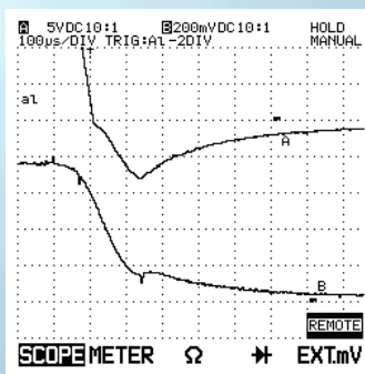
Figure 16: Inductive Load Shutdown - Current Decay (RY150B shown) Top Trace: Output Voltage Bottom Trace: Output Current (200 A/div)
