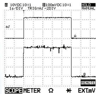
Figure 14: Overcurrent Level 2 Shutdown (RY150B shown) Top Trace: Output Voltage Bottom Trace: Output Current (100 A/div)
