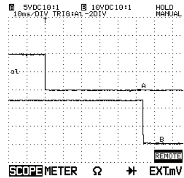
Figure 4: RYxxxB Turn-Off Time Top Trace: Trigger Voltage Bottom Trace: Output Voltage
