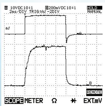
Figure 15: Short Circuit Shutdown (RY150B shown) Top Trace: Output Voltage Bottom Trace: Output Current (200 A/div)
