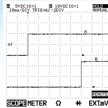
Figure 2: RYxxxB Turn-On Time Top Trace: Trigger Voltage Bottom Trace: Output Voltage
