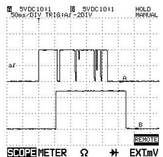
Figure 11: RYxxxA Trigger Noise Immunity Top Trace: Trigger Voltage Bottom Trace: Output Voltage
