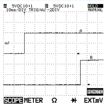
Figure 1: RYxxxA Turn-On Time Top Trace: Trigger Voltage Bottom Trace: Output Voltage
