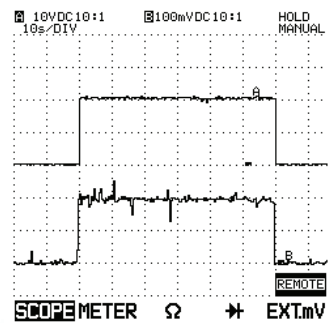
Figure 13: Overcurrent Level 1 Shutdown (RY150B shown) Top Trace: Output Voltage Bottom Trace: Output Current (100 A/div)
