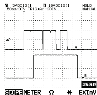
Figure 12: RYxxxB Trigger Noise Immunity Top Trace: Trigger Voltage Bottom Trace: Output Voltage
