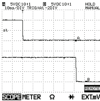
Figure 3: RYxxxA Turn-Off Time Top Trace: Trigger Voltage Bottom Trace: Output Voltage
