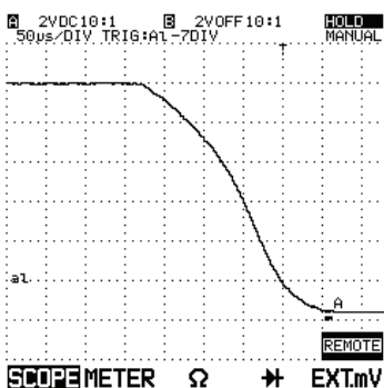
Figure 7: RYxxxA Output Fall Time
