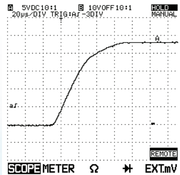
Figure 6: RYxxxB Output Rise Time
