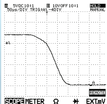
Figure 8: RYxxxB Output Fall Time
