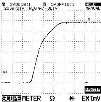
Figure 5: RYxxxA Output Rise Time
