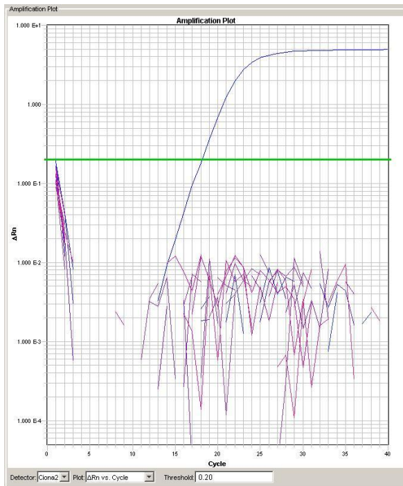
Figure 6: Amplification plot for C. intestinalis qPCR assay. Amplified product is C. intestinalis gDNA.
