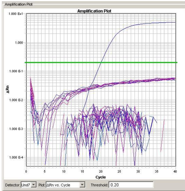
Figure 7: Amplification plot for U. pinnatifida qPCR assay. Amplified product is U. pinnatifida gDNA.
