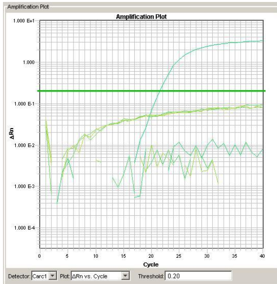
Figure 5: Amplification plot for C. maenas qPCR assay. Amplified product is C. maenas gDNA.
