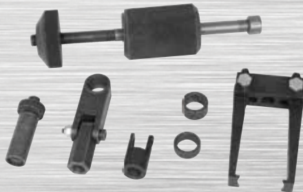
DIESEL INJECTOR PULLER KIT Part # 40740 - $269.95
