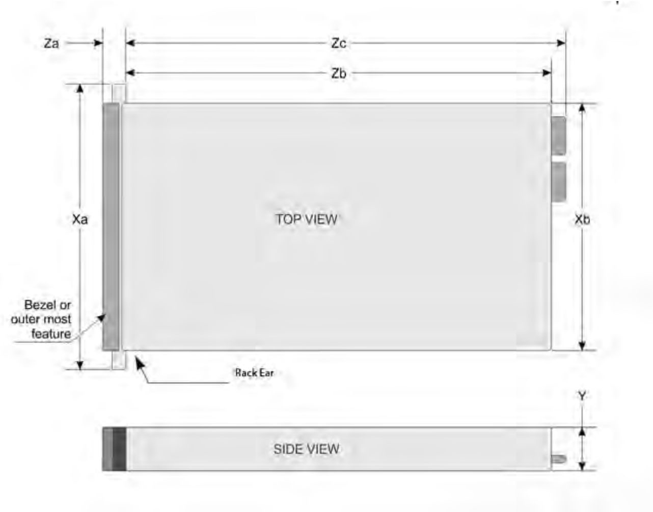
Figure 27. Chassis Dimensions for R740 and R740xd
