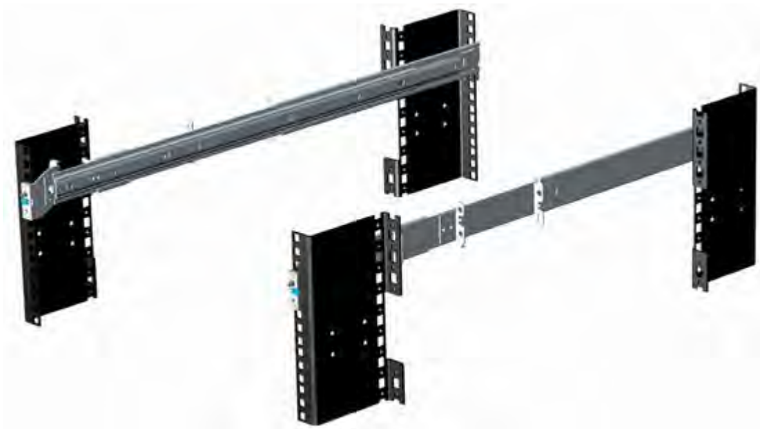
Figure 15. Static rails
