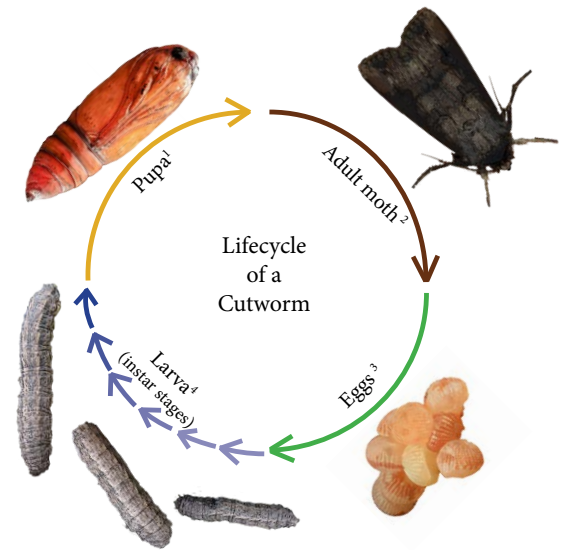
Cutworm lifecycle
