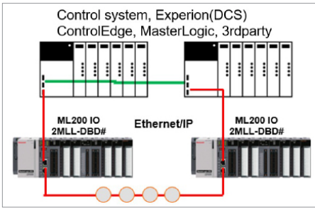
Figure 1: Ring Topology
