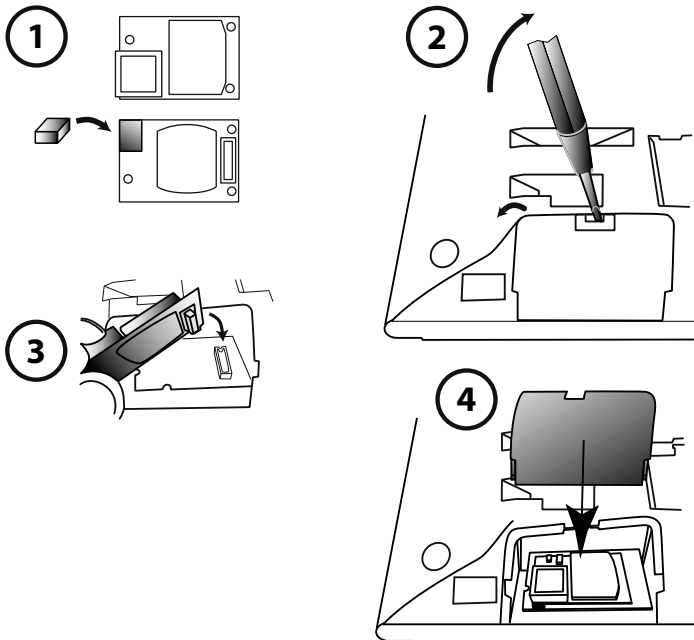
Fig. 64 Montage Bluetooth-Modul
