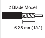
Quick strips RG59/RG6/RG7/RG11
