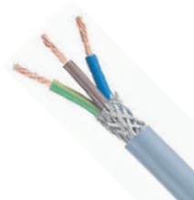
363-395 Belden 3 Core Screened CY Control Cable, 2.5 mm 2 CSA CYSE03.0050
