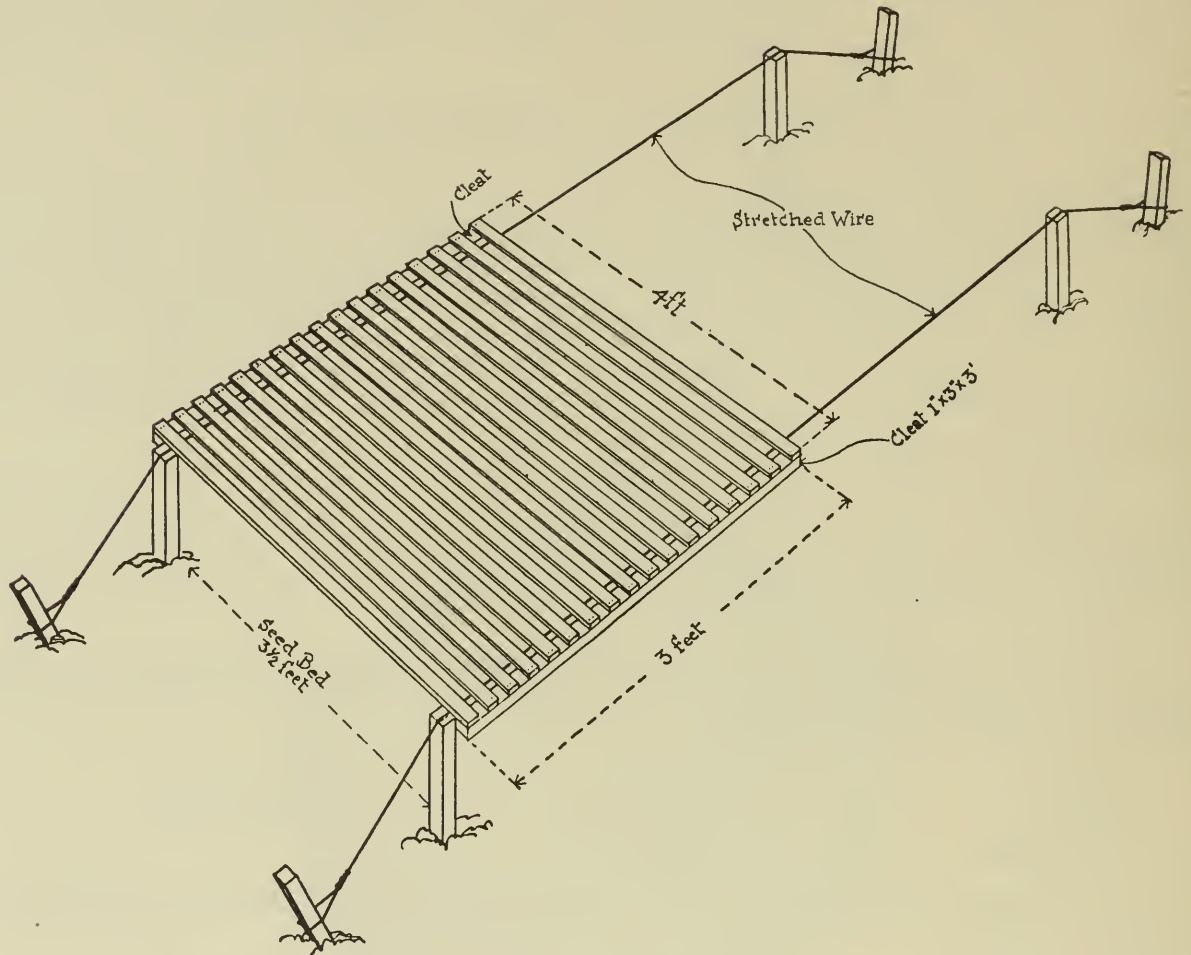
Method of supporting lath shade over seed-bed.
