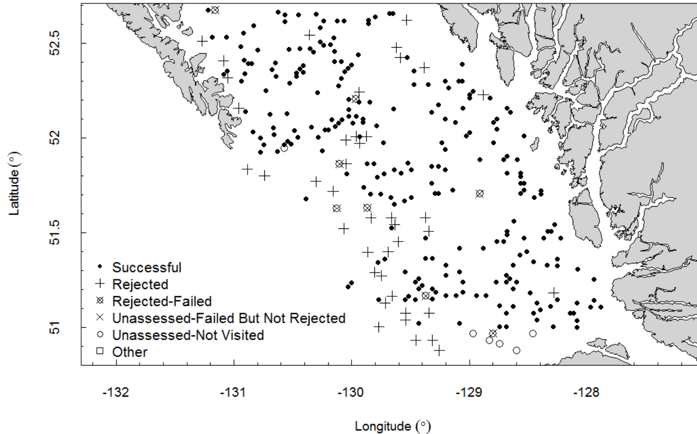
Figure 10. Final status of the 2015 QCS synoptic bottom trawl survey showing 240 successfully fished blocks (Successful), 41 blocks rejected after inspection or based on prior knowledge (Rejected), 8 blocks rejected after one or more failed fishing attempts (Rejected-Failed) and six blocks that were not visited and remain in the sampling frame (Unassessed-Not Visited).
