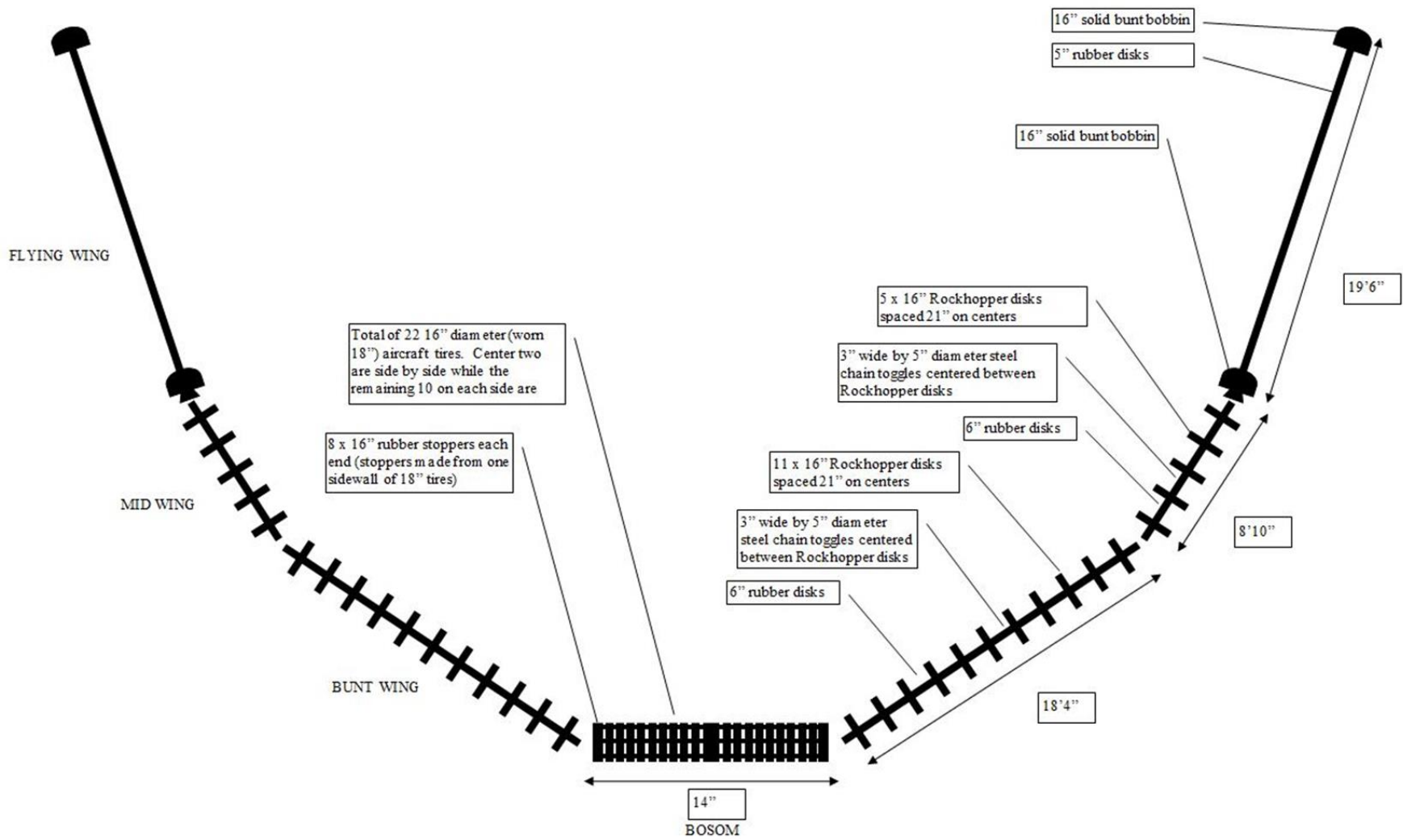
Figure 9. Details of the Rockhopper foot gear for the Atlantic Western Ila box trawl used on the 2015 QCS synoptic bottom trawl.
