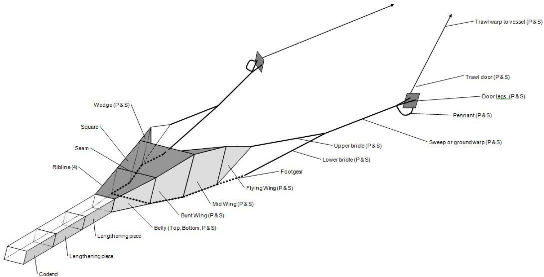
Figure 4. Overview diagram of the Atlantic Western IIA box trawl used on the 2015 QCS synoptic bottom trawl survey.
