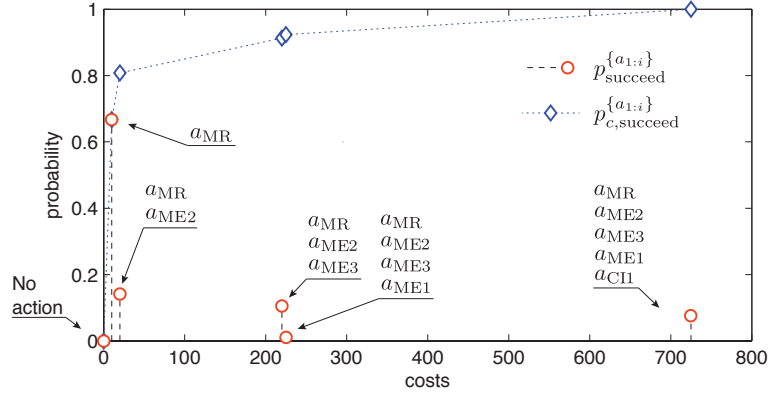
Figure 5: Probability mass function p_{\text{succeed}}^{\{a_{1:i}\}} and cumulative probability p_{c,\text{succeed}}^{\{a_{1:i}\}} for the costs of the optimized sequence of actions.
