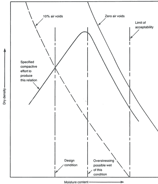
Figure 1. Principle of the method specification for the compaction of well-graded soils (from Parsons 1992).
