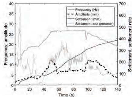
Figure 4. The vibrator and results from one compaction test.
