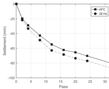
Figure 3. Settlement of the embankment surface.
