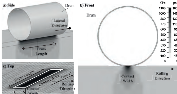
Figure 5. Finite Element Modelling of Roller-Soil Interaction
