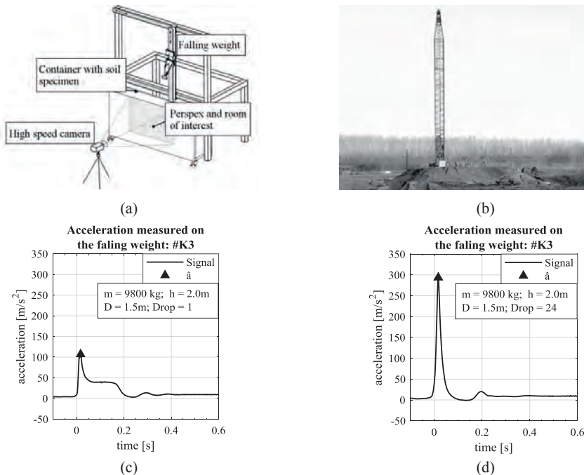
Figure 1. The experimental setup for the laboratory investigation with the PIV/DIC Method (a). A picture of the test site with the crawler crane just before the investigation took place (b). The acceleration measured on the falling weight in vertical direction after the first (c) and the 24 th impact (d).
