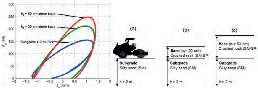
Figure 2. Field measured F_c - z_d loops from IC roller on vertically homogeneous subgrade soil
