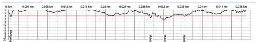
Figure 4. Planograf AX02: longitudinal profile, with comments, red limit line at 4 mm
