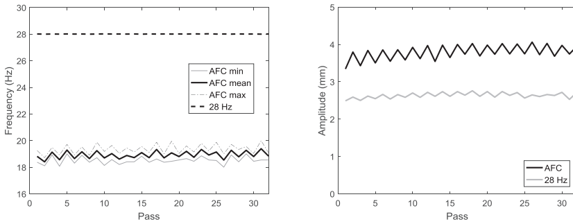
Figure 2. Compaction frequency (left) and displacement amplitude (right).
