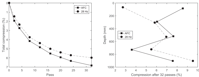
Figure 4. Total compression (left) and compression profile after 32 passes (right) from EMU sensors.
