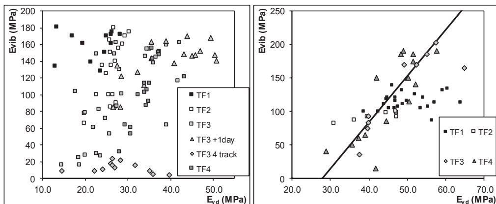
Figure 1. Results from test fields at Dolga vas (left) and PSP Avče (right).
