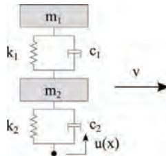
Figure 2. Vehicle model consisting of a two mass spring-dashpot-system.
