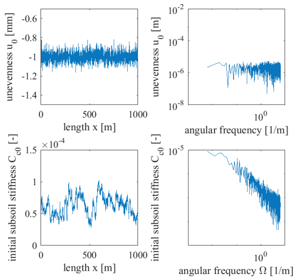
Figure 1. Unevenness u_0 and subsoil stiffness C_{c0} in initial state (left) and as a function of angular frequency (right).
