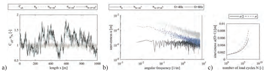
Figure 3. a) Longterm-unevenness approaching the initial soil stiffness (scaled). b) Unevenness u as a function of angular frequency for different load cycles. c) Unevenness u as a function of load cycles N ( \Omega=1 ) varying the initial compaction of the soil foundation in terms of the variance.
