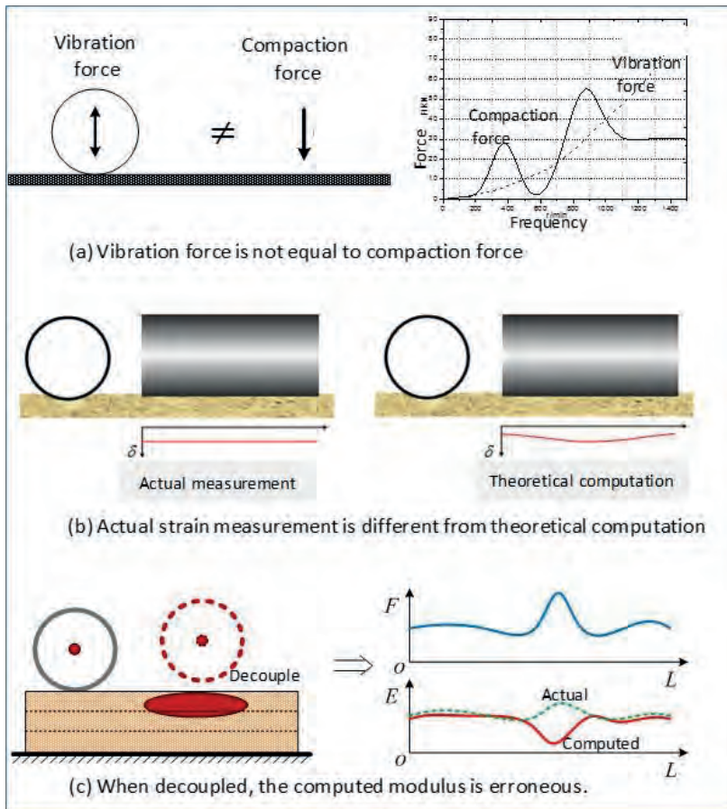
Figure 1. Main challenges to compute ICMV.
