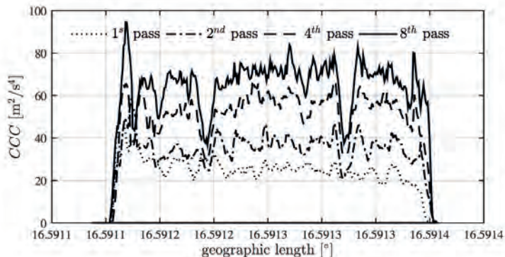
Figure 4. Progress of the measured CCC values of the passes 1, 2, 4 and 8 on lane 2 of layer 2 of the test field (Pistor 2016).
