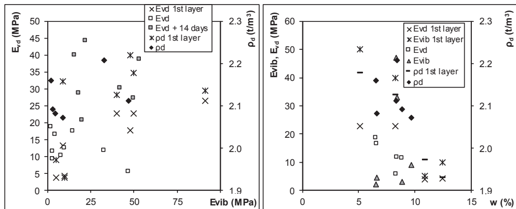
Figure 2. Field test results at test filed for HPP Brežice temporary dikes.
