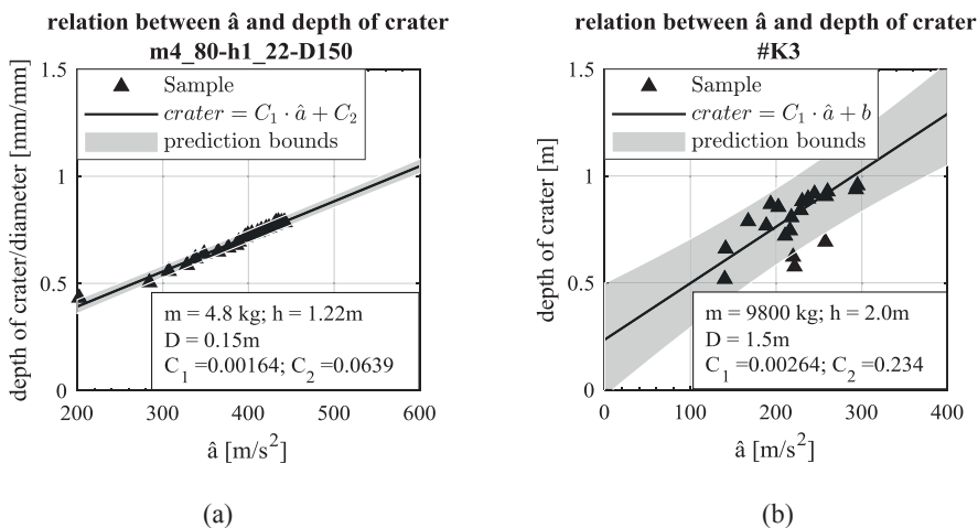
Figure 3. The maximum value of acceleration is in linear relationship with the depth of the crater in laboratory (a) and field condition (b).
