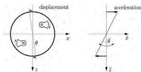
Figure 1. Excitation of an oscillatory drum.
