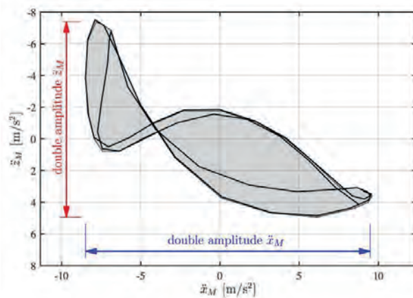
Figure 3. Horizontal and vertical accelerations in the bearing of the oscillatory drum for two periods of excitation during the eleventh pass on lane 2 of the test field (Pistor 2016).
