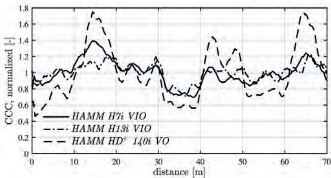
Figure 5. Validation of the CCC system exemplary for three oscillating rollers (Pistrol 2016).
