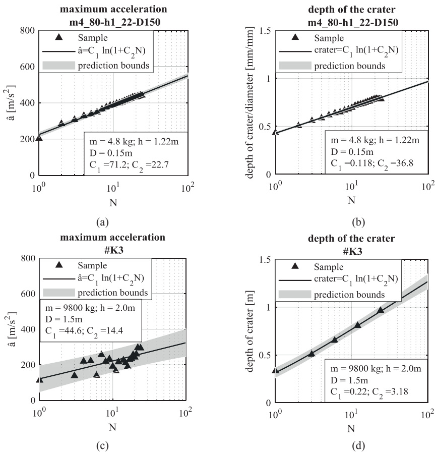
Figure 2. The results of the laboratory investigation (a-b) and the field investigation (c-d)
