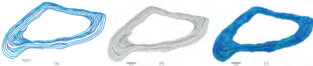
Figure 2. (a) Colour-coded CDCC values along several measuring tracks; (b) triangulation of the measurement points in order to define the grey shaded inspection lot; (c) interpolation of the measurements from (a) at equidistantly distributed reference points
