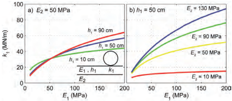
Figure 5. Model-simulated k vs E_1 for a two-layer system for: (a) variable h_1 , (b) variable E_2
