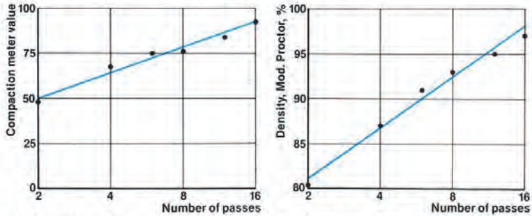
5.1. Correlation between the values recorded by the compaction meter and the number of passes.
