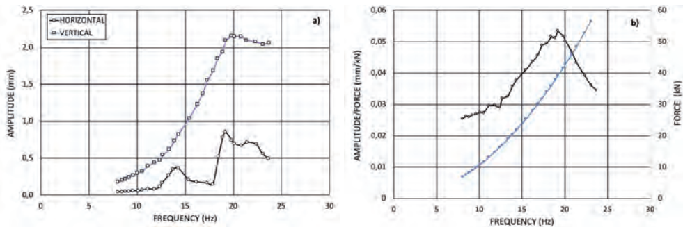
Figure 1. Effect of vibrator frequency on vertical displacement, data from Converse (1952). Influence of frequency on peak-to-peak amplitude. a) vibration amplitude as function of frequency, b) normalized vibration amplitude and centrifugal force.
