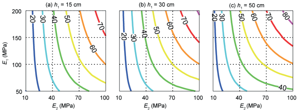
Figure 4. Simulated k values (MN/m) for (a) h_1 = 15 cm (b) h_1 = 30 cm and (c) h_1 = 50 cm
