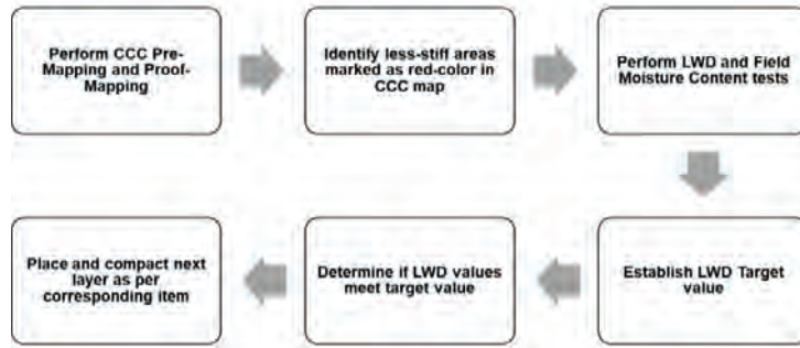
Figure 3. CCC Quality Management Process paired with Modulus-Based Spot Testing
