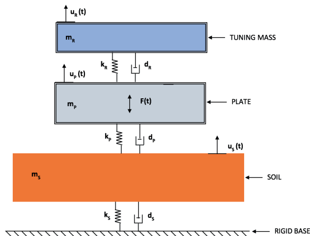
Figure 2. Theoretical model for optimization of vibratory plate compaction system.
