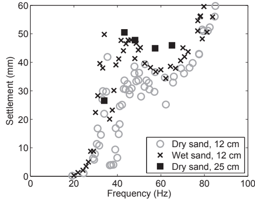
Figure 3. Frequency-dependent settlement/compaction in model tests, from Wersäll et al. (2015).
