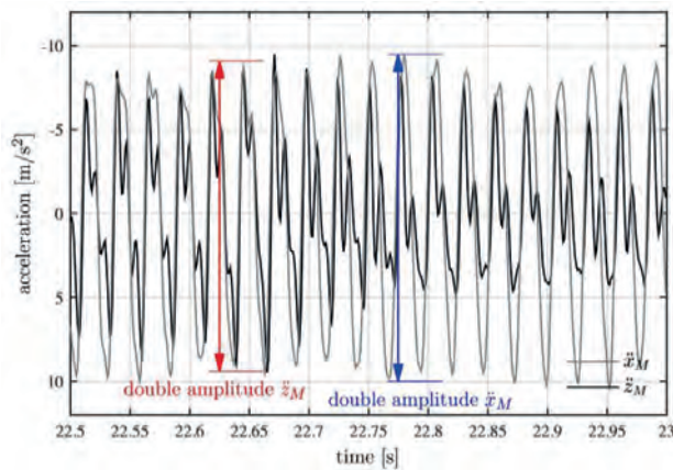
Figure 2. Horizontal and vertical accelerations in the bearing of the oscillatory drum for the eleventh pass on lane 2 of the test field (Pistor 2016).
