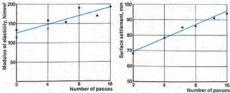
5.2. Correlation between the modulus of elasticity and the number of passes. ● dynamic modulus of elasticity determined by falling weight deflectometer ○ static modulus of elasticity determined by plate loading test.
