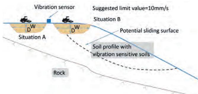
Figure 1. Zone subjected to strength degradation due to vibratory compaction. Vibration sensor location is tentative and has to be adapted to the specific project. The idea is to measure vibrations as close as possible to vibratory equipment and the potential sliding surface.
