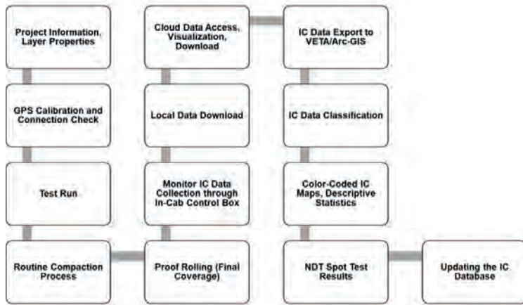
Figure 1. An Ideal Flowchart for Application of CCC in Quality Management
