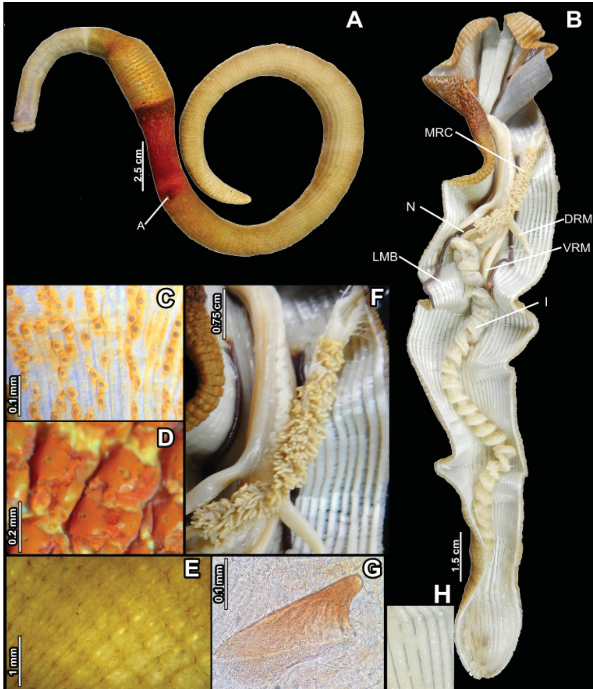
Fig. 4. Siponosoma cf. vastum (Selenka & Bülow in Selenka, 1883) from Oaxaca, Mexico. A. External morphology. B. Internal morphology. C. Introvert papillae. D. Posterior introvert papillae. E. Trunk wall from the median region of the trunk. F. Multiple rectal caeca. G. Hook. H. Longitudinal muscle bands. Abbreviations: A = anus; DRM = dorsal retractor muscles; I = intestine; LMB = longitudinal muscle bands; MRC = multiple rectal caeca; N = nephridium; VRM = ventral retractor muscles.
