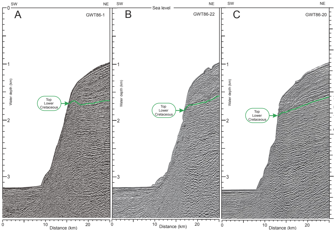
Figure 10. Seismic reflection lines GWT86-1, GWT86-22, and GWT86-20 (see Fig. 3 for location) show southeastward variation of escarpment height and profile and the position of the top of Lower Cretaceous strata. Escarpment height ranges from ~1.6 km (C) to ~1.9 km (A) along this segment. Vertical exaggeration is ~13:1 at seafloor.
