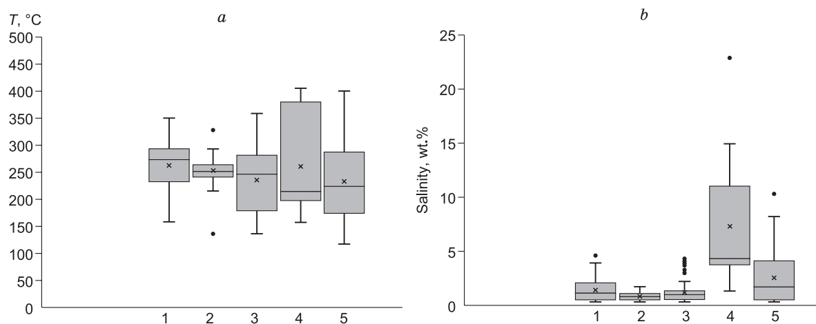
Fig. 11. Box plots of the homogenization temperatures (a) and fluid salinity (b) of inclusions in minerals of epithermal Au–Ag deposits in north-eastern Russia. Line inside the box is a median, cross is the average value, and points mark outliers. Regions: 1, East Chukchi flank zone of the OCVB; 2, inner zone of the OCVB; 3, Central Chukchi sector of the OCVB; 4, Oloi volcanic belt, Baimka zone (Vesennee deposit); 5, Early Cretaceous volcanic troughs (Tytel’veem and Krichal’).
