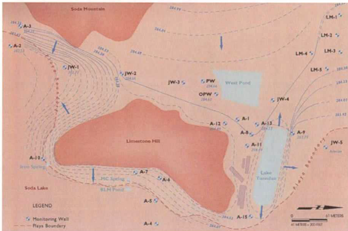
Locations of monitoring wells and interpolated groundwater contours April, 1995 (Dirling, 1997)
