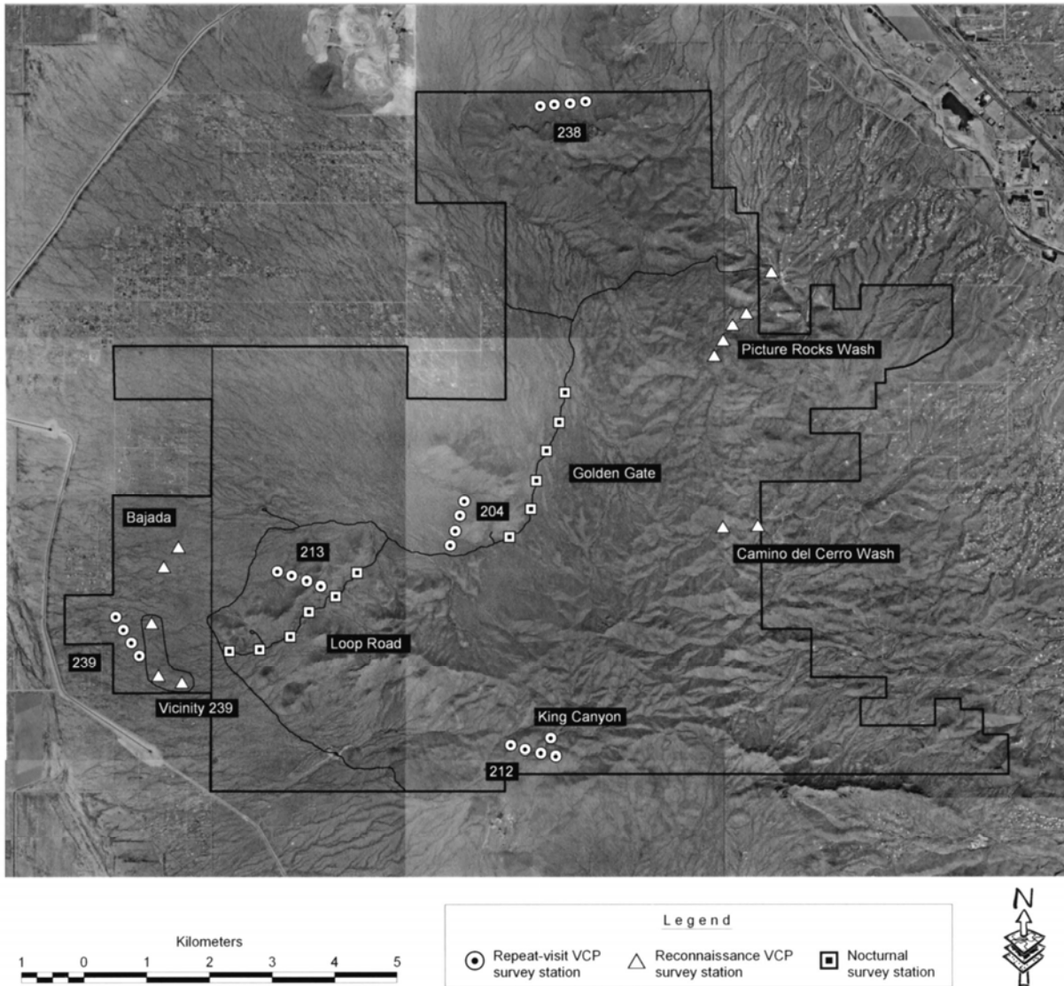
Figure 5.1. Location of VCP and nocturnal survey stations for birds, Saguaro NP, Tucson Mountain District, 2001 and 2002.
