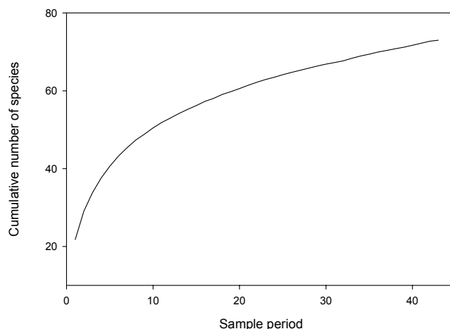
Figure 5.2. Species accumulation curve for birds, all survey methods, Saguaro NP, Tucson Mountain District, 2001 and 2002. Each sample period is a randomized combination of approximately 50 observations ( N = 2,142 ).
