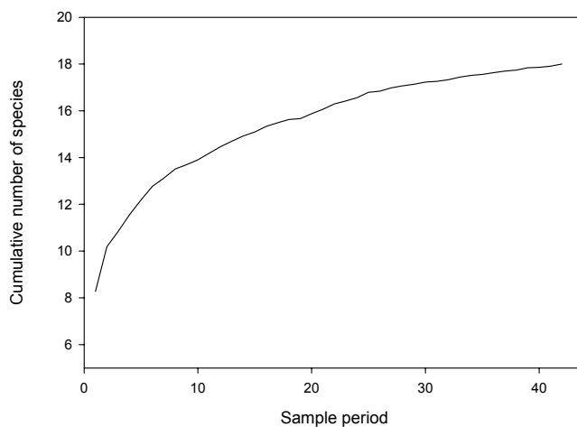
Figure 6.7. Species accumulation curve for infrared-triggered photography, Saguaro NP, Tucson Mountain District, 2002-2005. Each sampling period represents a random ordering of 10 observations.
