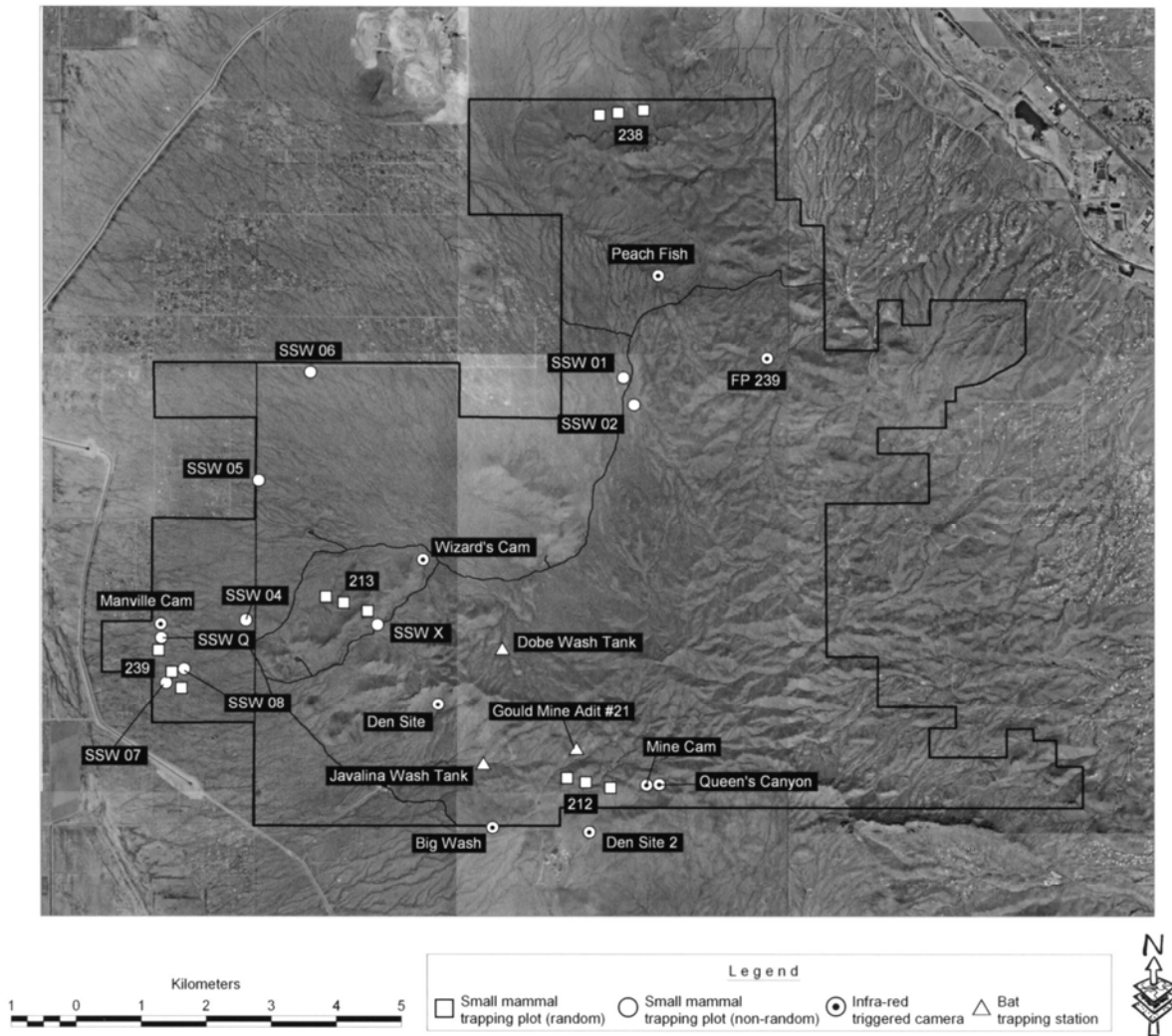
Figure 6.1. Location of random and non-random small-mammal trapping sites, bat trapping stations, and Trailmaster cameras (infrared-triggered cameras), Sagueno NP, Tucson Mountain District, 2001.
