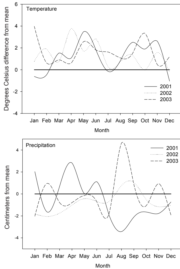
Figure 2.3. Comparison of monthly weather data during the time of the majority of the inventory effort (2001–2003) compared to the mean (1894–2004 for University of Arizona; thick solid line in all figures), Tucson Mountain District, Saguaro National Park. Data from WRCC (2005).
