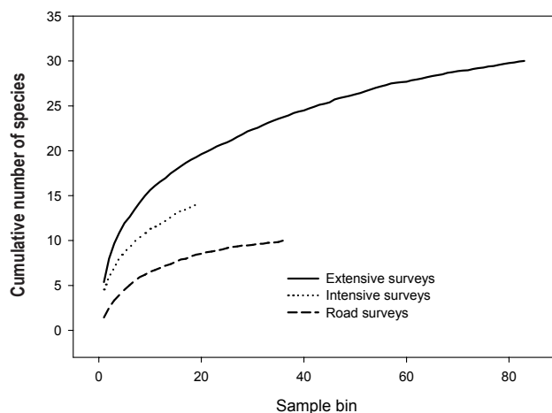
Figure 4.4. Species accumulation curve for herpetofauna surveys, by survey type, Saguaro NP, Tucson Mountain District, 2001 and 2002. Each sampling bin for extensive and intensive surveys represents batches of 11 individuals, and the sampling bin for road transects represents two individuals.
