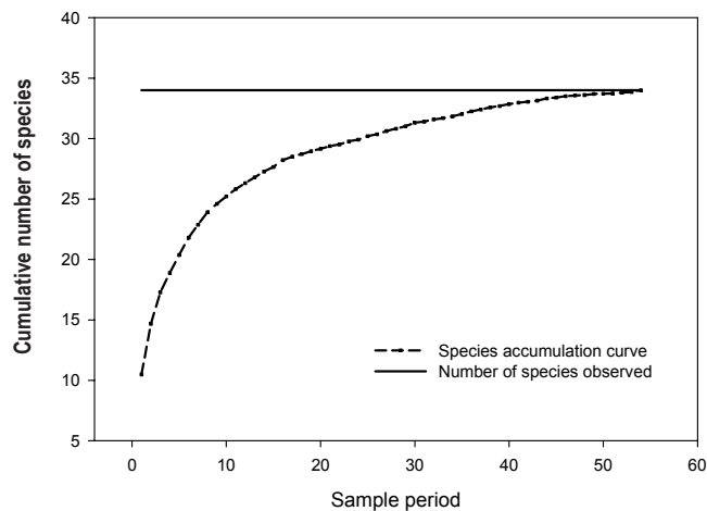
Figure 4.3. Species accumulation curve for herpetofauna surveys, all methods combined, Saguaro NP, Tucson Mountain District, 2001 and 2002. Each sampling period represents batches of 33 individuals, the mean number of individuals observed in an 8-hour field day.
