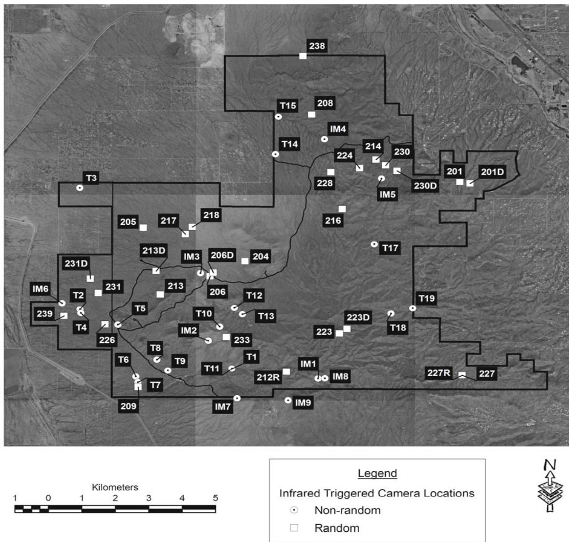
Figure 6.2. Location of infrared-triggered camera units, Saguro NP, 2002-2005. Includes symbols for 2001 and 2002 (from Fig. 6.1), non-random points; 2002-2005, random points, and 2002-2005, non-random points.
