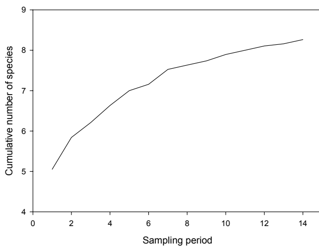
Figure 6.6. Species accumulation curve for small-mammal trapping, Saguaro NP, Tucson Mountain District, 2001. Each sampling period represents a random ordering of 10 observations.
