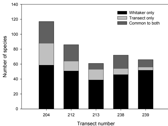
Figure 3.4. Number of plant species at the five random sites that were found by each of the two field methods used at focal points (point-intercept transect and modified-Whitaker plot), Saguaro NP, Tucson Mountain District, 2001.
