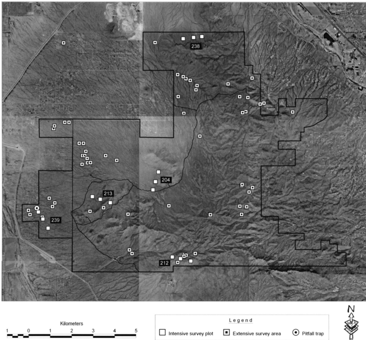
Figure 4.2. Study site locations for herpetofauna, Saguaro NP, Tucson Mountain District, 2001 and 2002.
