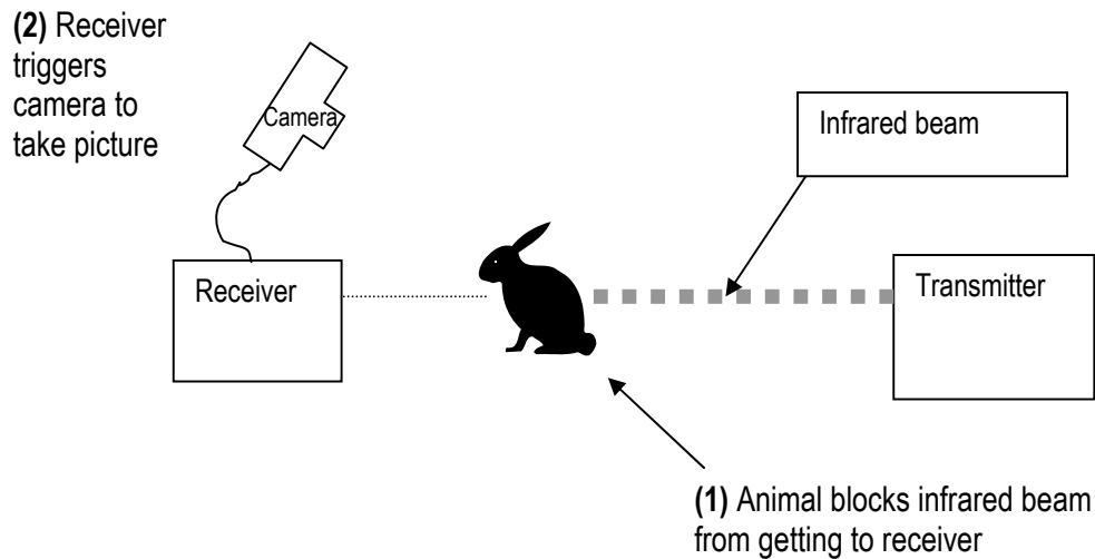
Figure 6.5. Typical configuration for an active infrared-triggered camera system. Image based on Swann et al. (2004).
