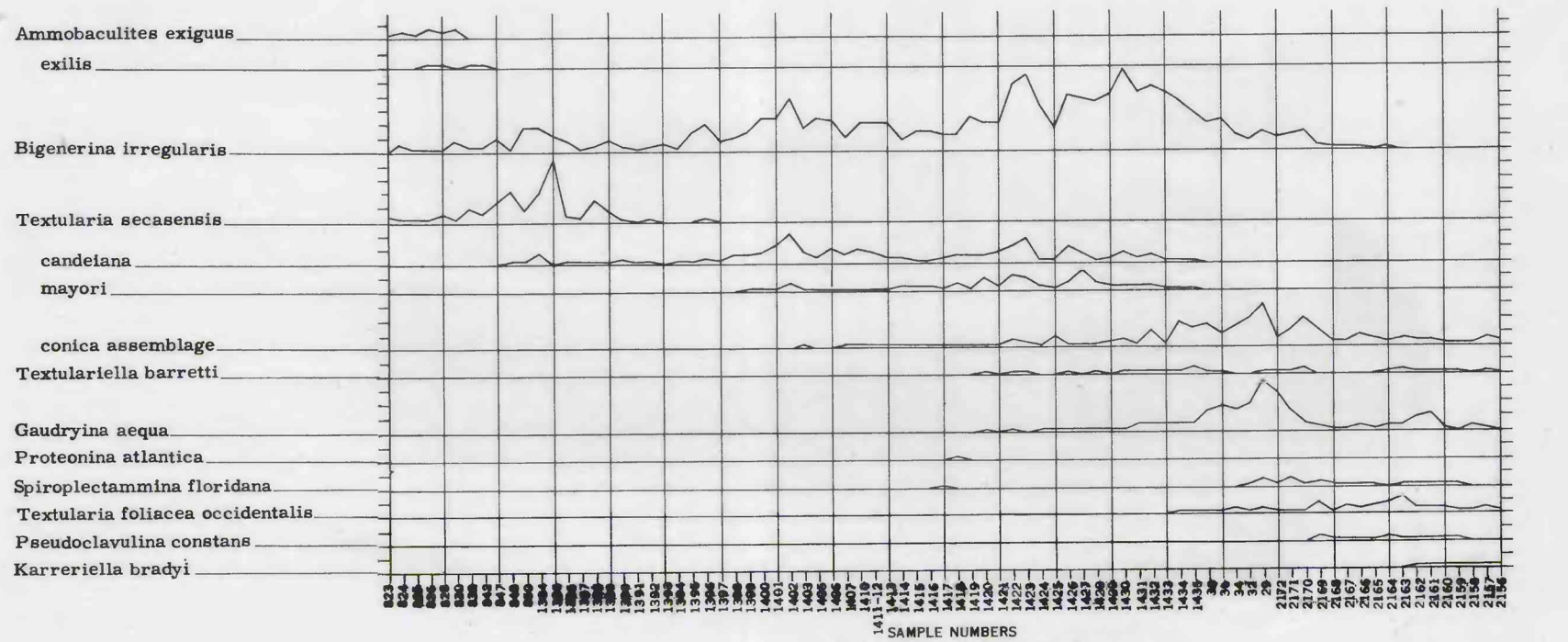
FORAMINIFERAL DISTRIBUTION OFF THE COCOHATCHEE RIVER, FLA.
