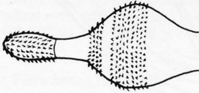
1.6 Andracantha
