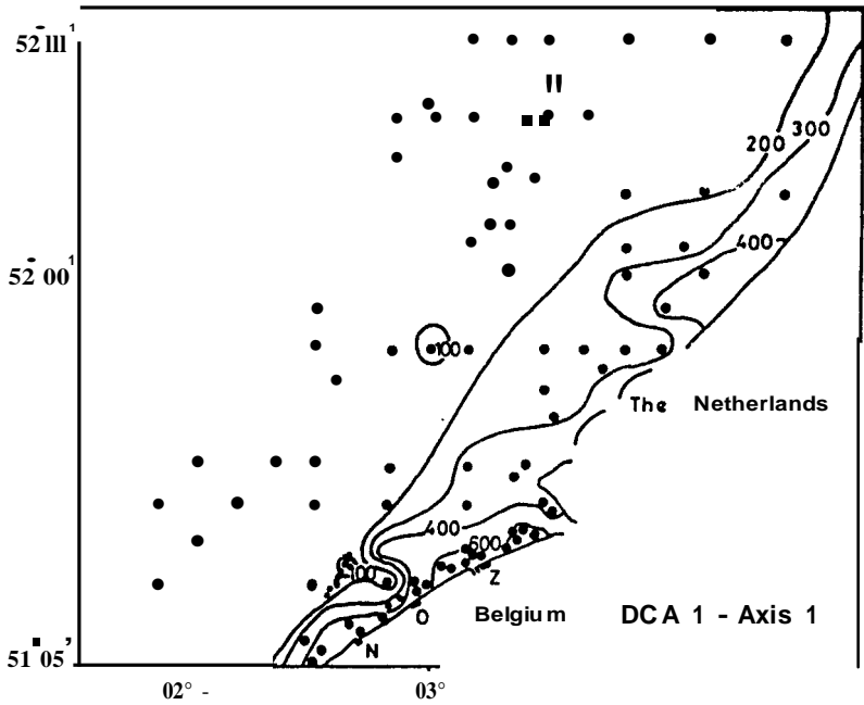
Fig. 9 : Areas demarcated by iso-lines of DCA 1-Axis 1 scores of the Southern Bight.
