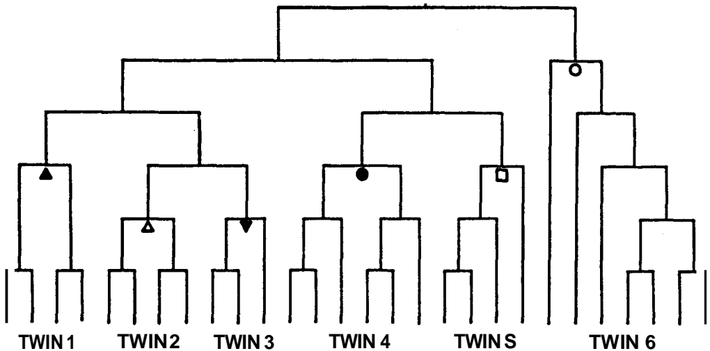
Fig. 6: Dendrogram of the Twinspan classification.
