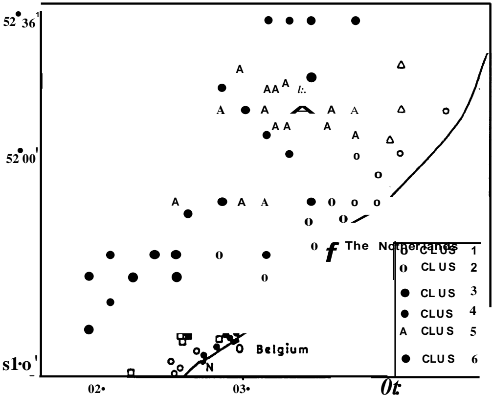
Fig. 5 : Distribution of the six station groups of the cluster analysis in the Southern Bight.
