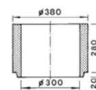
BE300SCH280
