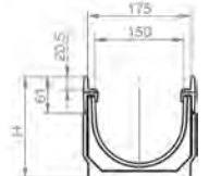
STRONGLINE 150
