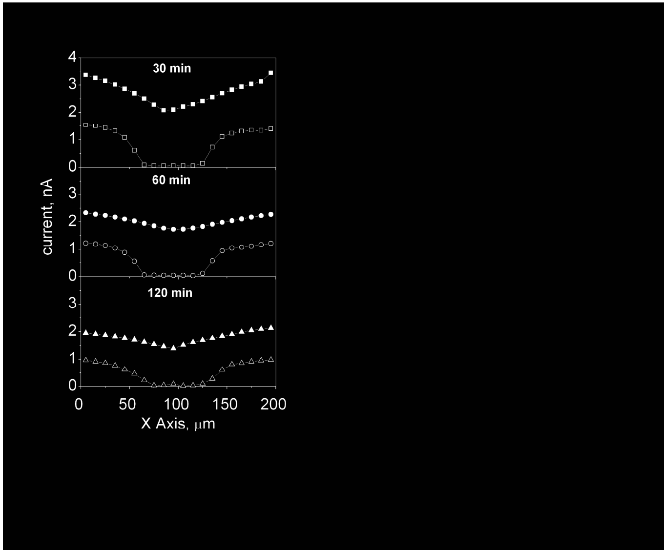
Fig. 7. Plots of line scans performed by SECM at different immersion times (indicated on the figure) in the electrolyte solution on a scratched (scratch width: 20 \mu\text{m} ) epoxy coated (filled symbols) and a microcapsules embodied epoxy coated steel sample (open symbols). The oxygen reduction process is monitored.
