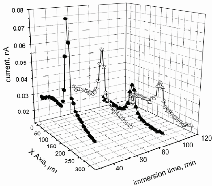
Fig. 4. 3D plot of line scans performed by SECM at different immersion time in the electrolyte solution on an epoxy coated and narrow scratched (20 \mu\text{m} ) steel sample. The \text{Fe}^{2+} oxidation process is monitored. Immersion time: 30 min (●), 60 min (○), 90 min (▲), 120 min (Δ)
