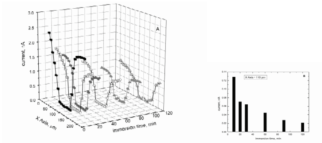
Fig. 5. A: 3D plot of line scans performed by SECM at different immersion time in the electrolyte solution on an epoxy coated and scratched (20 \mu\text{m} ) steel sample. The oxygen reduction process is monitored. Immersion times: 10 min (■), 20 min (□), 30 min (●), 60 min (○), 90 min (▲), 120 min (Δ) B. The time dependence of oxygen reduction current measured in the middle of the scratch
